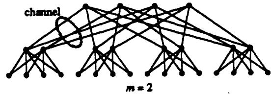
Figure 1: A fat-tree.
