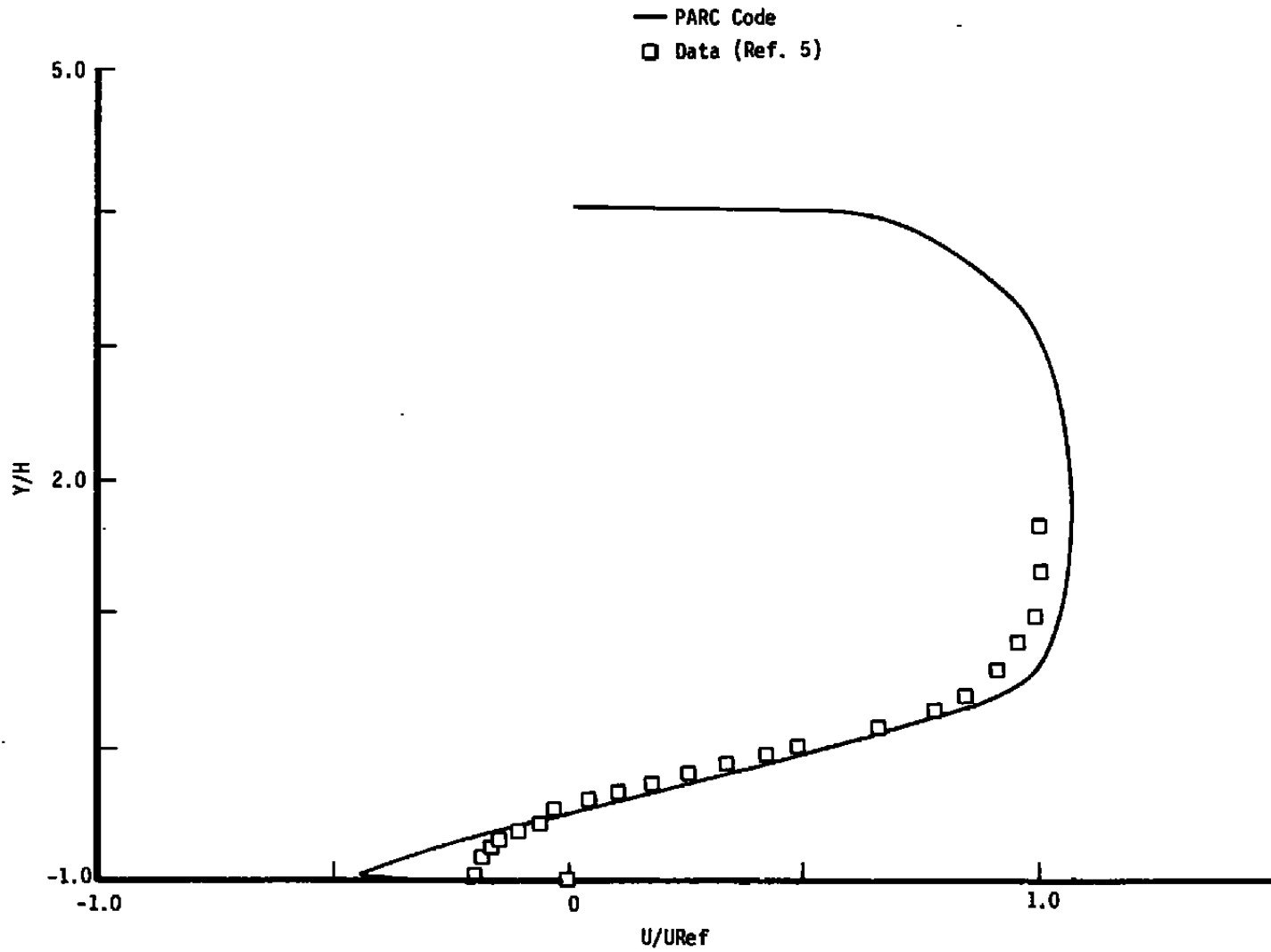
a. X/H = 3.2 ( X/H = 0 at step) Figure 26. Velocity profile comparisons for backstep flow.
