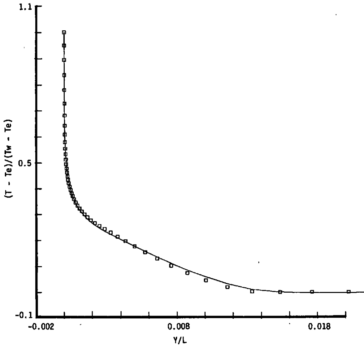
b. Temperature profile (edge scaling) Figure 10. Continued.
