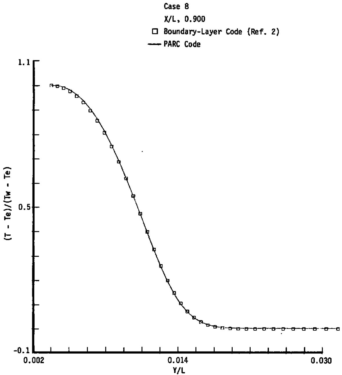
b. Temperature profile Figure 6. Continued.
