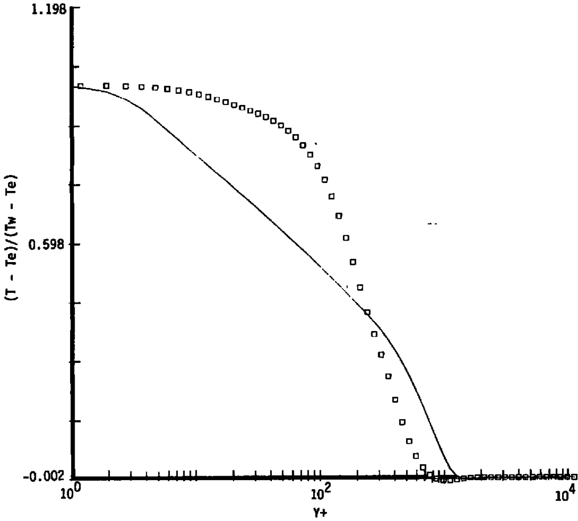
d. Temperature profiles (old versus new; wall scaling) Figure 14. Concluded.
