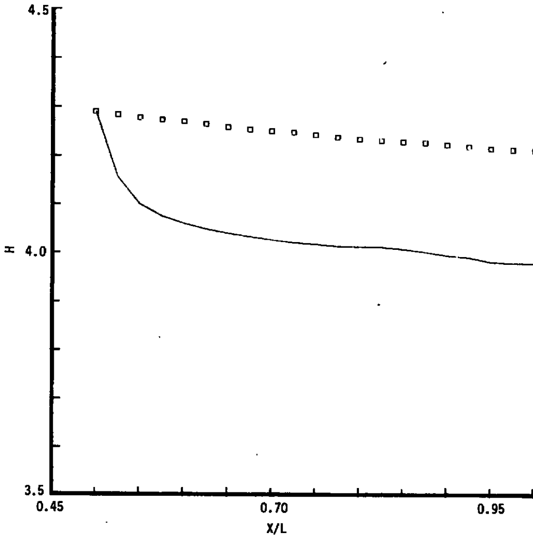
c. Shape factor streamwise variation Figure 13. Continued.
