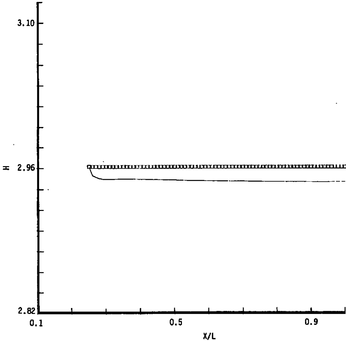
c. Shape factor streamwise variation Figure 2. Continued.
