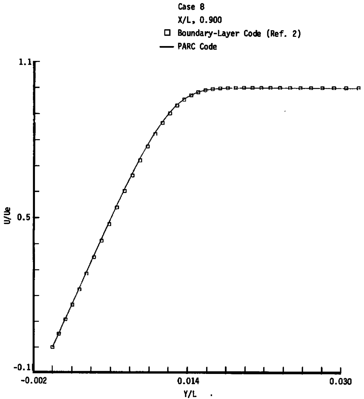
a. Velocity profile Figure 6. Supersonic laminar flat-plate flow comparisons.
