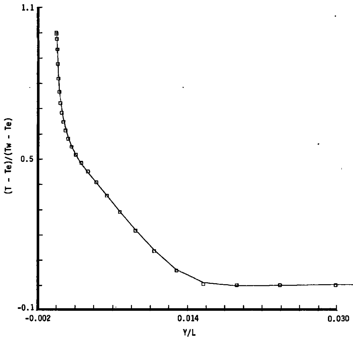
b. Temperature profile (edge scaling) Figure 13. Continued.
