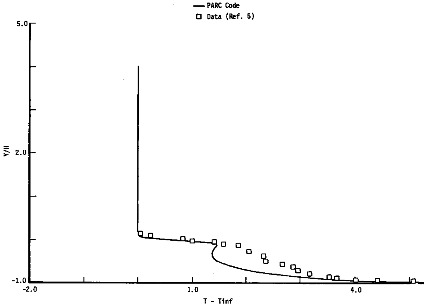
a. X/H = 0.33 (X/H = 0 at step) Figure 27. Temperature profile comparisons for backstep flow.
