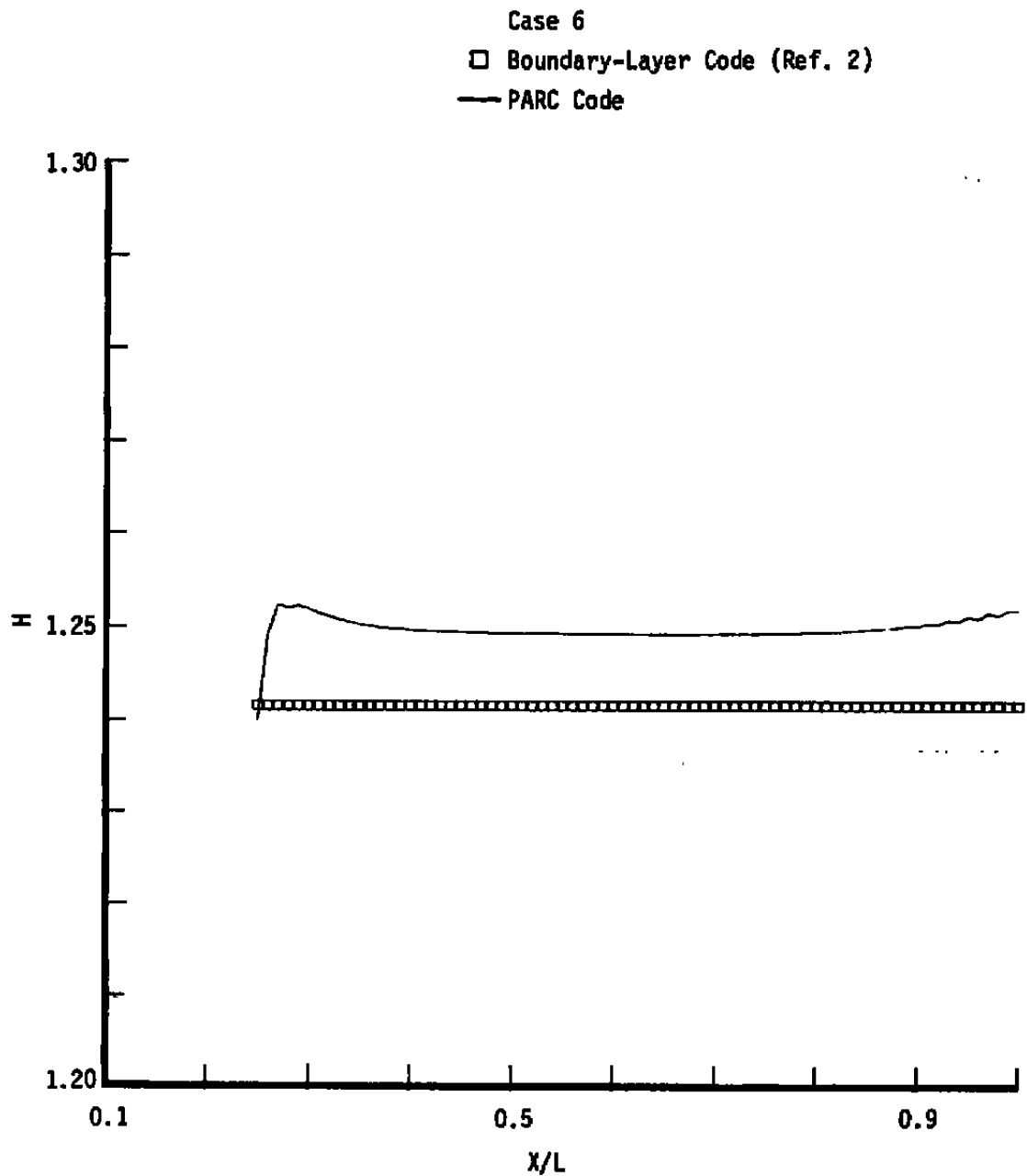
c. Shape factor streamwise variation Figure 4. Continued.
