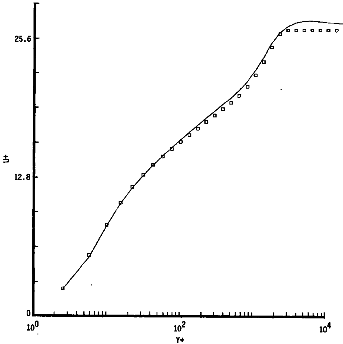
e. Velocity profile (wall scaling) Figure 12. Continued.
