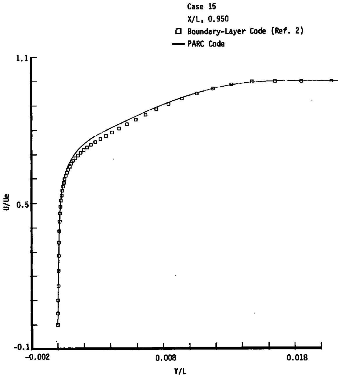
a. Velocity profile (edge scaling) Figure 11. Hot-wall comparisons for turbulent flat-plate flow.
