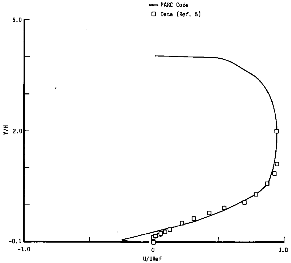
b. X/H = 5.87 Figure 26. Continued.
