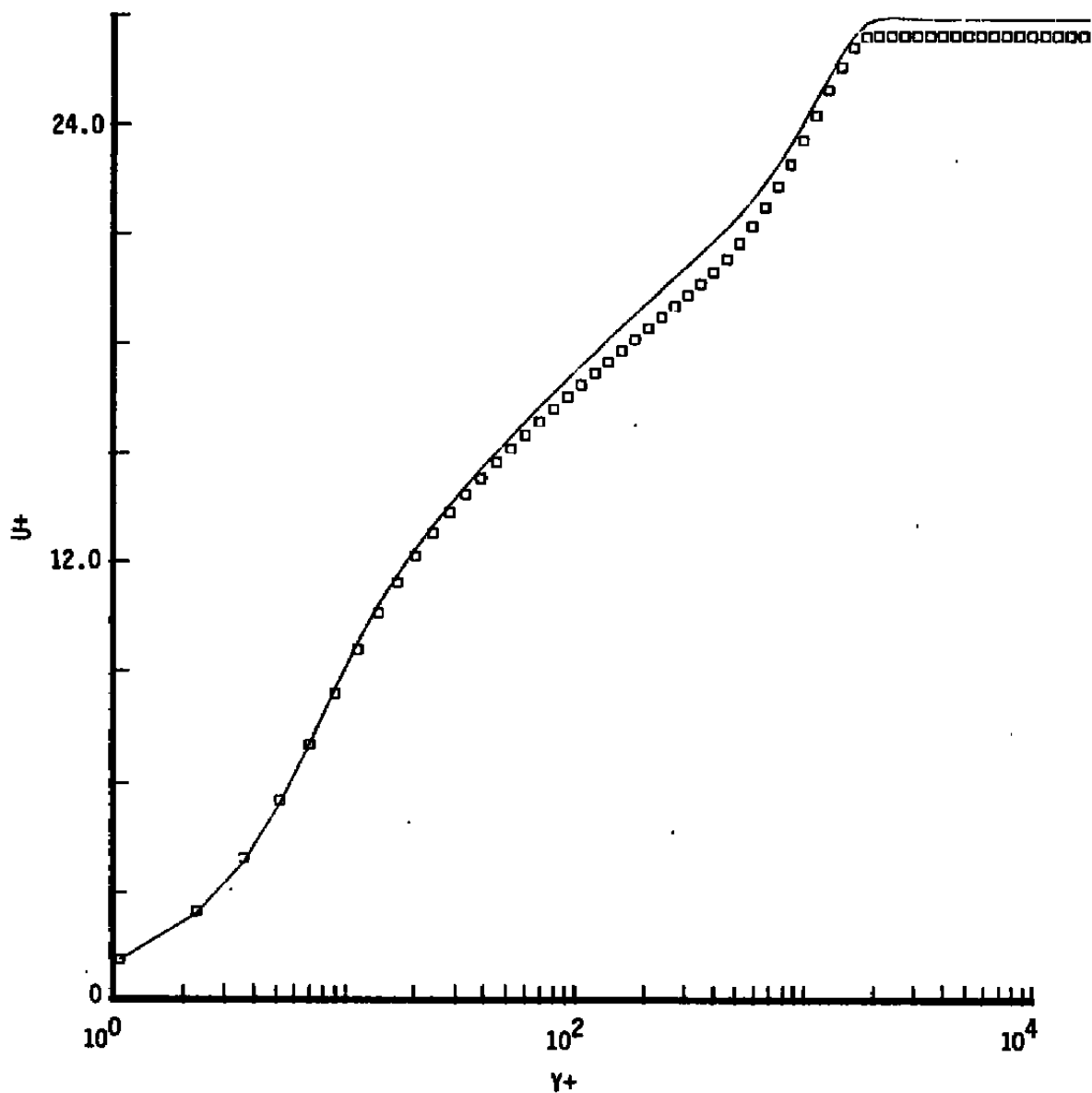
e. Velocity profile (wall scaling) Figure 8. Concluded.
