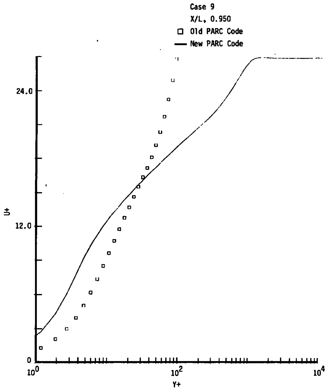
c. Velocity profiles (old versus new; wall scaling) Figure 14. Continued.
