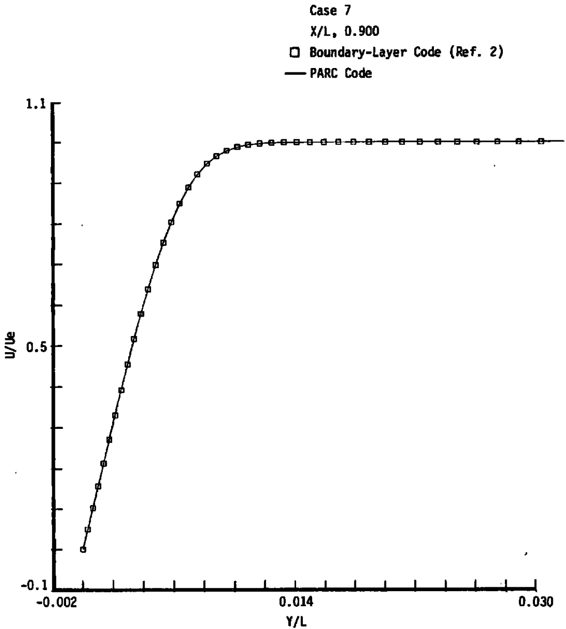
a. Velocity profile Figure 5. Subsonic laminar flat-plate flow comparisons.
