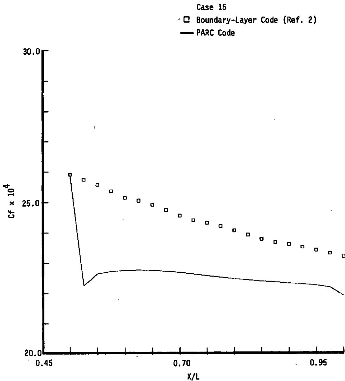
d. Skin friction streamwise variation Figure 11. Continued.
