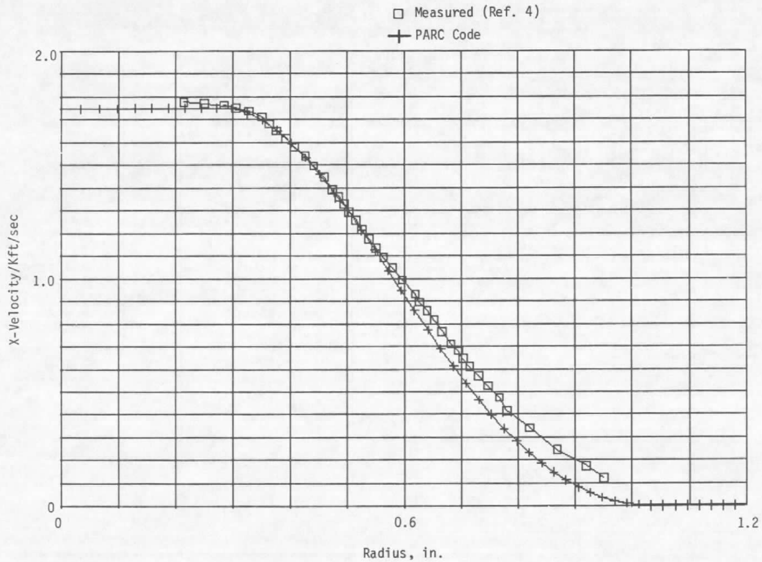
d. X/R_{ne} = 11.0 Figure 18. Continued.
