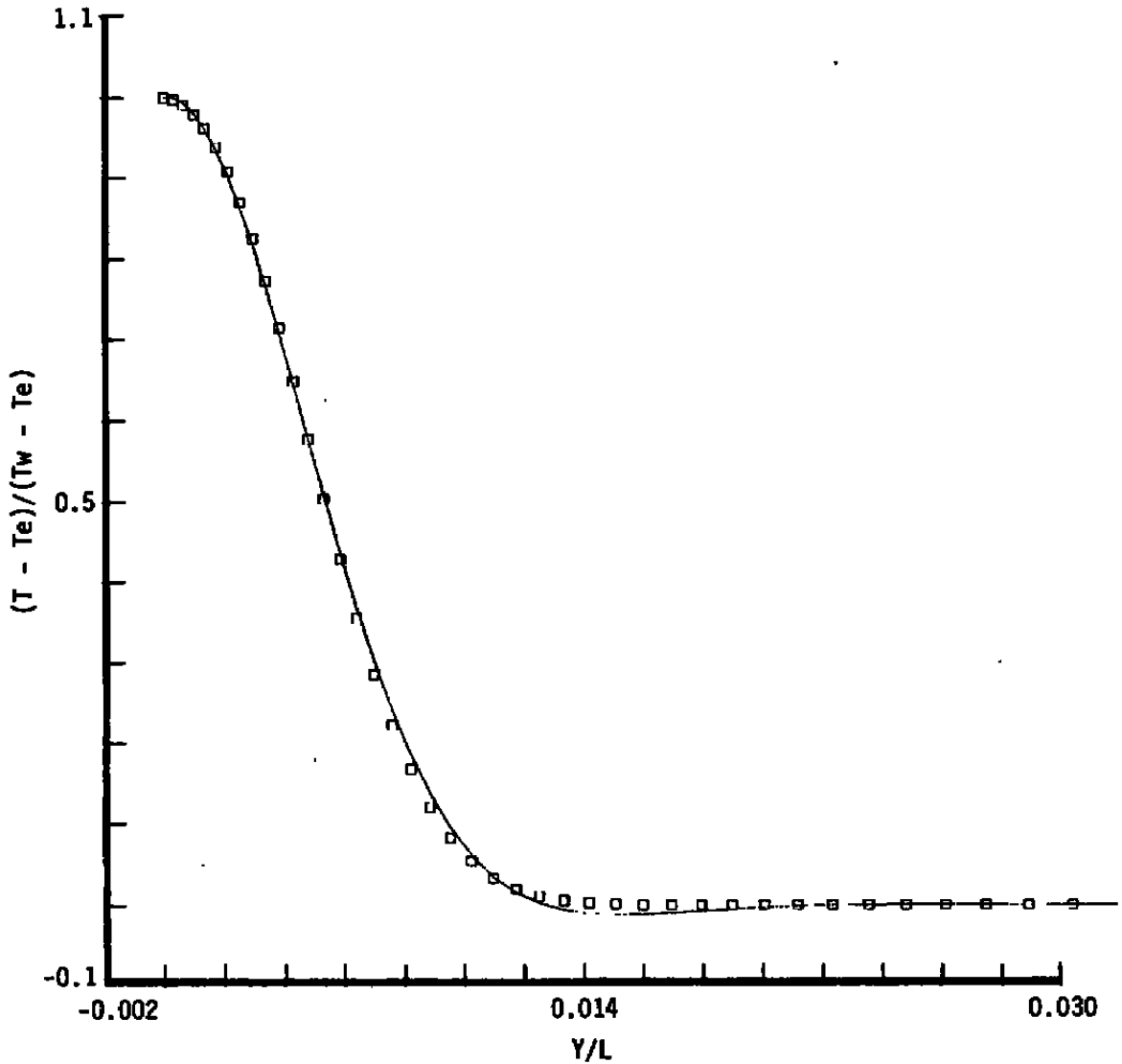
c. Temperature profile (old model, Case 7) Figure 7. Continued.
