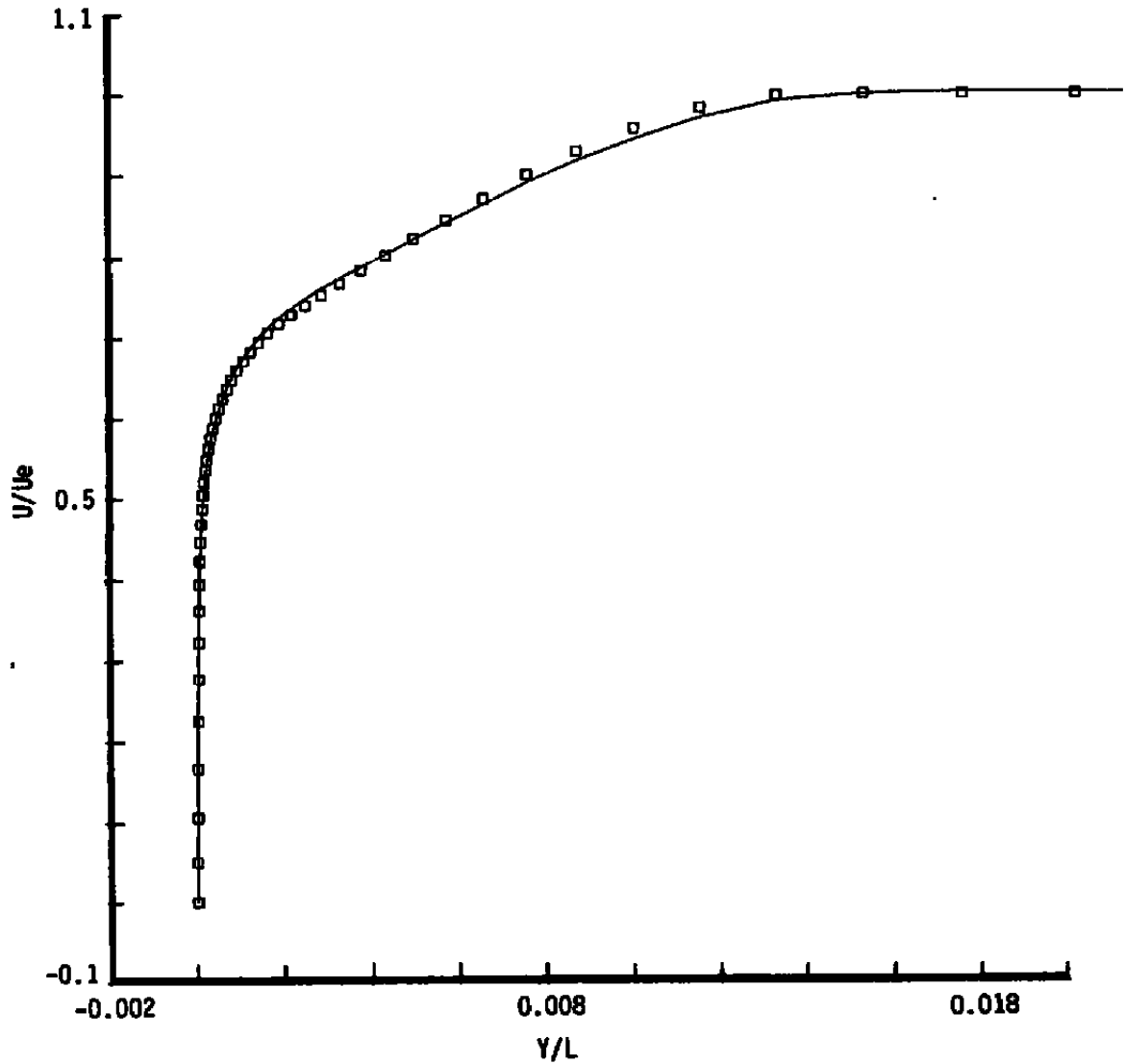
a. Velocity profile (edge scaling) Figure 10. Cold-Wall comparisons for turbulent flat-plate flow.
