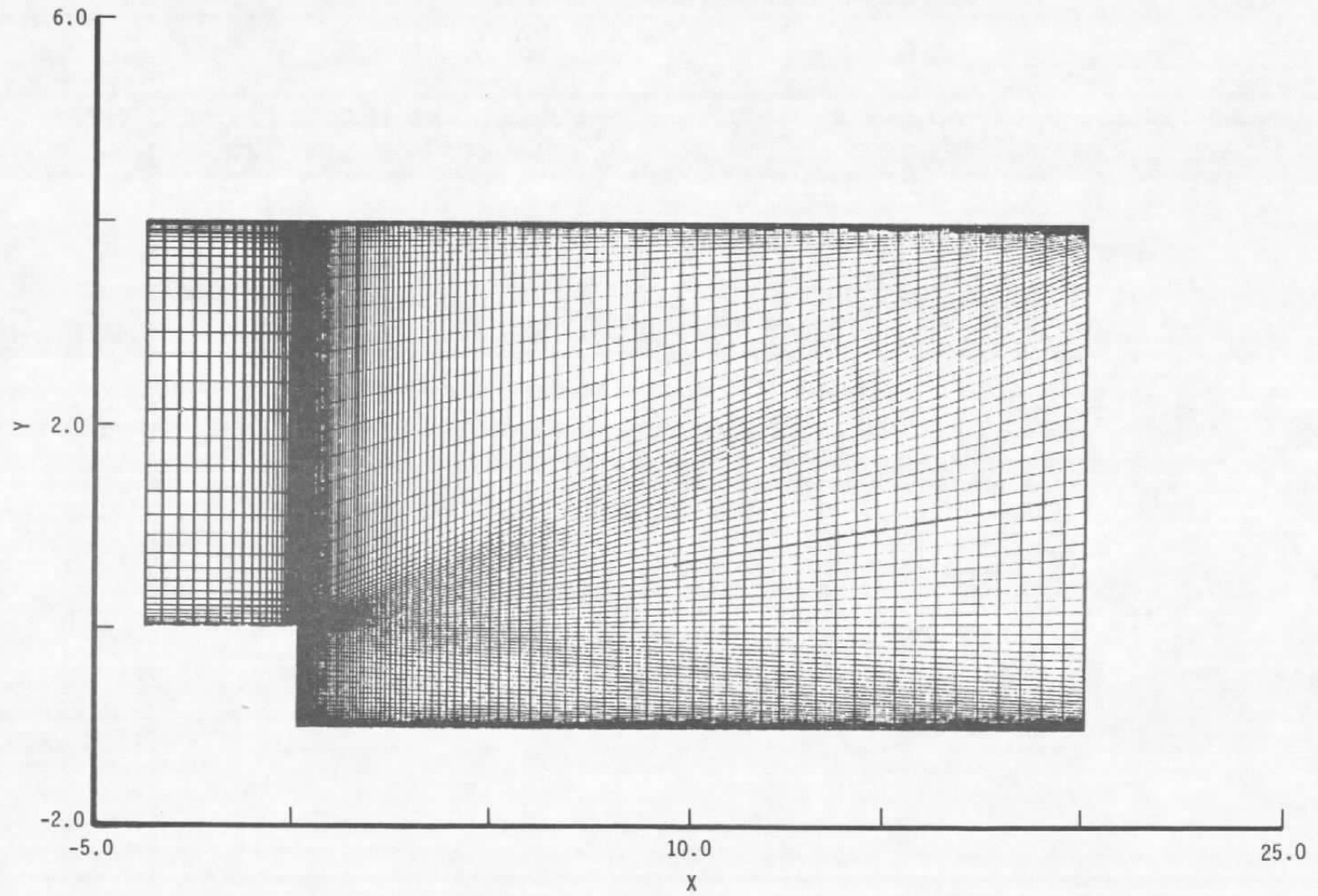
Figure 25. Grid for backstep flow simulation.
