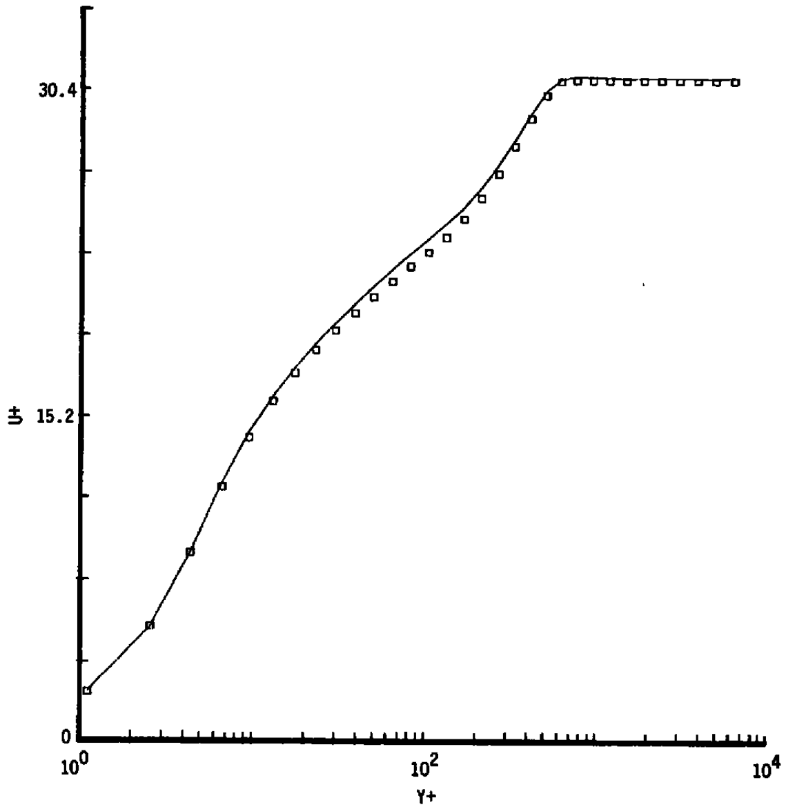
e. Velocity profile (wall scaling) Figure 13. Continued.
