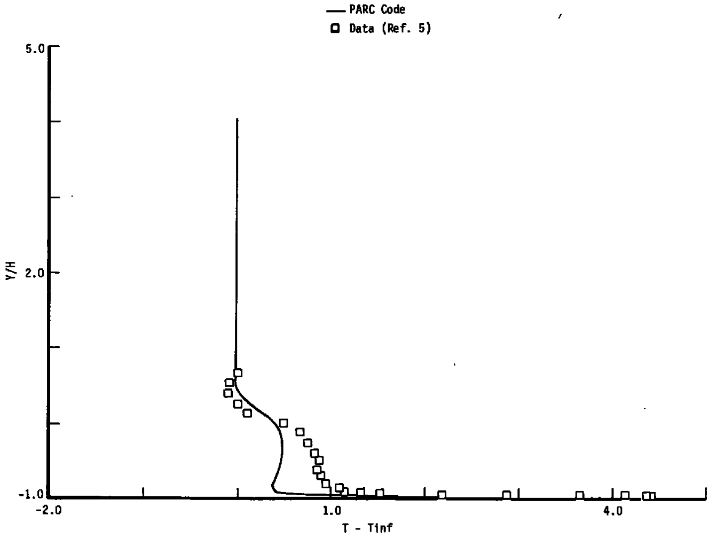
b. X/H = 3.0 Figure 27. Continued.
