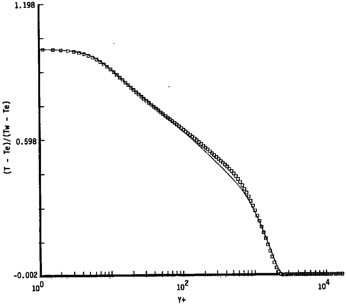
c. Dense grid temperature profile (wall scaling, Case 12) Figure 9. Concluded.
