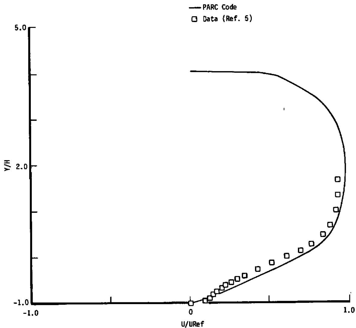
c. X/H = 7.2 Figure 26. Continued.
