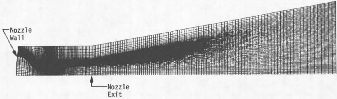
Figure 16. Near-wake grid for supersonic free jet.
