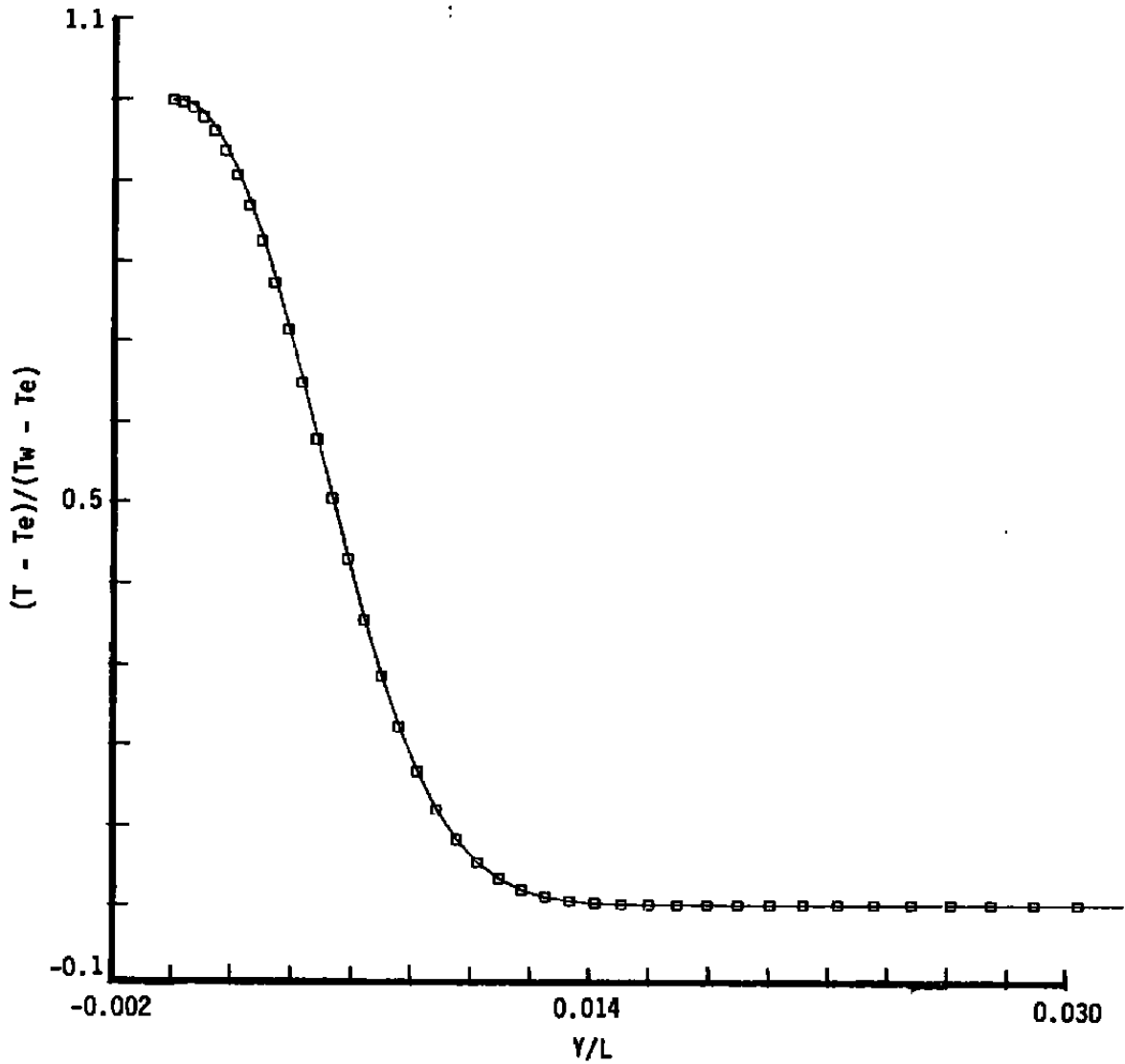
b. Temperature profile Figure 5. Continued.
