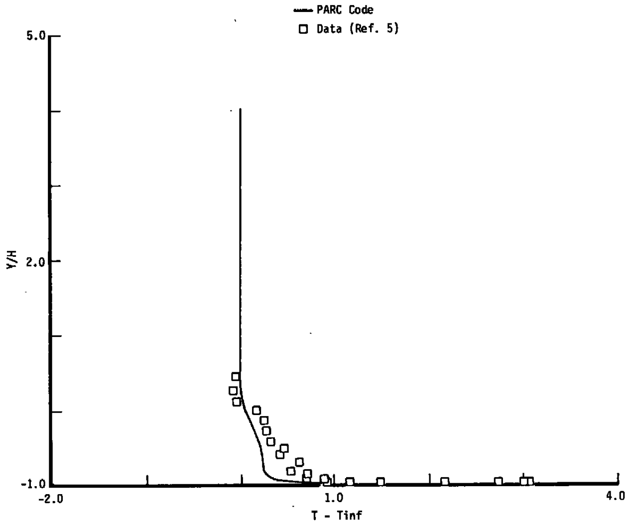
c. X/H = 7.0 Figure 27. Continued.
