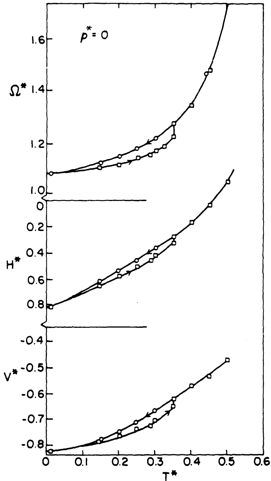
Fig. 2 - Temperature dependent changes in the Volume per atom \Omega^* , enthalpy per atom H^* , and potential energy per atom V^* , all in normalized units for the one-component material under an external pressure of p^* = 0 .
