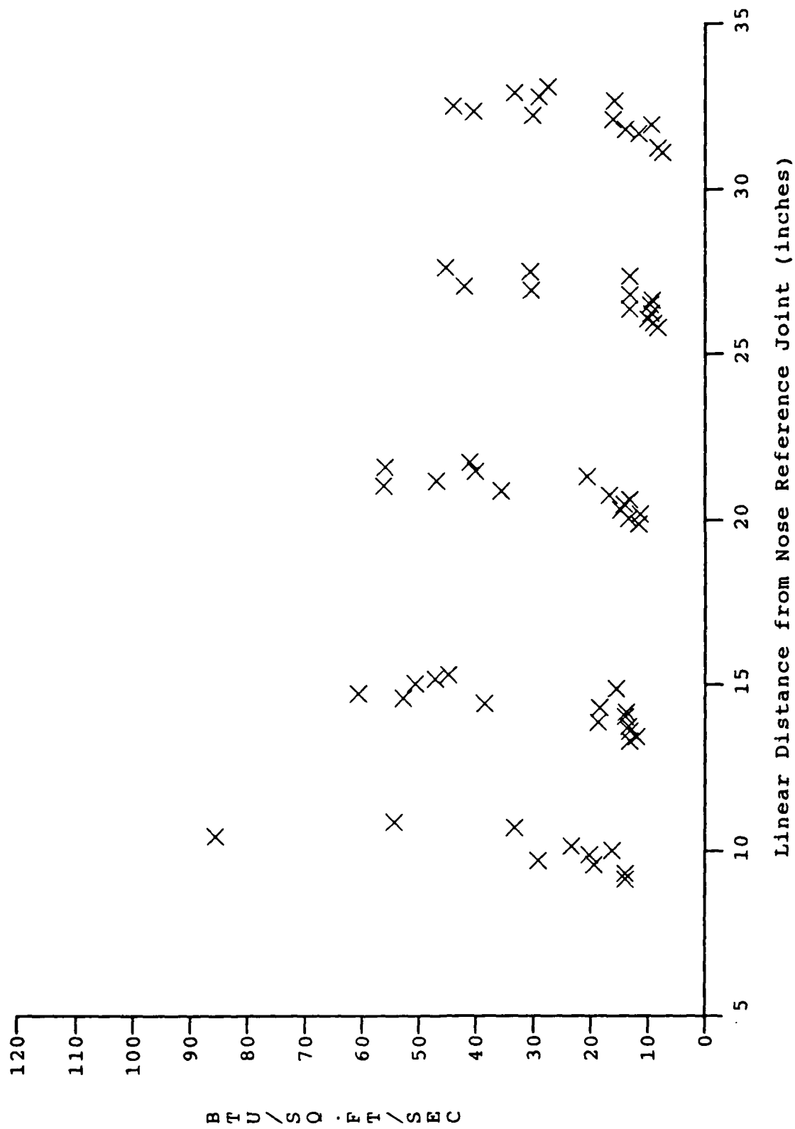
Figure 57c. Distribution of Heating Along Model Surface [ Run# 4, B'=-0.639, M=13, Re/ft=5.0X10 6 ]
