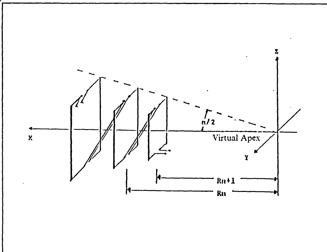
Figure 4. Quad Log-Periodic Antenna with Improved Feed (Staggered Feed)
