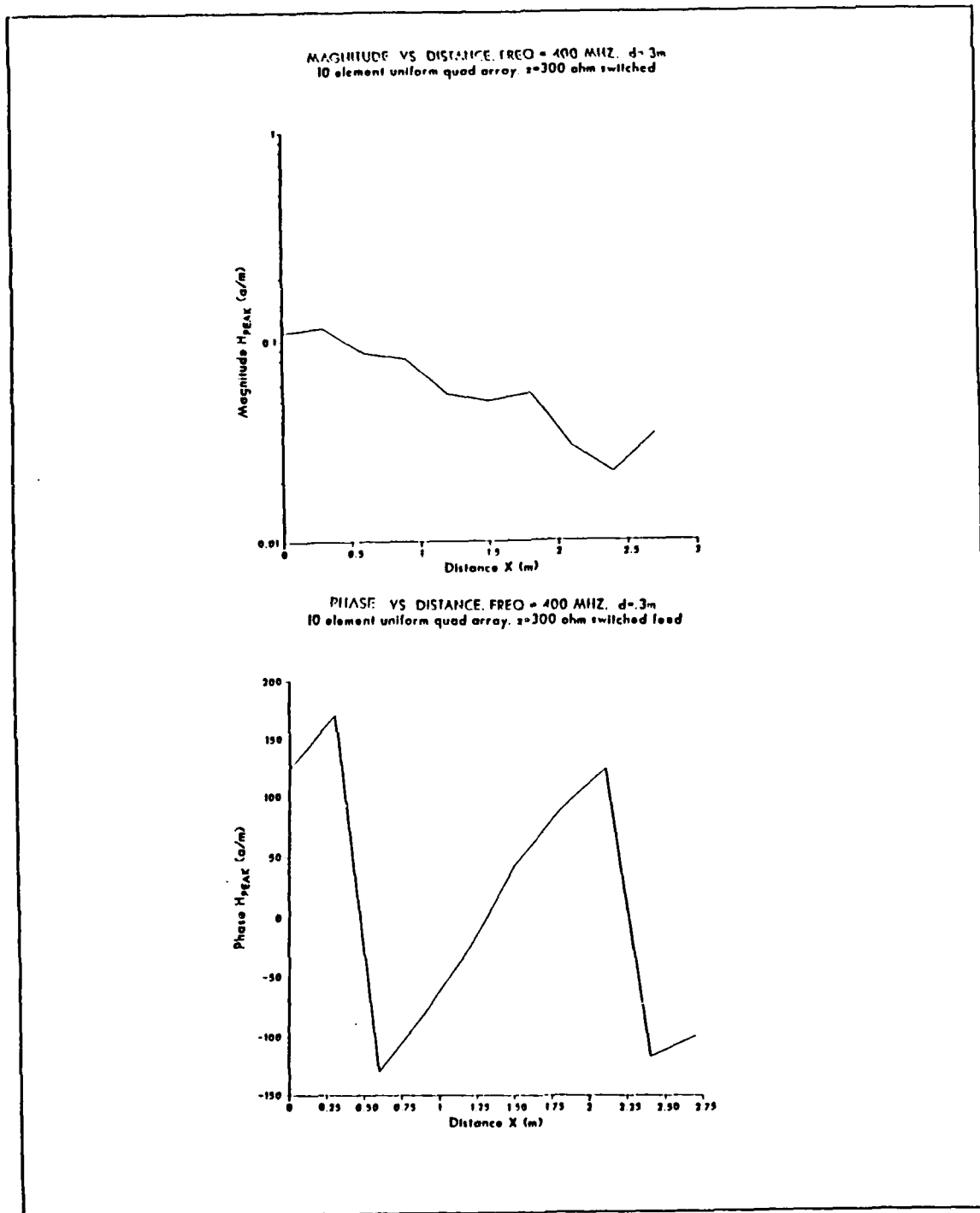
Figure 10. Current Amplitude and Phase in the Backward Radiation Region of a Quad Array
