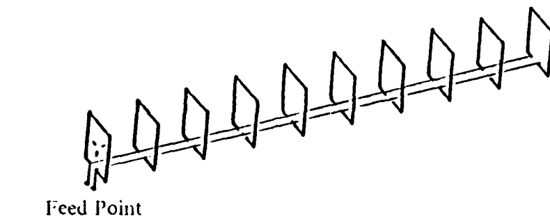
(a) Unswitched Transmission Line
