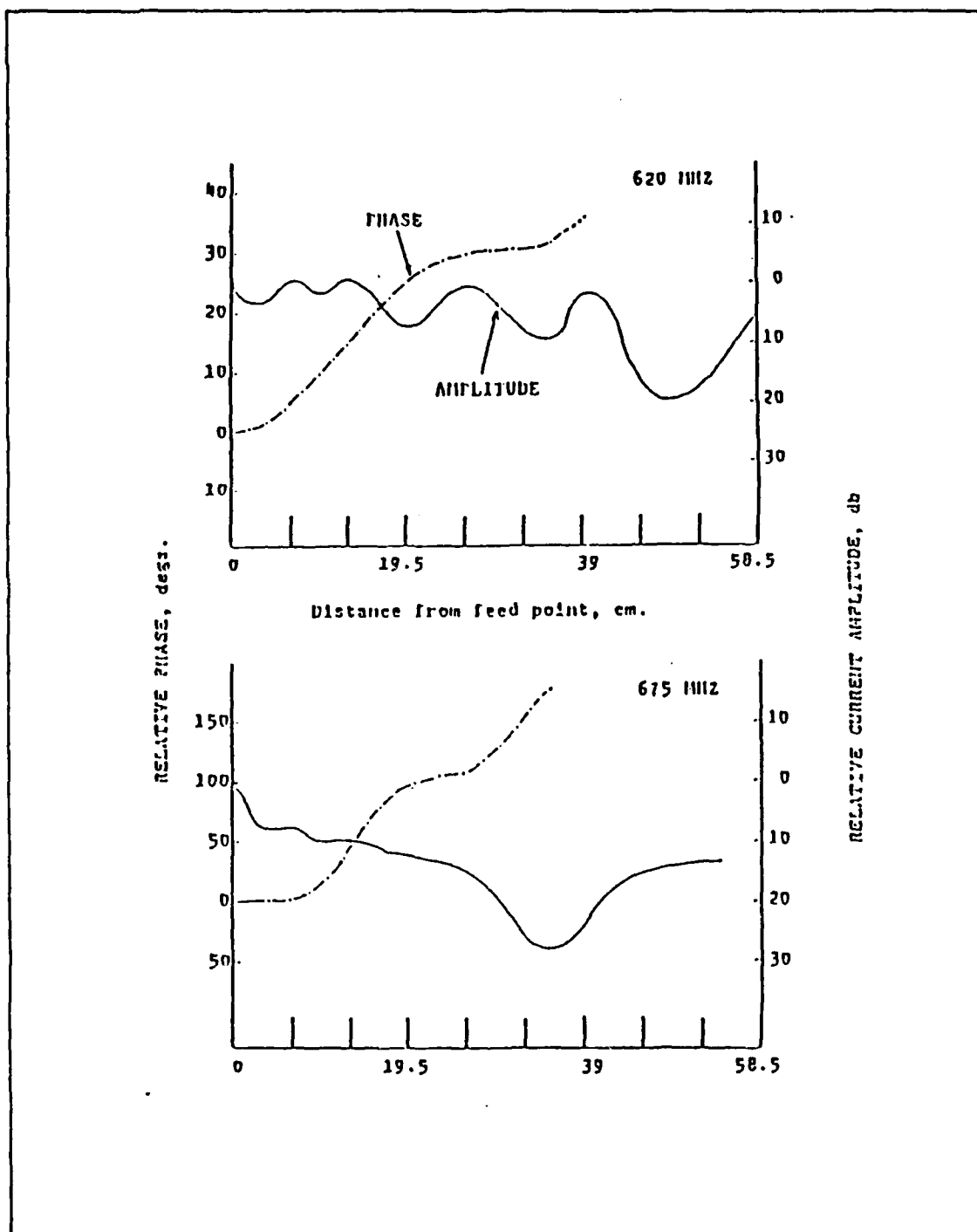
Figure 9. Current Amplitude and Phase in the Backward Radiation Region of a Loop Array [Ref. 10]
