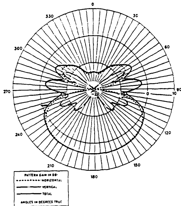
14 ELEMENT QUAD LOG-PERIODIC ARRAY ( FREQ = 560 MHZ ) TAU=.915, SIGMA=.125, (DUPA=.25M) , Z=300 OHM SWITCHED FEED
