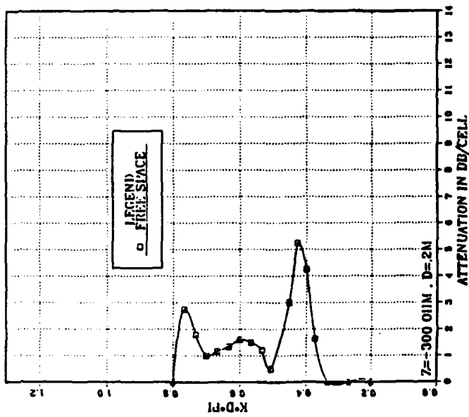
ATTENUATION DIAGRAM
