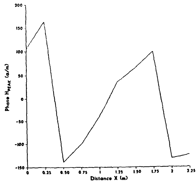
PHASE VS DISTANCE. FREQ = 450 MHz. d=25m 10 element uniform quad array. z=300 ohm switched feed
