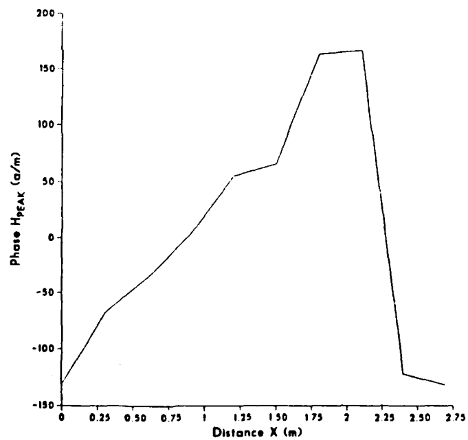
PHASE VS DISTANCE. FREQ = 300 MHZ. d=3m 10 element uniform quad array. z=300 ohm switched feed
