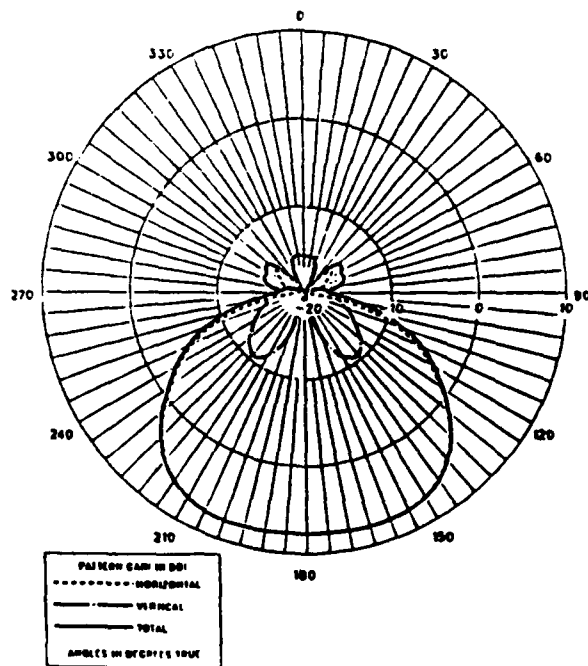
10 ELEMENT UNIFORM QUAD ARRAY ( FREQ = 350 MHZ ) HORIZONTAL PATTERN. D=.25M , Z=300 OHM SWITCHED FEED
