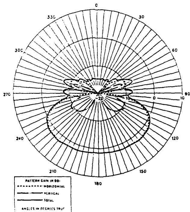
14 ELEMENT QUAD LOG-PERIODIC ARRAY ( FREQ = 560 MHZ ) TAU=.915, SIGMA=.125, (DUPA=.25M) , Z=300 OHM SWITCHED FEED
