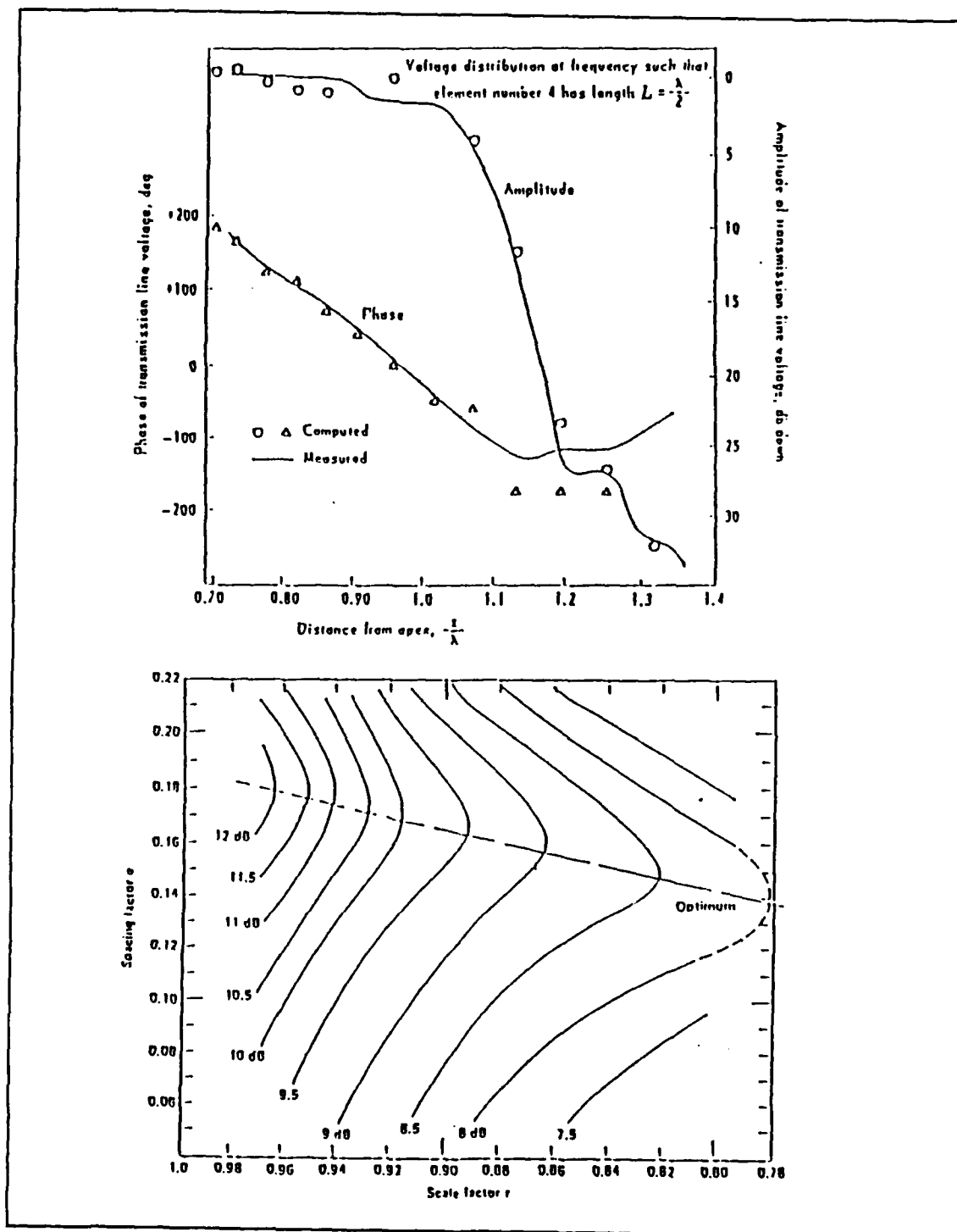
Figure 7. Carrel's Curves and Experimental Values [Ref. 3]
