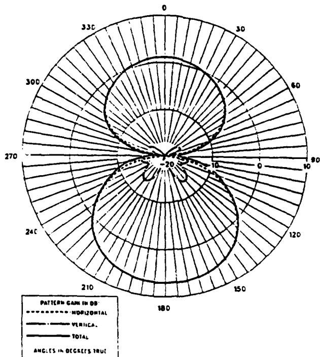
14 ELEMENT QUAD LOG-PERIODIC ARRAY ( FREQ = 230 MHZ ) TAU=.915, SIGMA=.125, (DUPA=.25M), Z=300 OHM SWITCHED FEED
