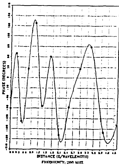
CURRENT PHASE
