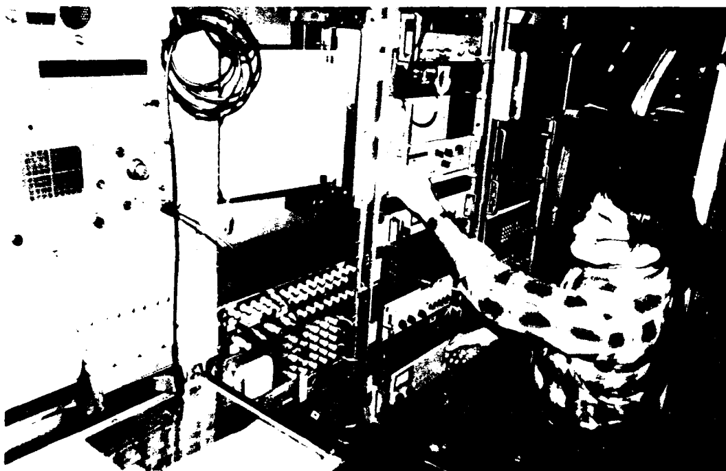
Figure 10. The chirp receiver is checked out. Please. The unit checks out the Chirp Sounder Receiver on the ship's deck. The receiver is mounted on a rack of equipment in the support of the Over the Horizon Backscatter
