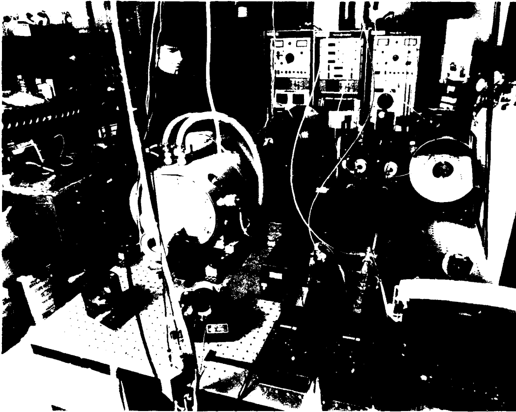
High-Power Electron Beam Injection CO 2 TEA Laser Under Development at AFGL. (This laser will act as the transmitter in a coherent, Doppler wind-sensing system to provide meter-per-second wind velocities out to a range of 30 km. Such a lidar system has application to design criteria for electro-optical systems performance, to the detection of wind shear and low-level turbulence, and to the determination of local wind patterns over complex terrain.)
