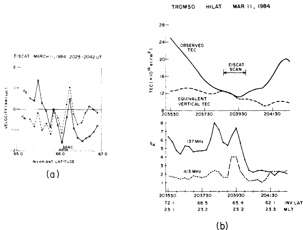
Coordinated EISCAT/HILAT Measurements Showing Presence of Intense VHF/UHF Scintillations in the Absence of "Blobs," or TEC Structure, but in Association with Velocity Shears in the F-region.
