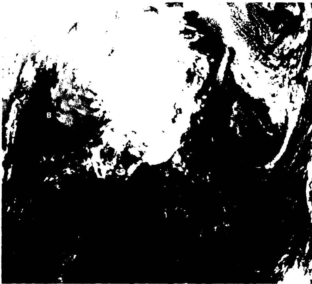
NOAA-7 AVHRR 3.7 \mu\text{m} Imagery for June 11, 1982, at 0800 GMT over South Carolina. (Note how well the fog (feature A) contrasts with the adjacent cloudfree land (feature B); 3.7 \mu\text{m} imagery is useful for the detection of nighttime fog and low clouds. Contrasts are poor between low clouds and cloudfree land or oceans in longer-wavelength 10-12 \mu\text{m} imagery, making it difficult to use for detection of low clouds and fogs at night. Next generation DMSP meteorological sensors will be providing imagery at 3.7 \mu\text{m} .)
