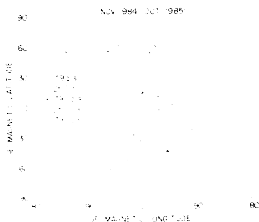
Figure 1. Contours of Constant Dose Rate for the Electrons >2.5 MeV Lolet Channel. Plotted in Corrected Geomagnetic Latitude and Longitude Coordinates.
