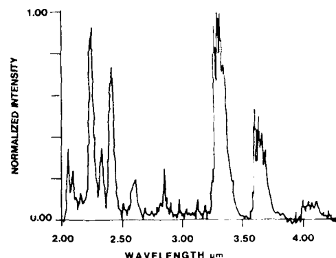
Short Wavelength Infrared Emission Spectrum Observed from Discharged Ar/N 2 with Ar Counterflow under Conditions of High N 2 Flow. (Resolution is 0.013 μm. The flow conditions were 2500 μmole per second Ar and 250 μmole per second N 2 through the discharge and 2700 μmole per second Ar through the counterflow.)
