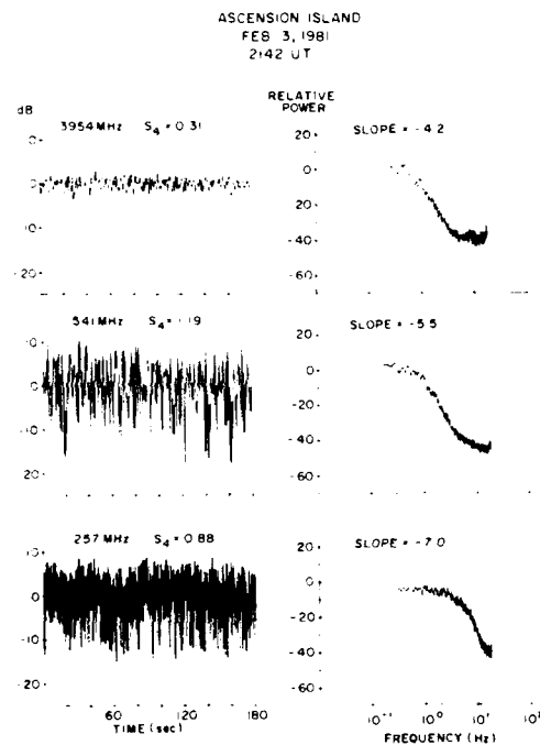
Three-minute Data Segment of Scintillations Observed at 3954, 1541, and 257 MHz at Ascension Island and Their Respective Spectra.
