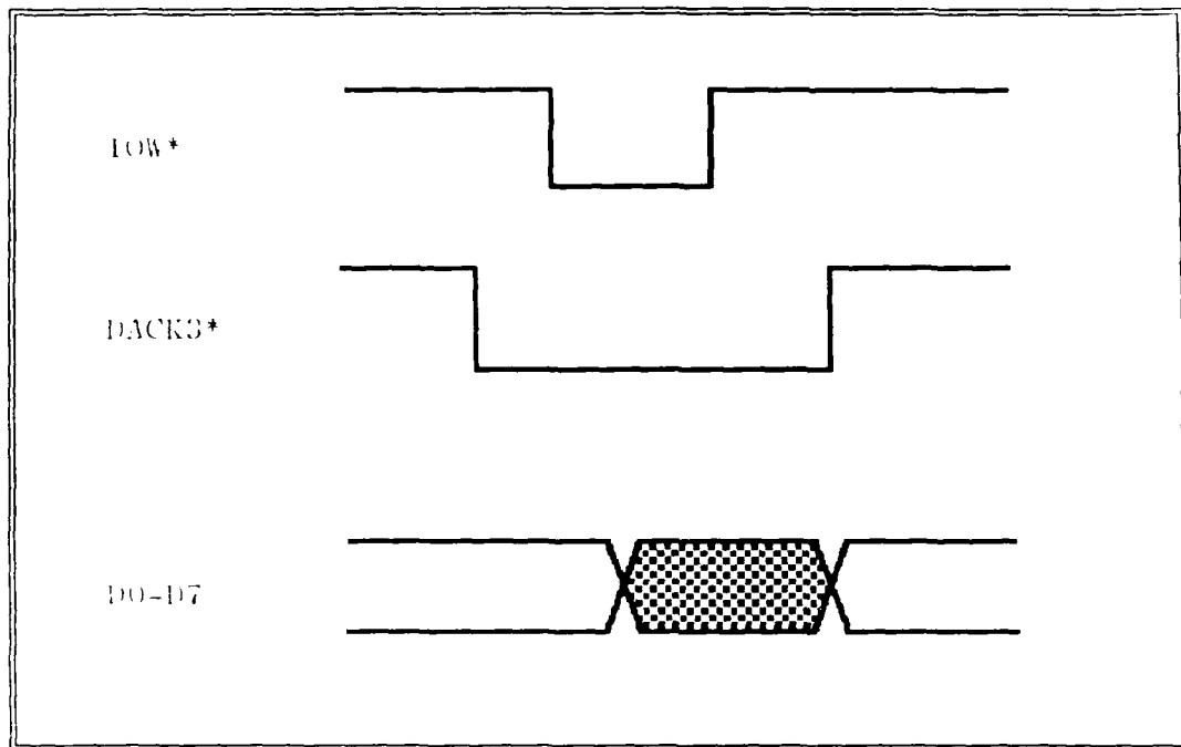
Figure 7. DMA Initiated Read From Memory
