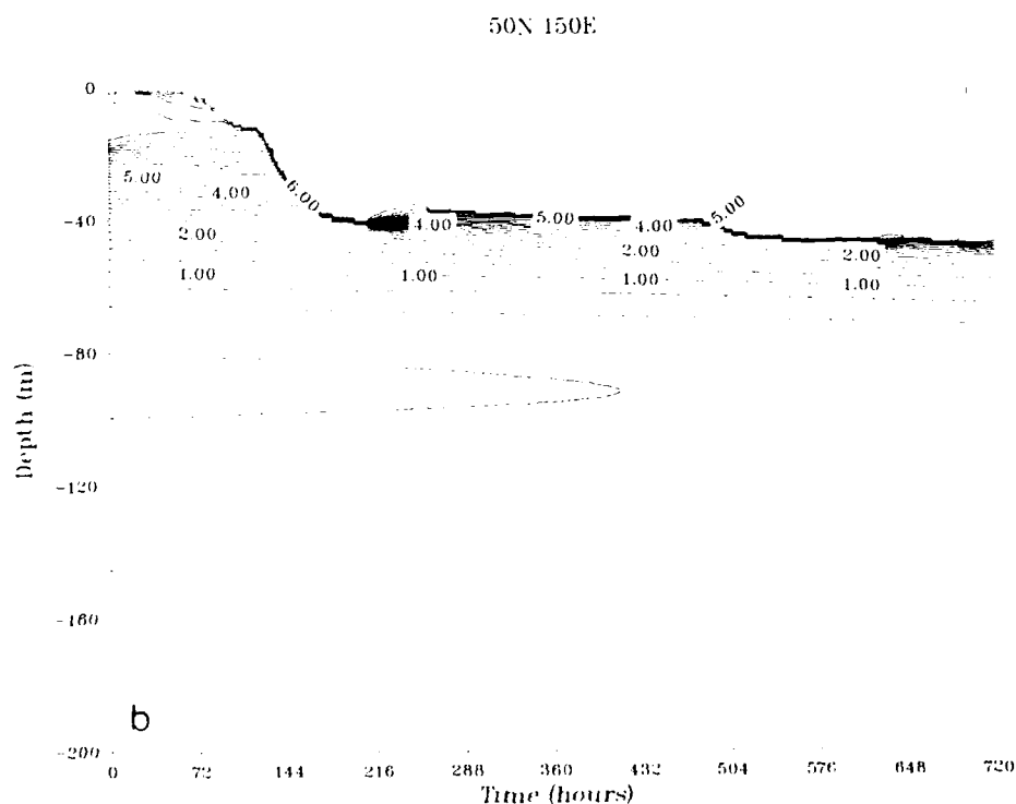
Fig. 5. Temperature (m degrees Celsius) as a function of time (0-30 days) and depth (0-200 m) at 50 N, 150 E in the (a) control and (b) nuclear winter experiments.
