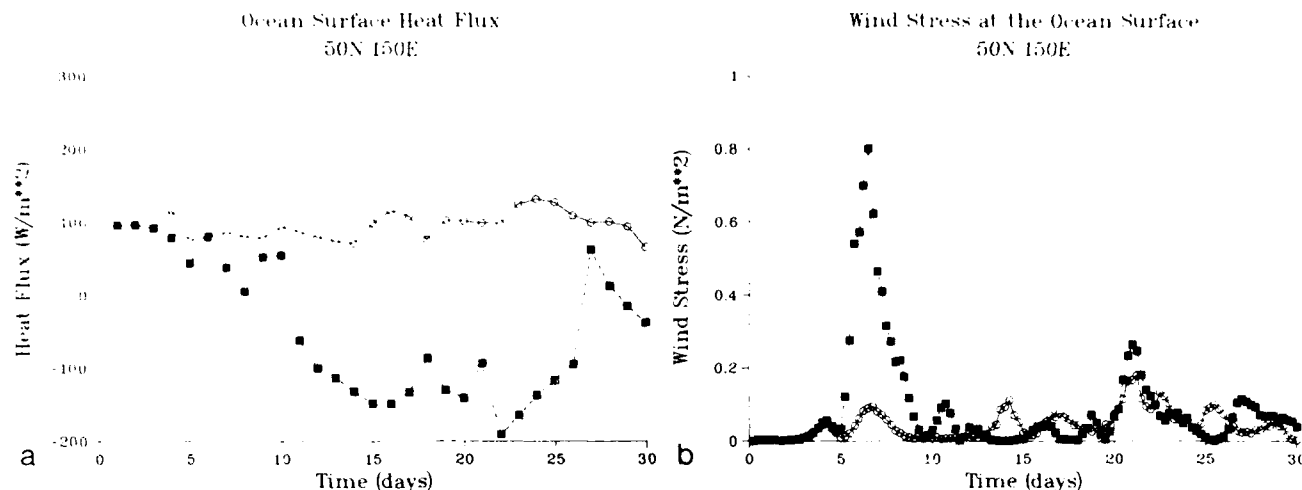
Fig. 4. Time evolution of the calibrated (a) net surface heat flux Q_n and (b) surface wind stress \tau at 50 N, 150 E used in the control experiment (solid lines) and the nuclear winter experiment (dashed).
