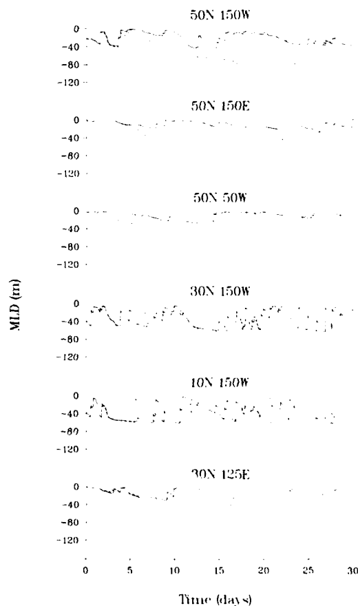
Fig. 3. Same as Figure 2 except for mixed layer depth.
