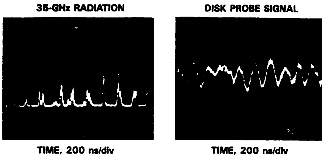
Figure 12. Electrostatic fluctuations have the same frequency components as the output radiation.
