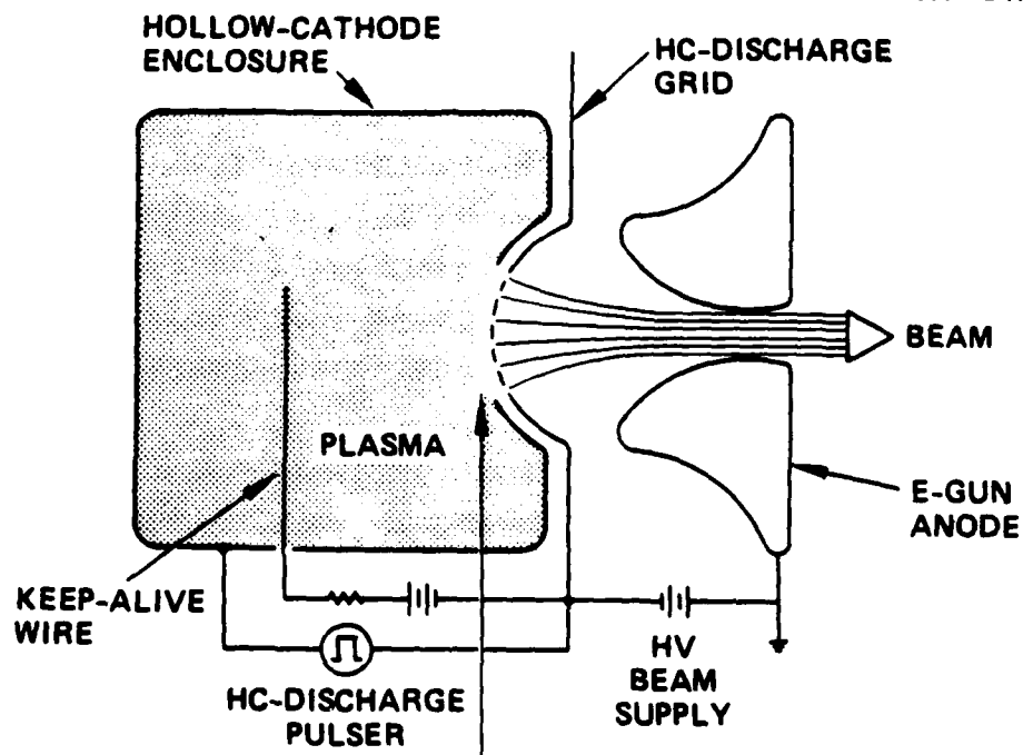
Figure 27. Hollow-cathode-plasma electron-gun configuration.
