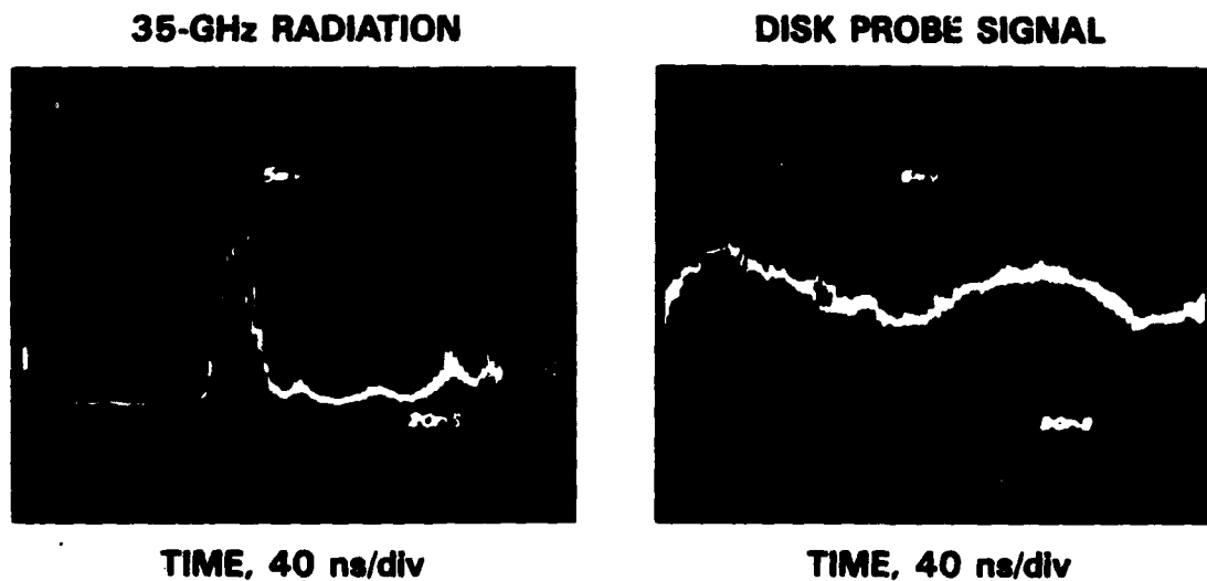
Figure 13. The radiation and the disk probe signal are compared using a faster oscilloscope time scale.
