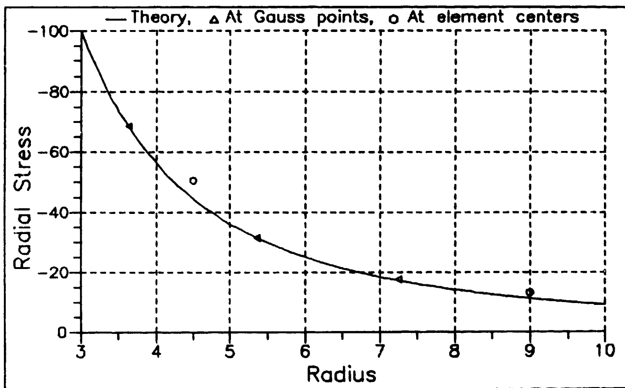
Figure 14b. Model 5: numerical prediction of \sigma_{rr} versus theory.
