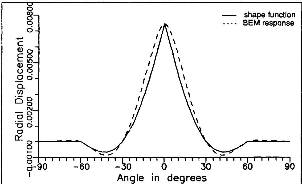
Figure 21. "Model 3": u_r along \Gamma due to a radial load of 1000 applied at a extreme node.
