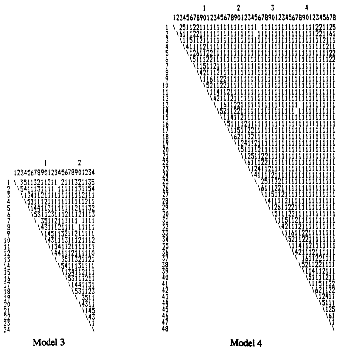
Figure 13. Asymmetry in the stiffness matrices of circular cavity models 3 and 4.
