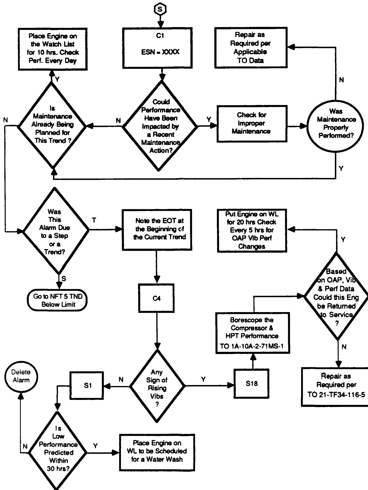
Figure 15. Sample: T.O. No. 1A-10A-2-71MS-5 Troubleshooting Algorithm.
