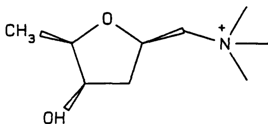
c. epimuscarine
