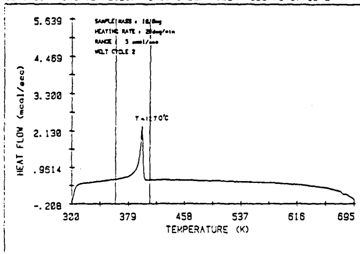
Figure 2.2.10(B): Thermal Analysis of Ethylene Glycol Milled- \text{YBa}_2\text{Cu}_3\text{O}_{7-x} Green Fiber With HDPE Blend Above: First Heating Cycle in Nitrogen Below: Second Heating Cycle in Nitrogen
