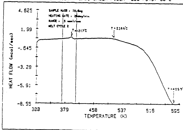
Figure 2.2.10(A): Thermal Analysis of Ethylene Glycol Milled- \text{YBa}_2\text{Cu}_3\text{O}_{7-x} Green Fiber With HDPE Blend Above: First Heating Cycle in Air Below: Second Heating Cycle in Air
