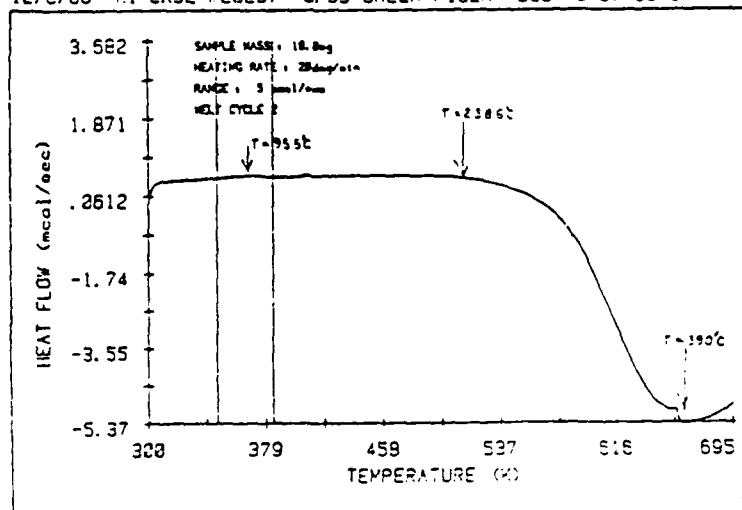
Figure 2.2.11(A): Thermal Analysis of Ethylene Glycol Milled-YBa 2 Cu 3 O 7-x Green Fiber With EVA Blend Above: First Heating Cycle in Air Below: Second Heating Cycle in Air
