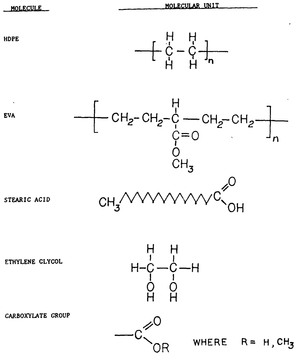
Figure 2.2.12: Molecular units of HDPE, EVA, Stearic Acid and Ethylene Glycol
