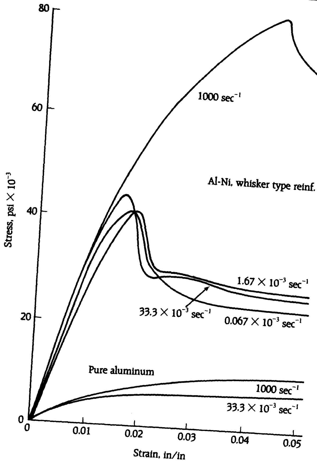
Figure 32 - Stress - Strain Curves Al-Al 3 Ni Composite, Reference [25]
