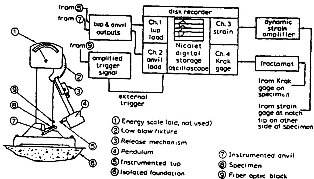
Figure 2. Modified instrumented Charpy impact testing system (17, 25, 26).
