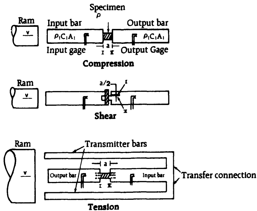
Figure 22 - Schematic Compression, Shear, Tension SHPB Arrangements, Reference [20]
