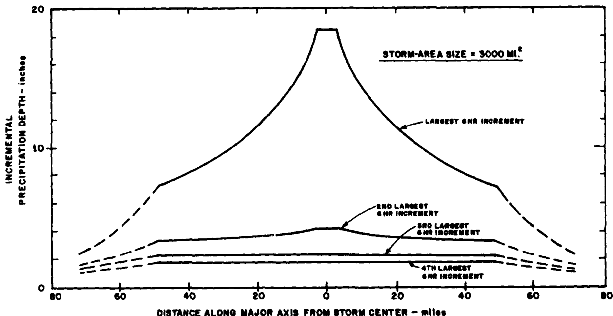
Figure 6. Spatial Variation in PMP Intensities
