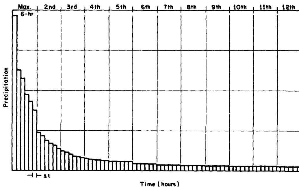
Figure 23. Incremental PMS Depth Histogram
