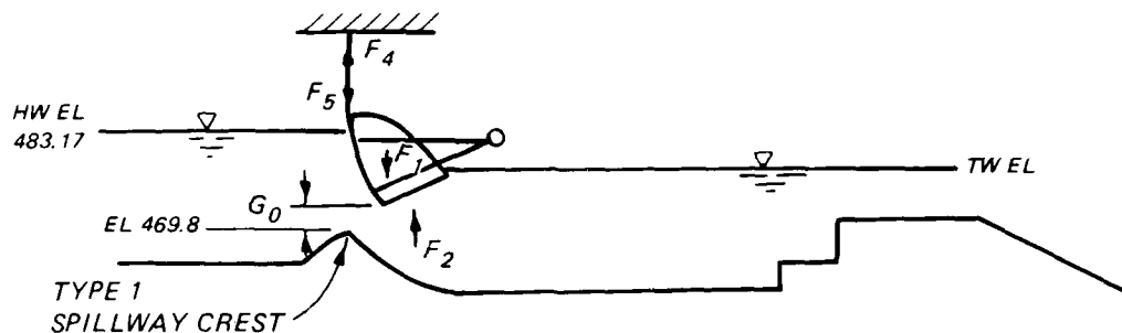
RAISED GATE DEFINITION SKETCH
