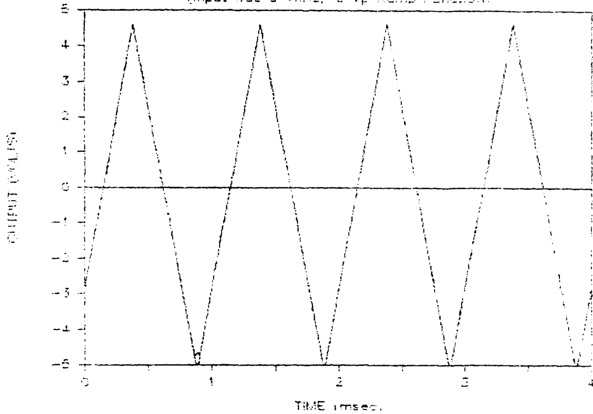
Figure 3. Recorder No. 5 with Ramp Input.
