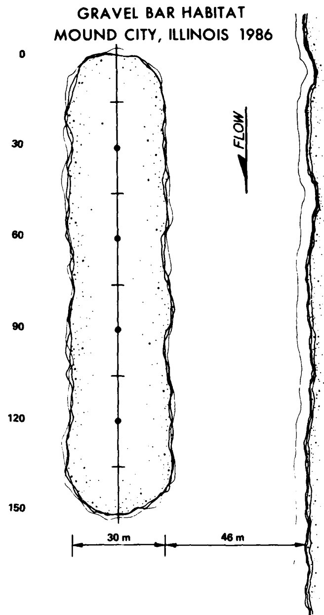
Figure 4. Diagram of the completed gravel bar habitat in the Ohio River
