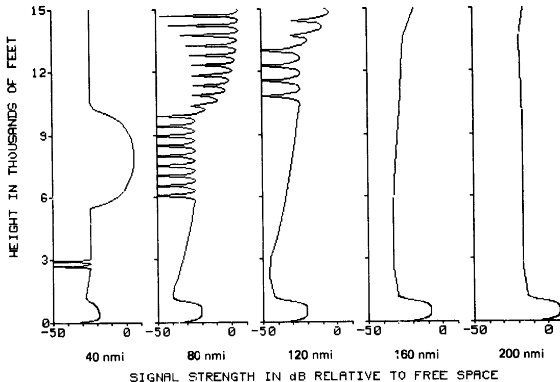
Figure 84. Sample ECM effectiveness display.
