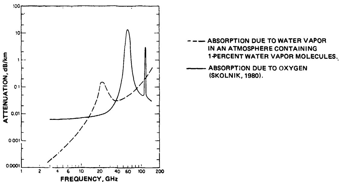
Figure 3. Attenuation of electromagnetic energy by atmospheric gases in an atmosphere at 76-cm pressure.
