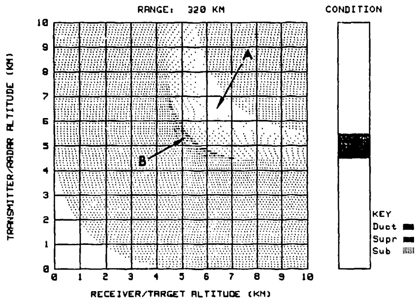
Figure 79. Conventional ray trace and AEW stationing aid for an elevated superrefractive layer.
