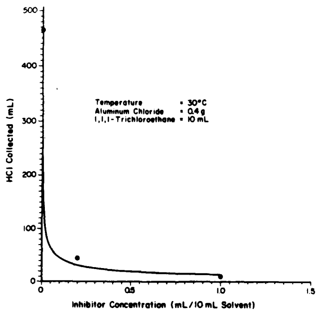
Figure 67. Effect of 1,4-dioxane on HCl collected.
