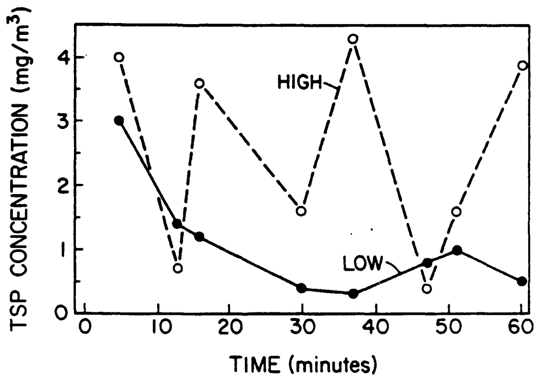
Fig. 3.8b Variation of TSP concentration ( \text{mg/m}^3 ) for wood smoke with burn time (min) showing the effect of sampling location.
