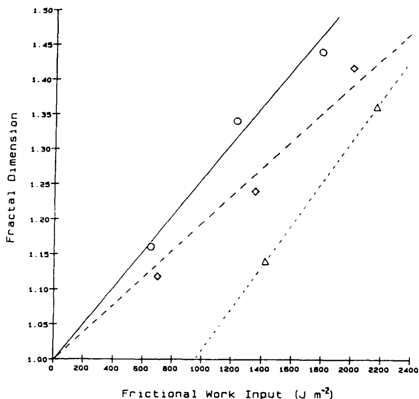
Figure 11 Fractal dimension of debris ad a functional work input ( \Delta ) Blend, ( \diamond ) NR, ( \circ ) PBD.
