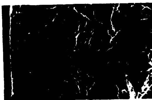
Figure 18. Fractograph of a PP specimen that failed by tearing instability; ductile failure on left and brittle on right. Prabhat and Donovan (19).
