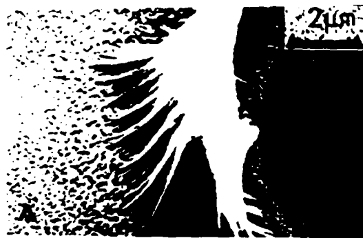
Figure 8. Bundle of fractured fibrils, with roots of fibrils to the left and a cleavage like fracture surface to the right. Doyle (8).
