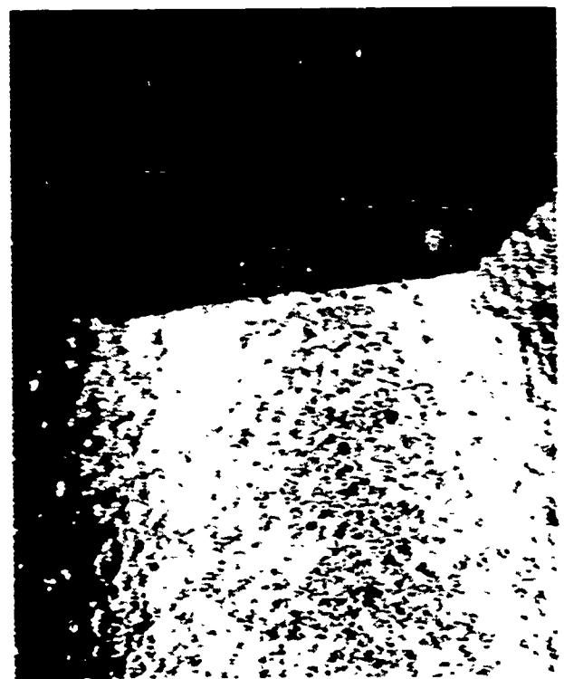
FIGURE 21 - 4340 STEEL AIRMELT 40/42 HRC AT 0.0060A, EXTERNAL FAILURE MODE AT MACHINE MARK - PEENING DID NOT OVERCOME RISER DUE TO GRIND MARK, 40X
