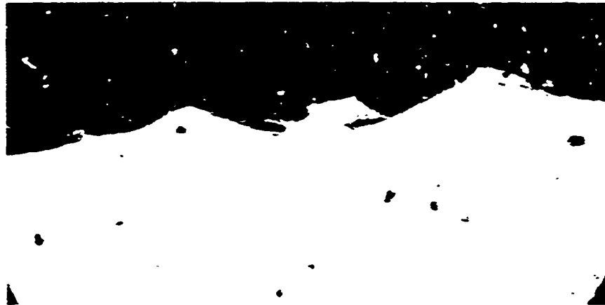
FIGURE 12 - 7075-T73 AT 0.0145A, PSEF IN BOTTOM OF ANOTHER IMPINGEMENT
