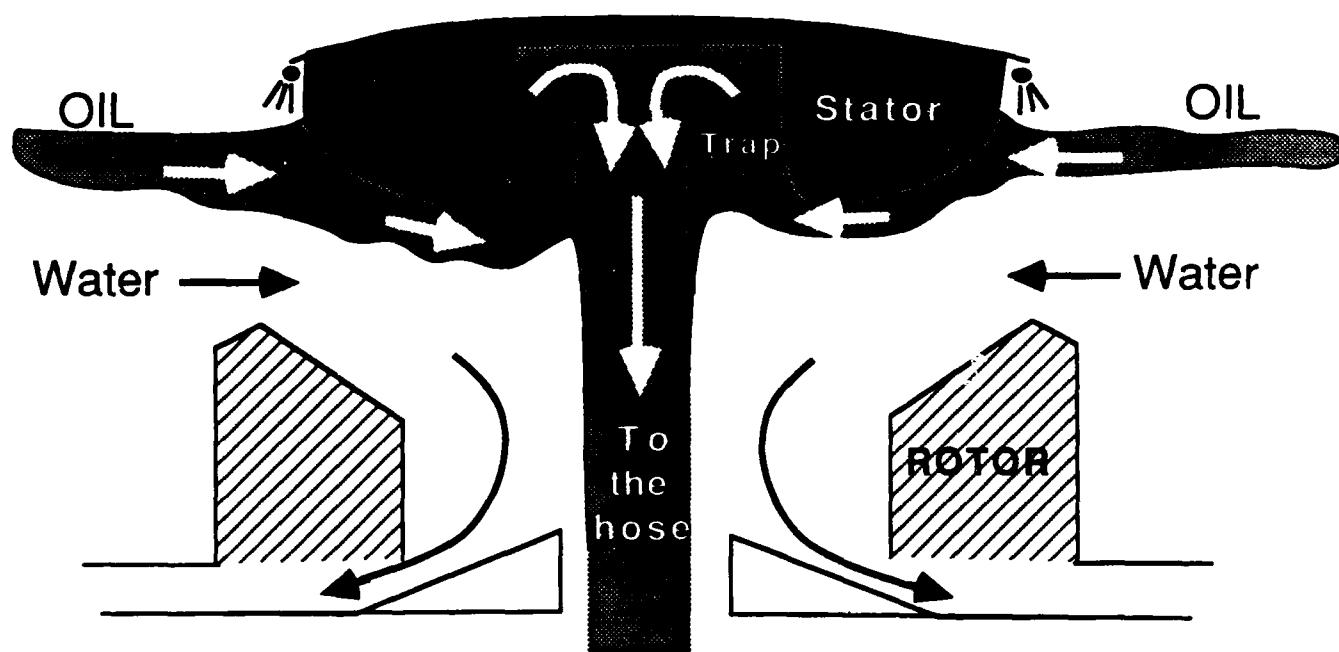
CUTAWAY VIEW
