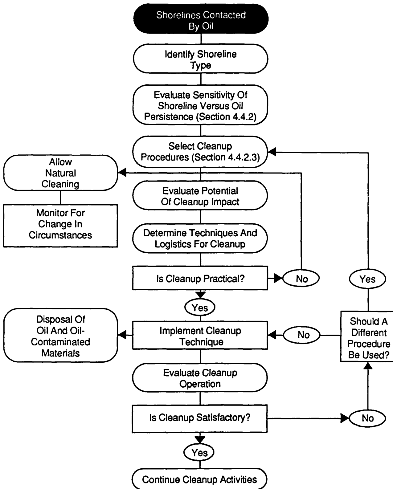
Shoreline Response Decision Tree - B
