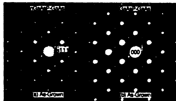
FIG. 1. Diffraction patterns on (110) cross sections for (a) InGaAsP and (b) GaAsP epitaxial layers grown on (100) GaAs substrates by MOCVD. The 1/2\ 1\bar{1}1 satellite diffraction spot of (a) is skewed along the [1\bar{1}5] direction.
