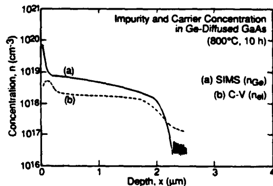
FIG. 1. Undoped bulk GaAs diffused with Ge at 800\text{ }^\circ\text{C} (10 h) from a vapor source. (a) shows the Ge concentration as measured by SIMS. (b) shows the electron concentration measured using C-V electrochemical profiling in the Ge-diffused region. The Ge diffuses into the GaAs largely compensated.
