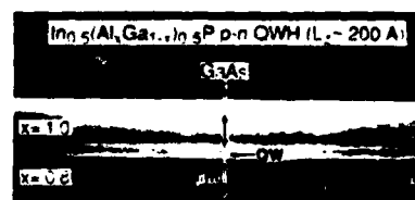
FIG. 1. Scanning electron microscope (SEM) image showing in cross section the active region of a p - n \text{In}_{1-y}(\text{Al}_x\text{Ga}_{1-x})_y\text{P}-\text{In}_{1-y}(\text{Al}_x\text{Ga}_{1-x})_y\text{P} quantum well heterostructure (QWH) grown lattice matched on GaAs with the use of metalorganic chemical vapor deposition (MOCVD). The layer compositions ( x ) are indicated along the left edge.
