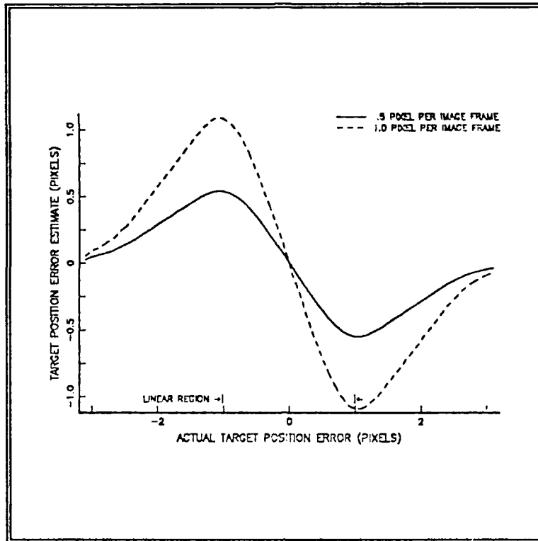
Figure 6-4. Estimated Position Error Versus Actual Position Error (Target Track 45 Degrees); \sigma_s^2=2.0 , r_2^n(0)=.7 for .5 Pixel per Frame, r_2^n(0)=.5 for 1.0 Pixel per Frame
