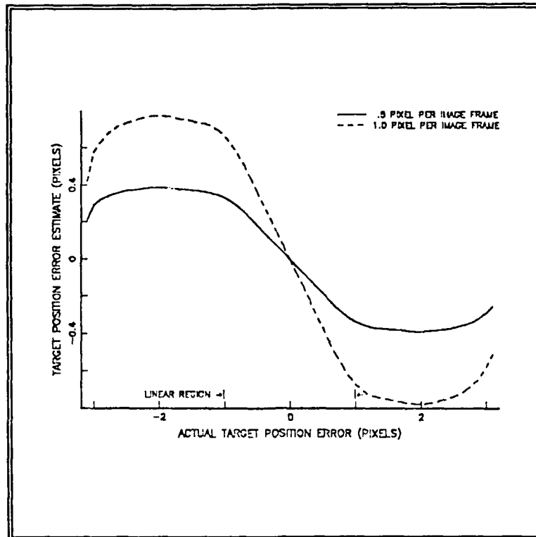
Figure 6-6. Estimated Position Error Versus Actual Position Error (Target Track 45 Degrees); \sigma_s^2=2.0 , r_z^n(0)=.1 for .5 Pixel per Frame, r_z^n=.2 for 1.0 Pixel per Frame
