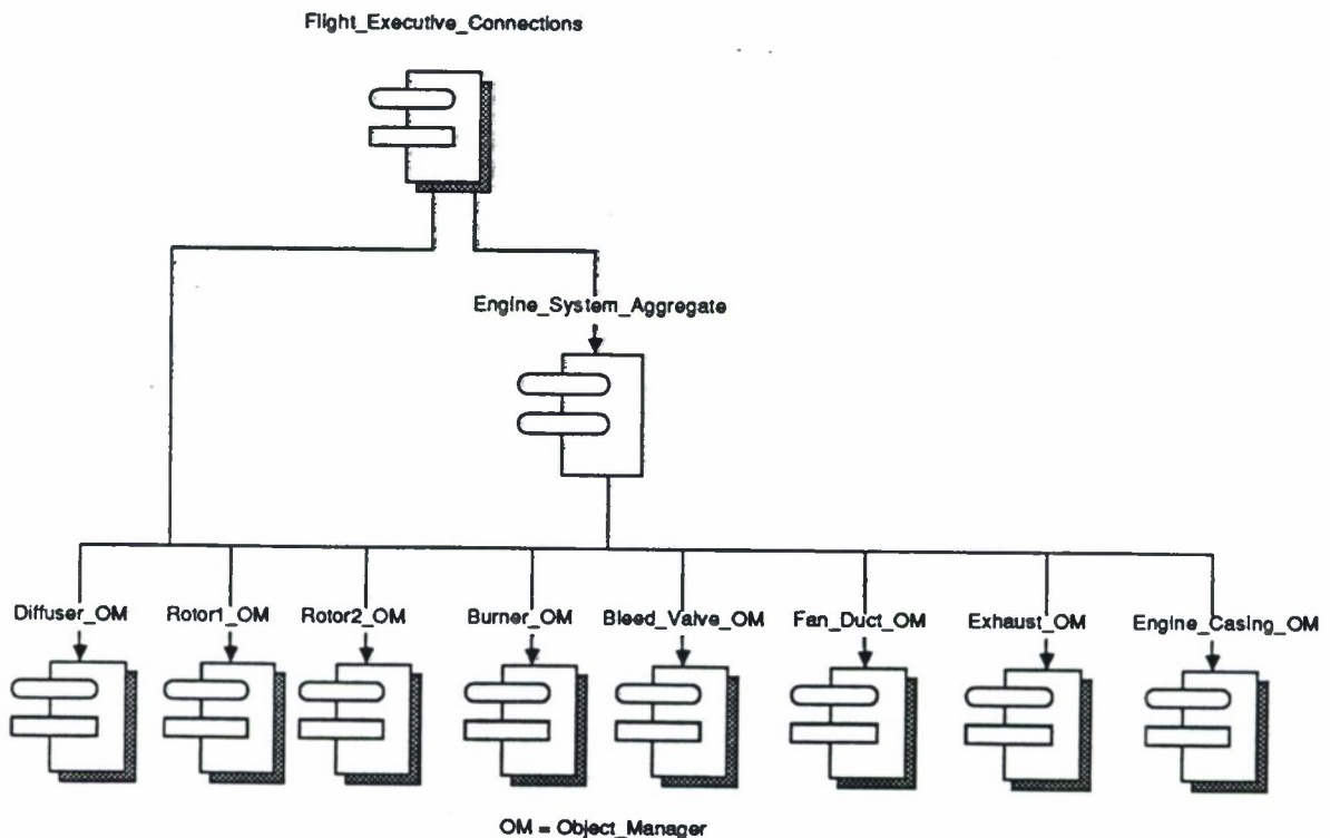
Figure 3-3: Connection Manager Software Architecture
