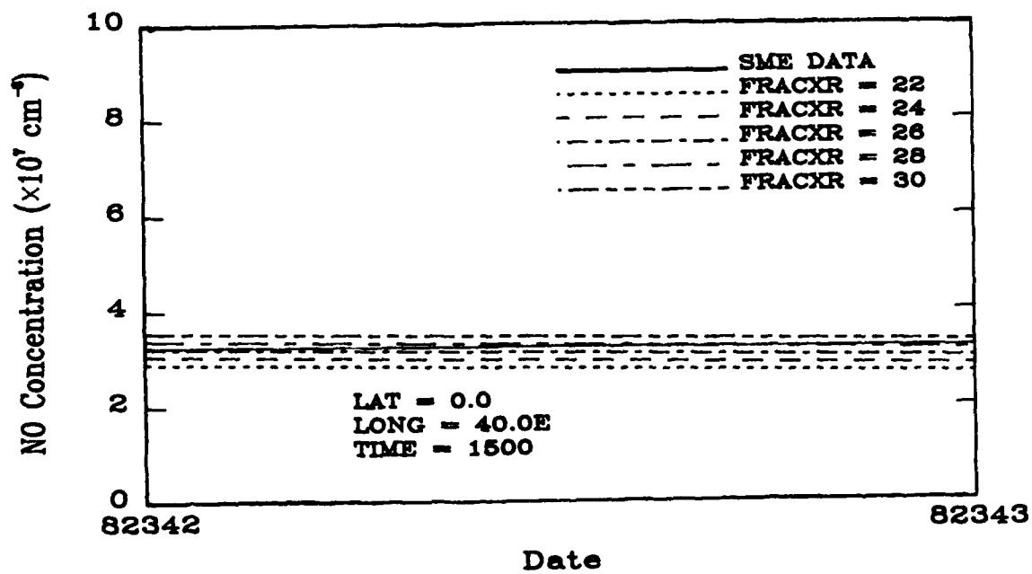
Figure 5.9. Model [NO] densities for F10.7 = 242
