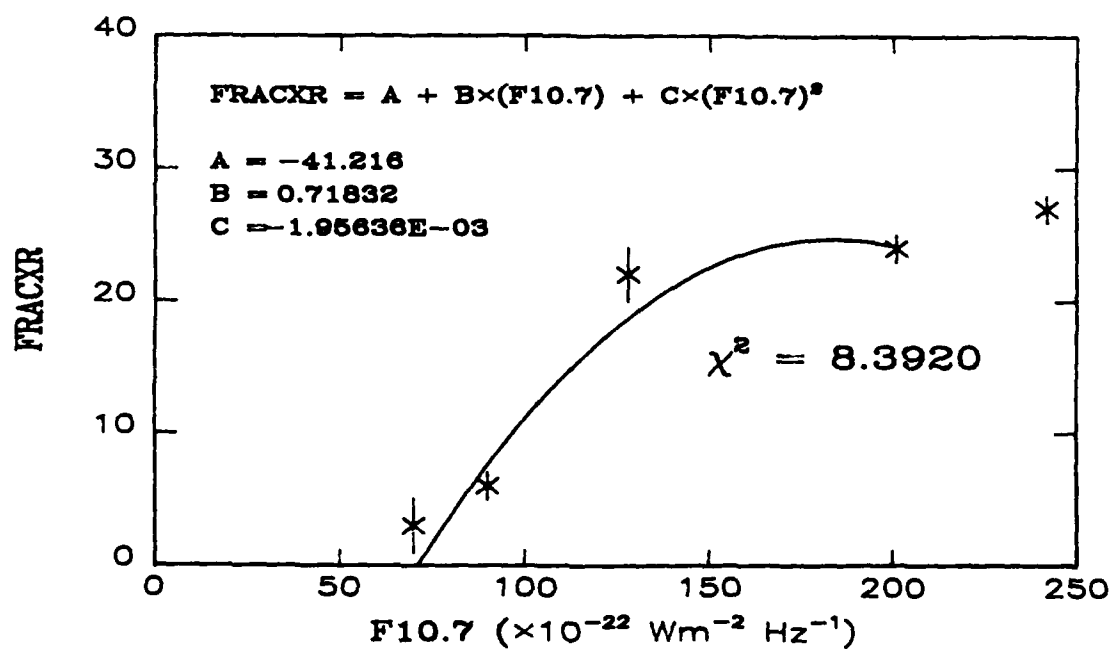
Figure 5.11. Weighted Quadratic Fit.
