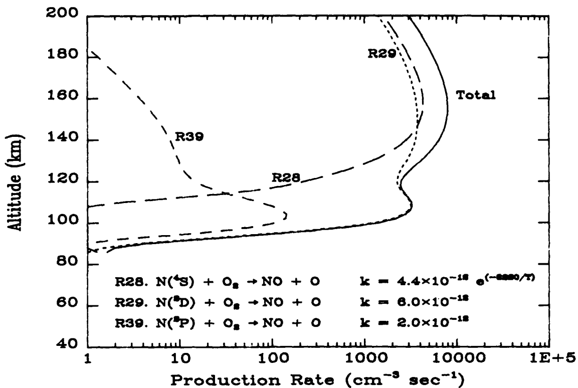
Figure 3.2. NO Production Rates
