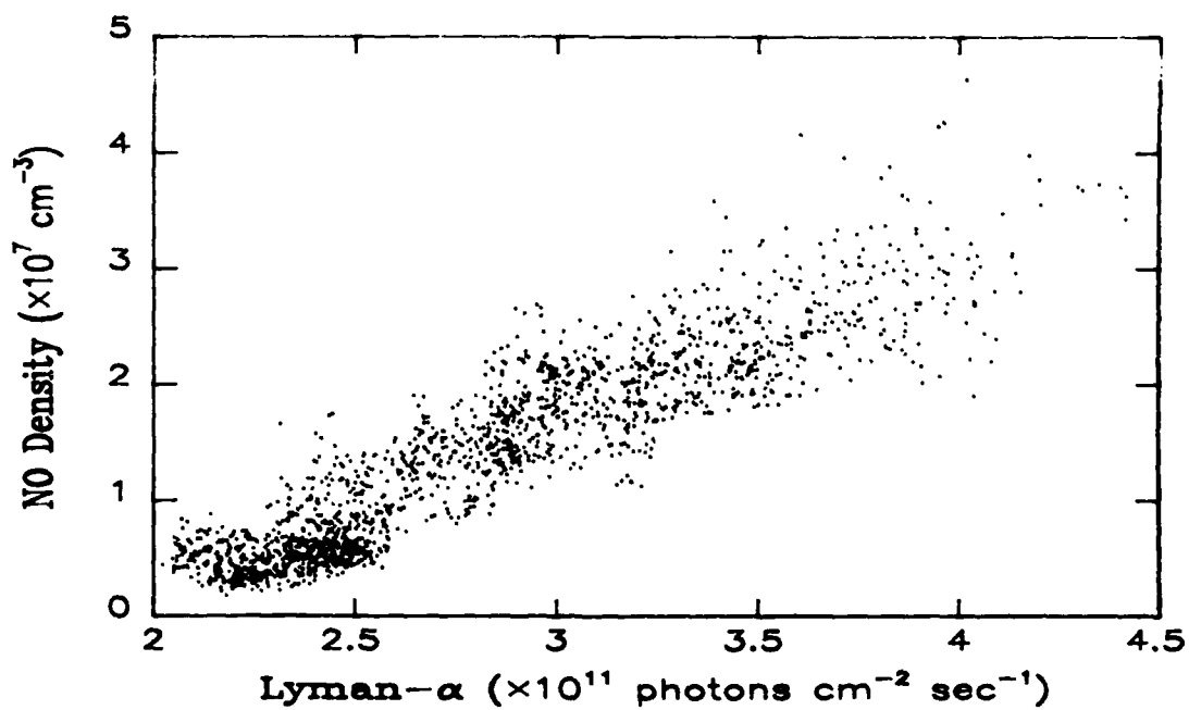
Figure 7.2. Correlation of NO and Lyman- \alpha .
