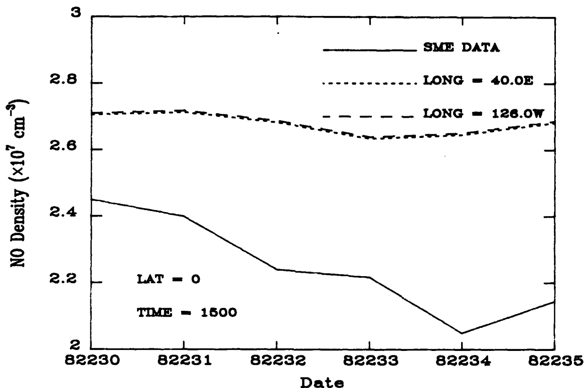
Figure 5.3. Model [NO] calculations for two different longitudes.
