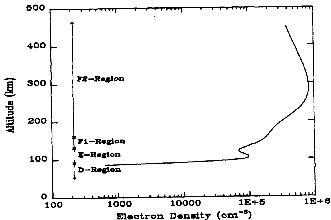
Figure 2.1. Regions of the Ionosphere.
