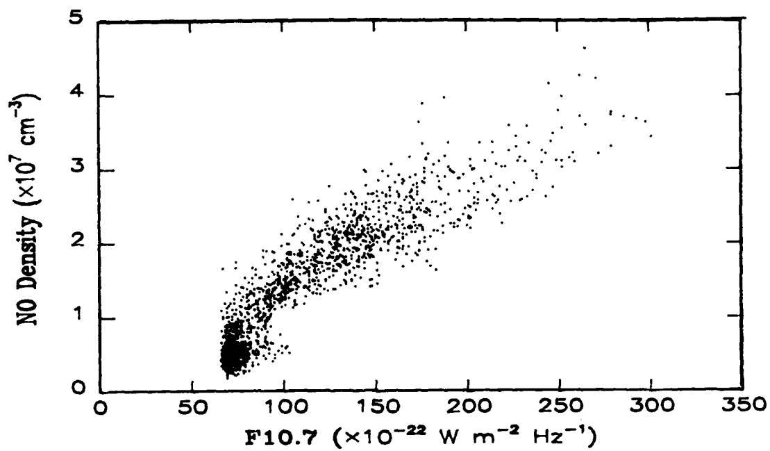
Figure 7.1. Correlation of NO and F10.7.
