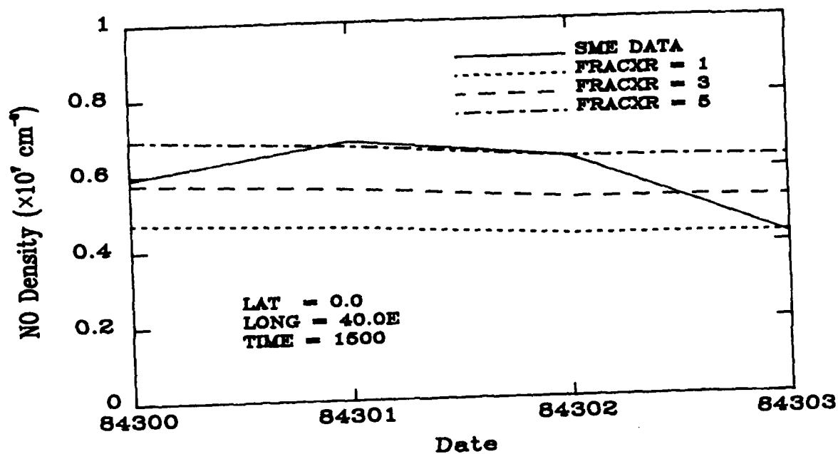
Figure 5.4. Model [NO] densities for F10.7 = 70.
