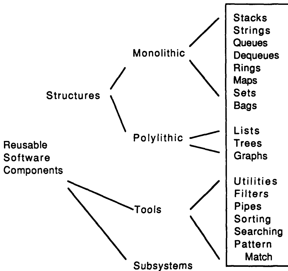
Figure 3. Booch Taxonomy
