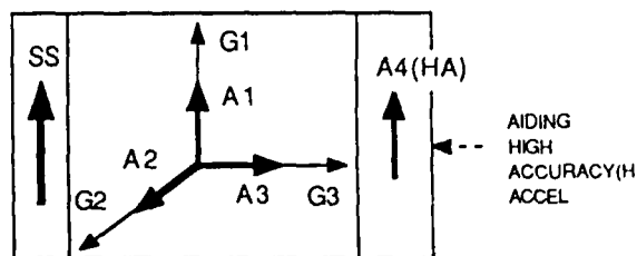
(2) SD/3A + 4TH THRUST AXIS ACCEL: (SD/4A)
