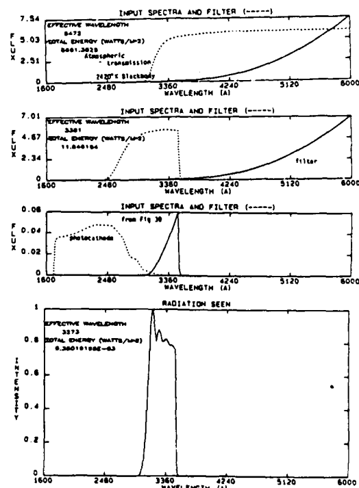
Figure 20. Convolved UV Camera System With Source Radiation
