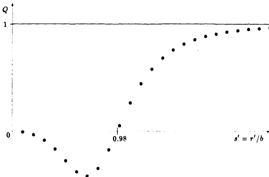
Figure 2: The electric charge of a spin 1/2 twiston plotted as a function of radius and normalised to behave like 1 for large s' .
