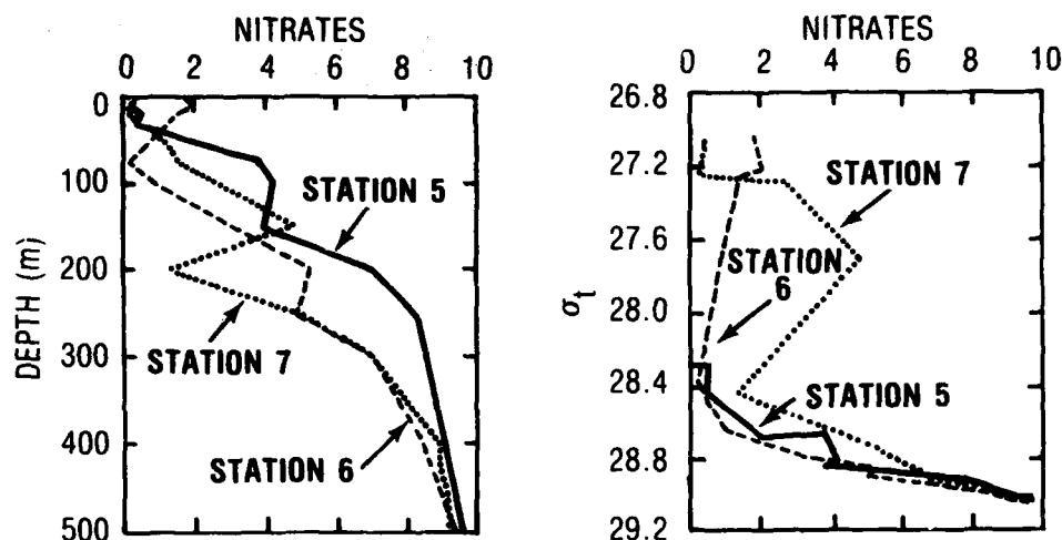
FIG. 9. Vertical nitrogen versus depth (a) and sigma- t (b) for section B.
