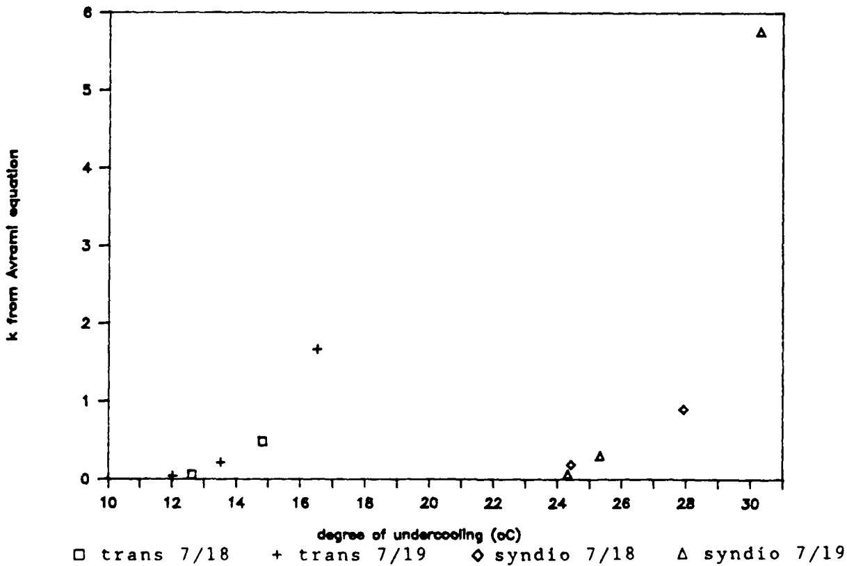
Figure 3: k(avg) vs. Undercooling
