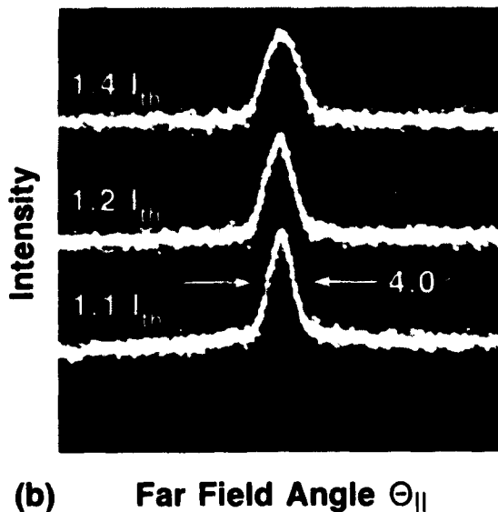
Fig. 1. (a) Spectrally resolved lateral near field and (b) far field patterns of a typical 50 \mu\text{m} gain-guided BA laser.
