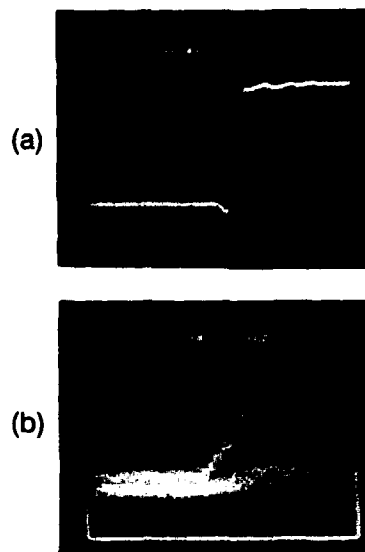
Fig.2. Wavelength-selection-time measurement. (a) DFB amplifier tuning-current waveform showing risetime < 200 ps. (b) Receiver output waveform showing wavelength-selection risetime \approx 1 ns. Upper trace of (b) is due to marks in the incident bitstream; lower trace is due to spaces.
