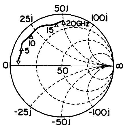
Fig.2 Smith chart plot of measured impedance.
