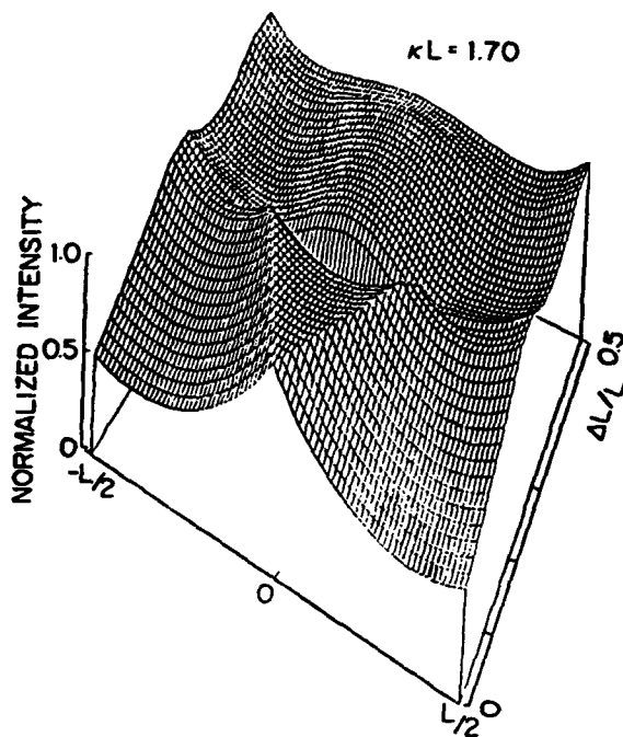
Fig.2 Axial intensity distributions of 2 \times \lambda/8 structures ( as a function of \Delta L/L )
