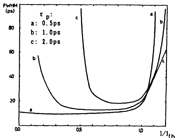
Fig. 4. Calculated D.C. bias dependence of the pulse width with different photon lifetimes. \tau_p = 0.5\text{ps} corresponds to a LD of about 95 \mu\text{m} and \tau_p = 1\text{ps} corresponds to a 140 \mu\text{m} LD.
