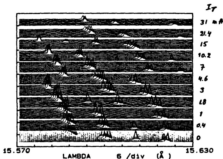
Fig. 3: \lambda vs. I_T characteristic of CT-DBR
