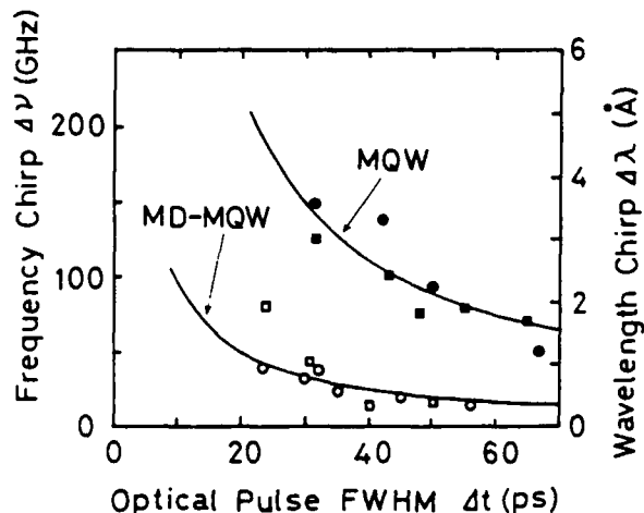
Fig. 4 Measured spectral chirping of p-type MD-MQW lasers( \circ \square ) and undoped MQW lasers( \bullet \blacksquare ).
