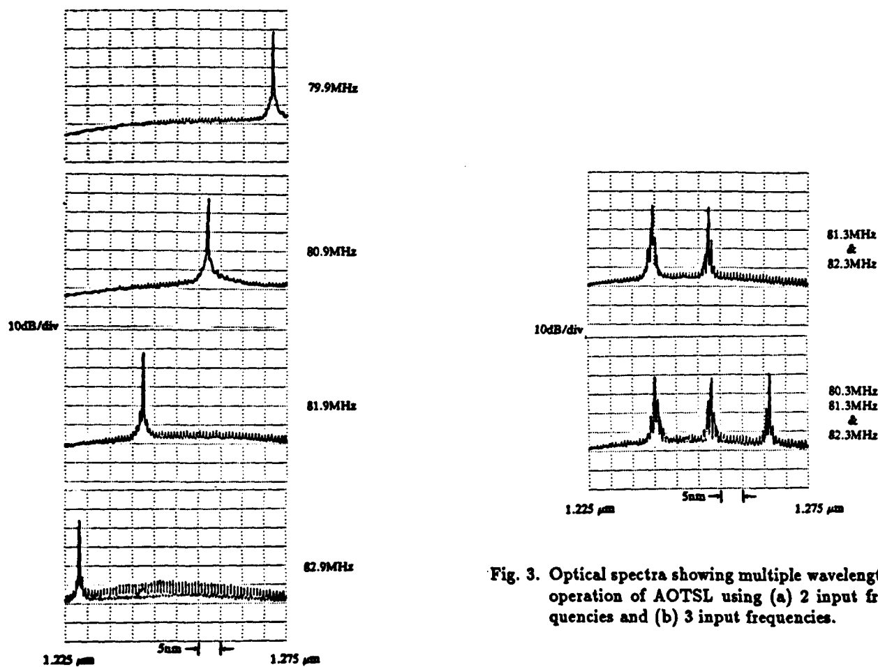
Fig. 2. Optical spectrum analyser traces of output of non-frequency-compensated AOTSL at 4 values of acoustic drive frequency, viz. F_a = 79.9, 80.9, 81.9, and 82.9\text{MHz} .
