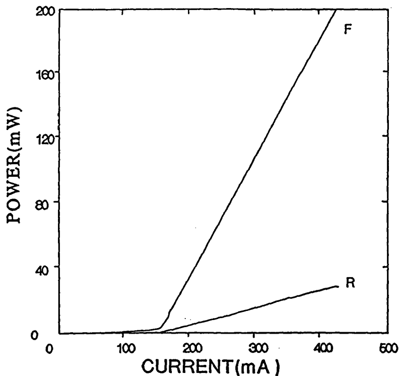
Figure 1. CW output power of front (F) and rear (R) facet of a 10-stripe \text{In}_x\text{Ga}_{1-x}\text{As-GaAs} laser with 100\text{ }\mu\text{m} aperture and 250\text{ }\mu cavity length.
