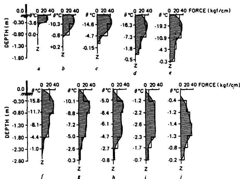
Figure 1. Distribution of relative frost-heaving forces, in kilograms-force per lineal centimeter of column perimeter, over the lateral surface of the pile (experiments of Yegerev reported by Tsyrovich 1975). z is depth in meters from the surface and \theta is the temperature in degrees Celsius.
