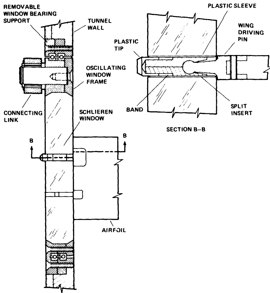
Fig. 7 Detail of airfoil support at window.
