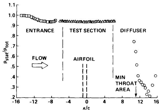
Fig. 9 Tunnel wall static pressure distribution, M_\infty = 0.3 , f = 5 Hz.
