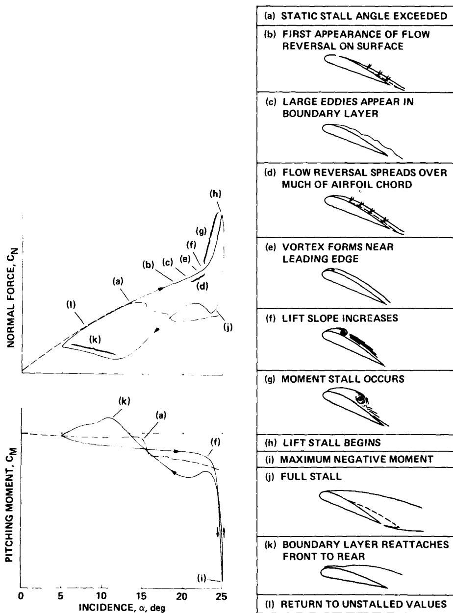
Fig. 1 Lift and moment versus angle of attack for airfoil experiencing dynamic stall. 1
