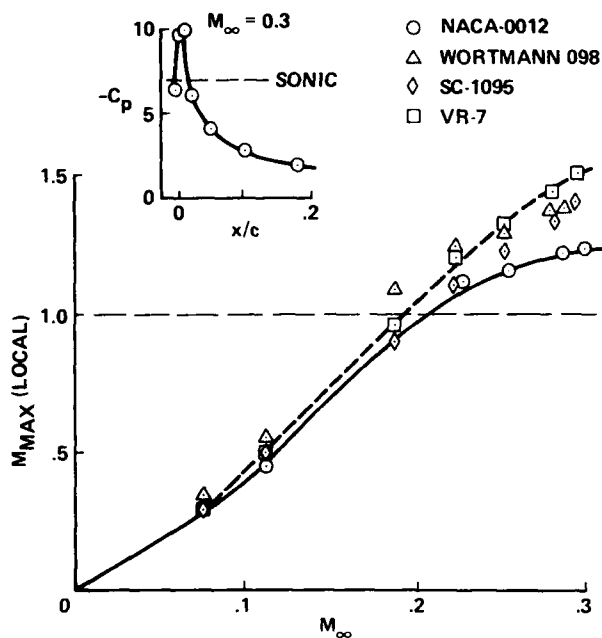
Fig. 2 Local Mach number on leading edge of oscillating airfoil versus free-stream Mach number. 2
