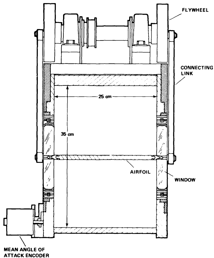
Fig. 6 End view of test section.
