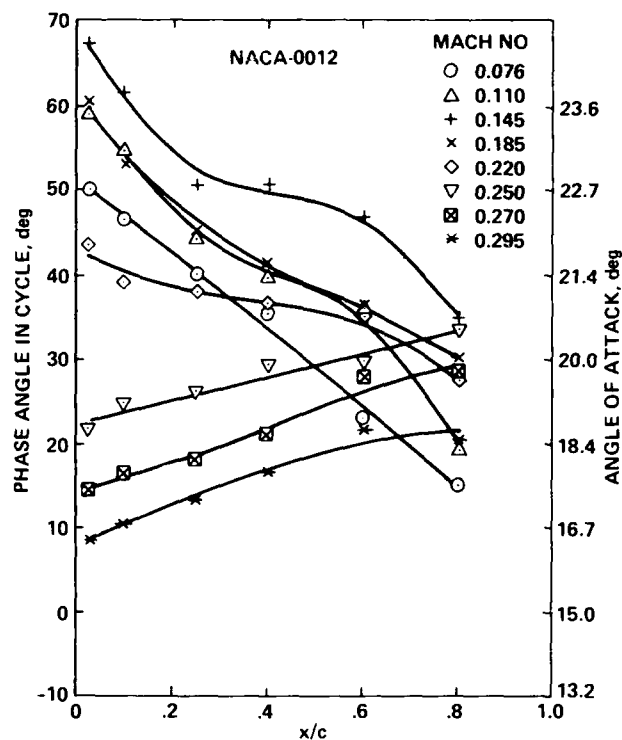
Fig. 3 Location of flow reversal on surface of NACA 0012 airfoil as a function of angle of attack for various Mach numbers for \alpha = 15^\circ + 10^\circ \sin \omega t . 2
