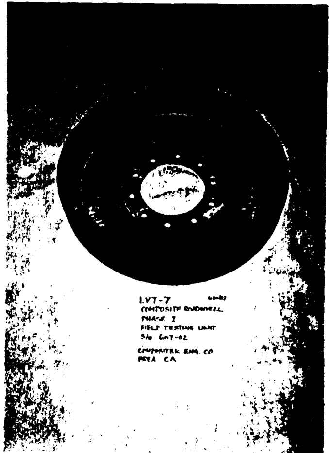
Figure 44. S/N 607-02 after Field Testing - inside view.
