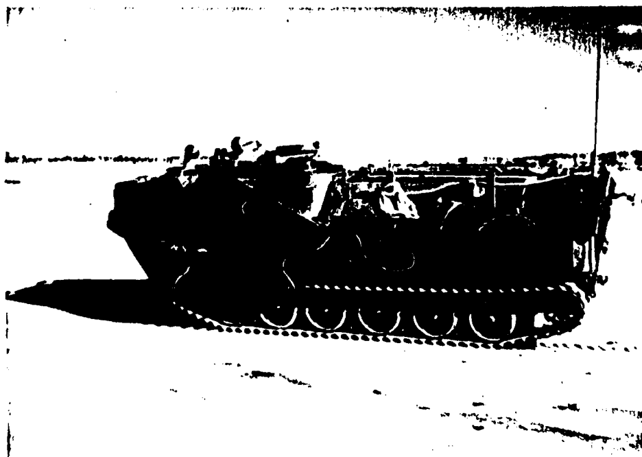
Figure 33. Composite Roadwheel Field Testing - Sea Water
