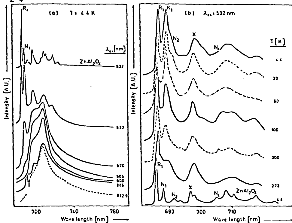
Figure 4. Comparison of the emission spectra of Cr(III) in ZnAl_2O_4 at \lambda_{ex} = 532 \text{ nm} and temperature 4.4 with Cr(III) in gahnite glass-ceramics. a at various excitation wavelengths and temperature 4.4K; b at \lambda_{ex} = 532 \text{ nm} and various temperatures [24].
