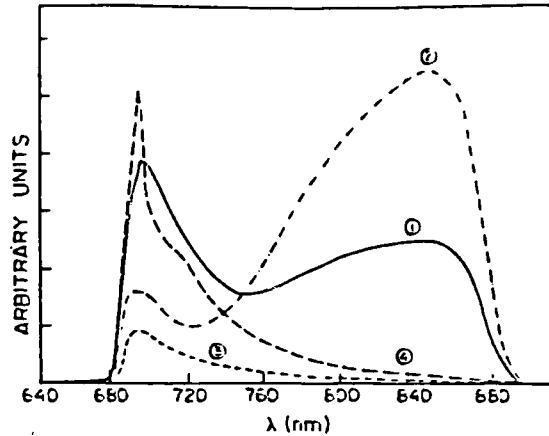
Figure 6. Emission spectrum of Cr(III)-doped parent glass under 532nm excitation at 4.4K.
