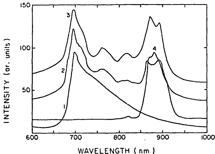
Figure 10. Emission spectra: Curve 1; 0.1 mole% Cr(III) excited at 550nm. Curve 2; 1 mole% Nd(III), 0.1 Cr(III) excited at 550nm. Curve 3; 3 mole% Nd(III), 0.1 mole% excited at 550nm. Curve 4; 3 mole% Nd(III) excited at 550nm. All samples in mullite glass-ceramics [19].
