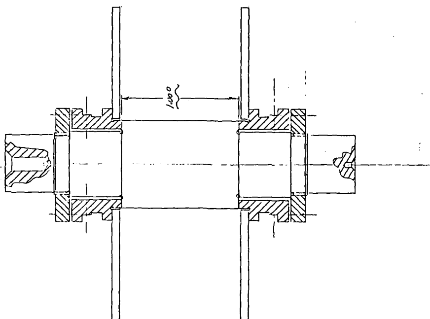
FIGURE 5-5 DISK MOUNTING AND SHAFT SUPPORT LAYOUT
