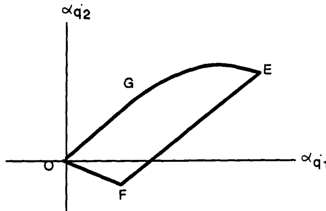
Figure 11: Image set S_{\dot{q}}
