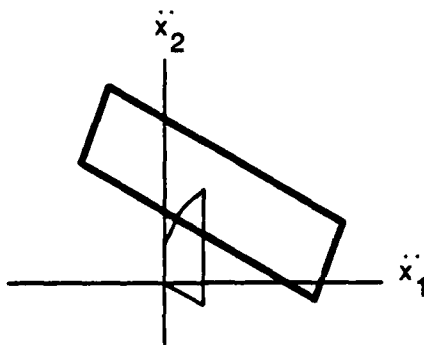
Figure 15: A local supremum
