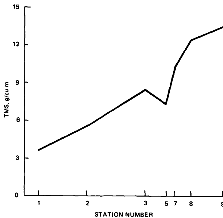
Figure 6. Longitudinal distribution of TSM concentration
