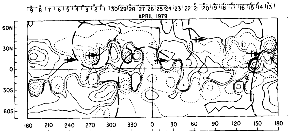
Fig. 4. Composite of two solar synoptic magnetic field maps (rotation 1680 and 1681) as in Solar Geophysical Data . Bold dashes mark potential field model sector boundaries at 2.6 R_s as in Hoeksema et al. (1983). Surface positions of five co-rotating features measured by HELIOS B are marked "→" assuming a constant velocity radial expansion.
