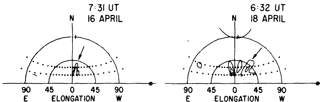
Fig. 3. HELIOS B contour plots showing a heliospheric co-rotating density enhancement (arrows mark the feature). In this presentation the Sun is centered. Electron columnar density is contoured in levels of 3 \times 10^{14} \text{cm}^{-2} upward from that level. The contours are drawn at times (given) when the 31^\circ photometers measure brightness. Data from the 15^\circ and 90^\circ photometers are interpolated to the times indicated. (a and b) Movement of the feature from east to west over a period of approximately two days from April 16 to April 18, 1979.
