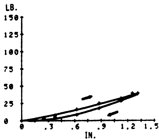
Figure 83. Skin Compliance Curves for Upper Leg-Position 1
