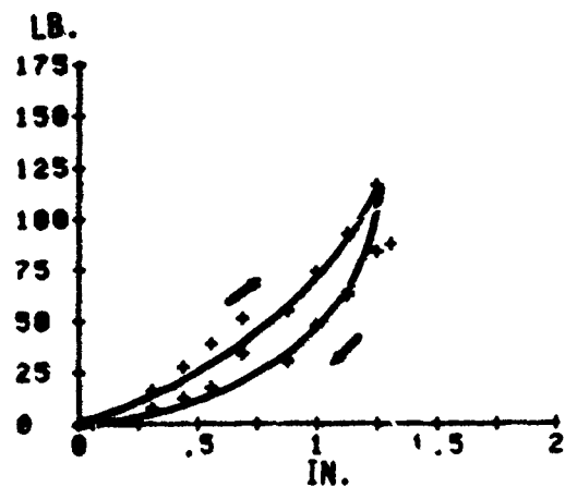
SEATED MANIKIN Figure 75. Skin Compliance Curves for Front of Thorax-Position 1
