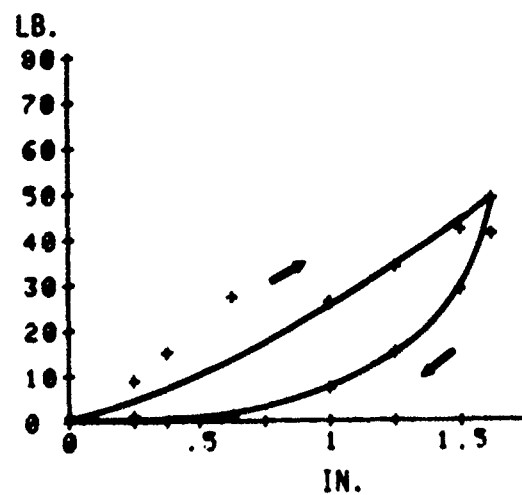
Figure 78. Skin Compliance Curves for Back of Throat
