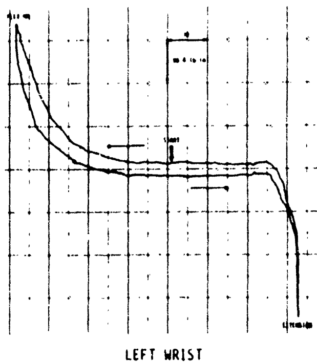
FIGURE 40. WRIST FLEXION-EXTENSION AT 180° MEDIAL ROTATION FOR SEATED MANIKIN
