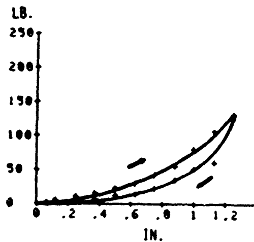
Figure 96. Skin Compliance Curves for Forearm-Position 2
