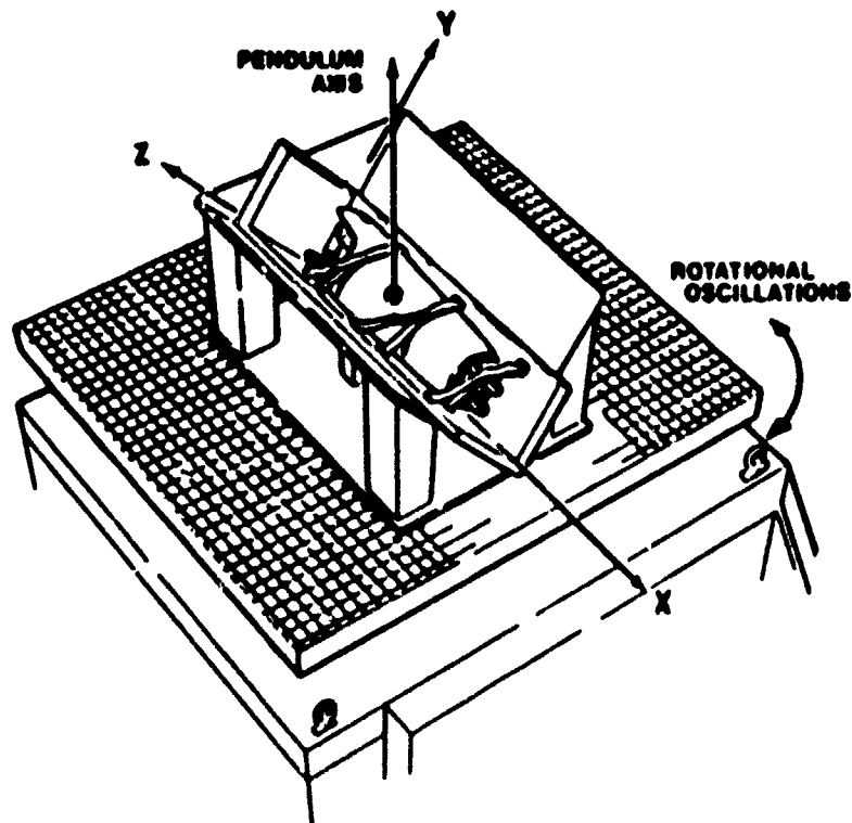
Figure 11. Forearm Mounted on MPI Platform to Determine Moment of Inertia
