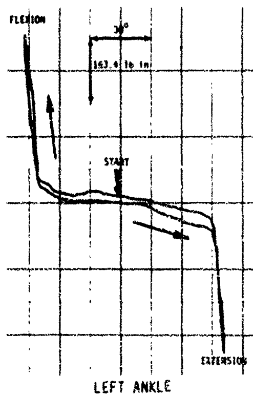
FIGURE 47. ANKLE FLEXION-EXTENSION FOR SEATED MANIKIN
