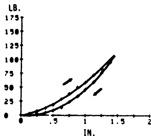
SEATED MANIKIN Figure 77. Skin Compliance Curves for Front of Thorax-Position 3
