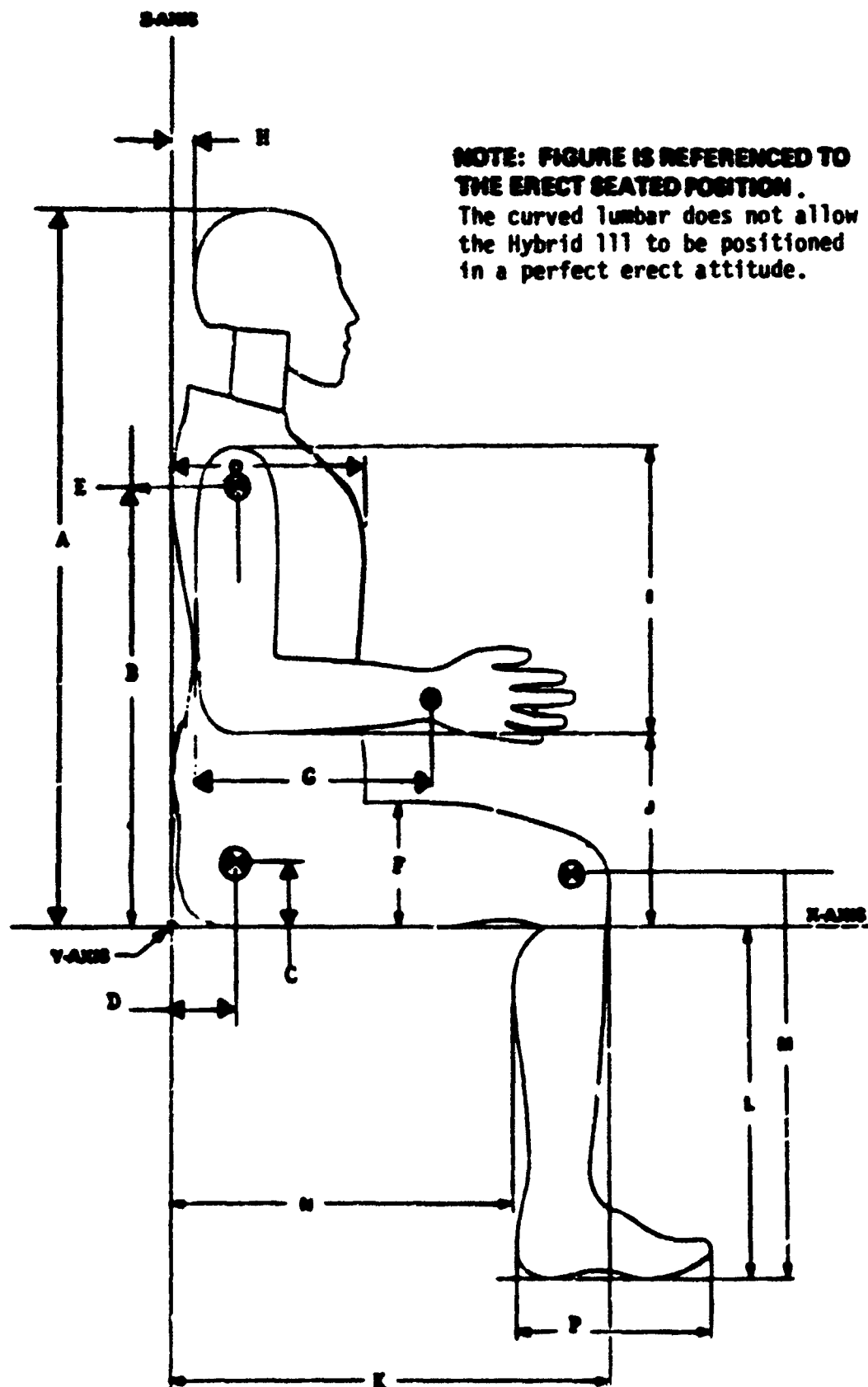
Figure 3. Hybrid 111 Exterior Body Dimensions - Side View
