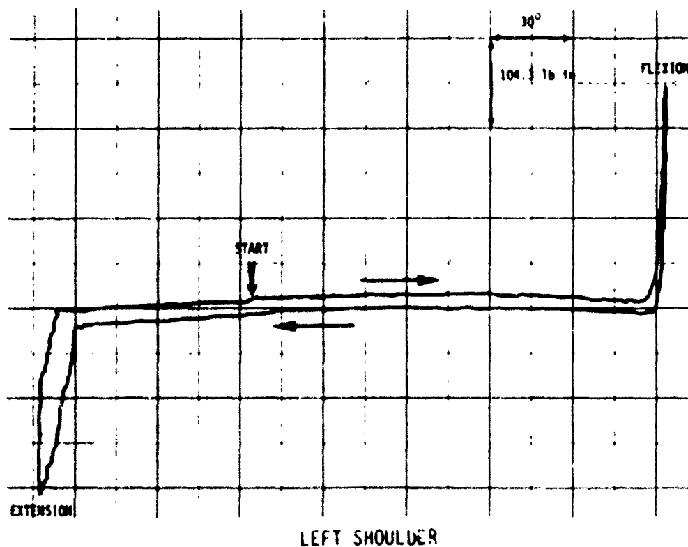
FIGURE 21. SHOULDER FLEXION-EXTENSION AT 0° ABDUCTION FOR SEATED MANIKIN
