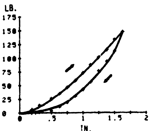
SEATED MANIKIN Figure 77. Skin Compliance Curves for Front of Thorax-Position 3
