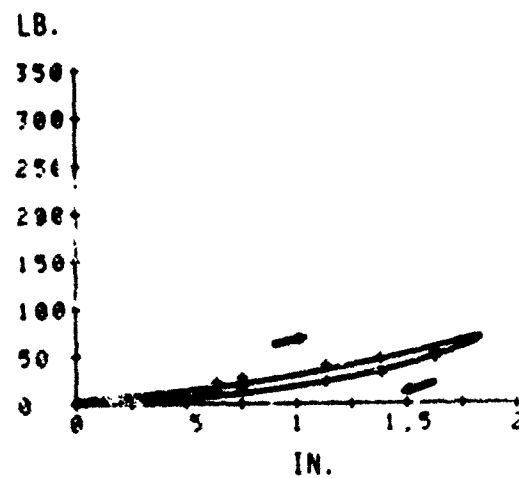
SEATED MANIKIN Figure 89. Skin Compliance Curves for Back of Lower Leg-Position 3
