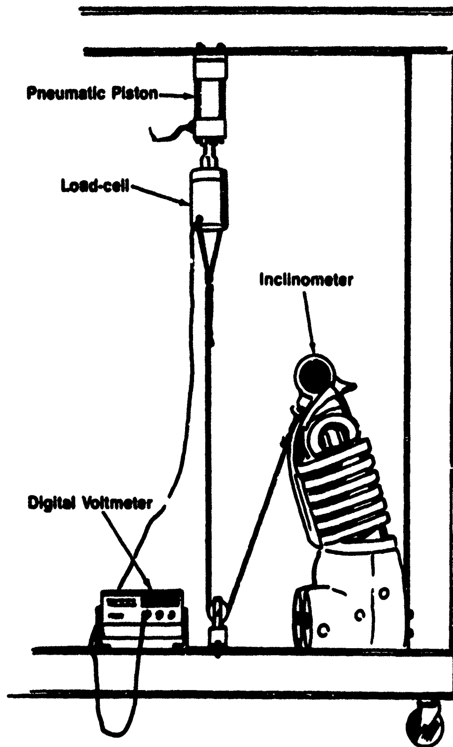
Figure 56. Lumbar Spine Flexion Test Setup with Abdomen in Place
