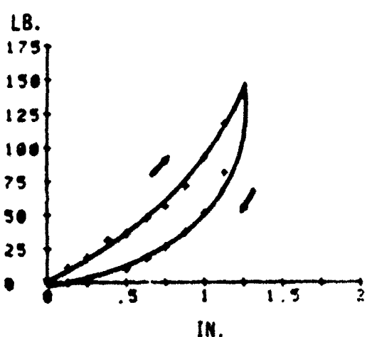
Figure 82. Skin Compliance Curves for Buttocks-Position 3
