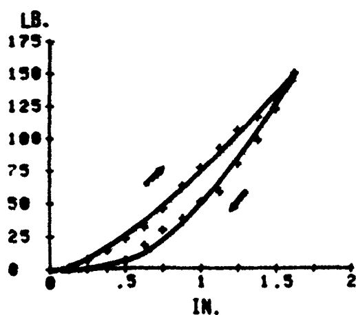
SEATED MANIKIN Figure 75. Skin Compliance Curves for Front of Thorax-Position 1
