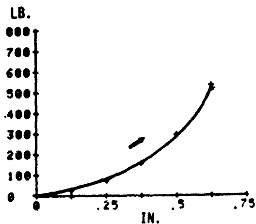
Figure 73. Skin Compliance Curves for Front of Head
