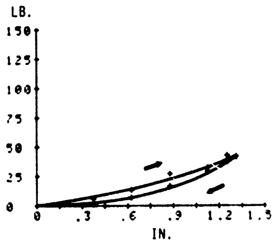
Figure 84. Skin Compliance Curves for Upper Leg-Position 2
