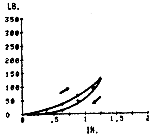
SEATED MANIKIN Figure 87. Skin Compliance Curves for Front of Lower Leg-Position 1
