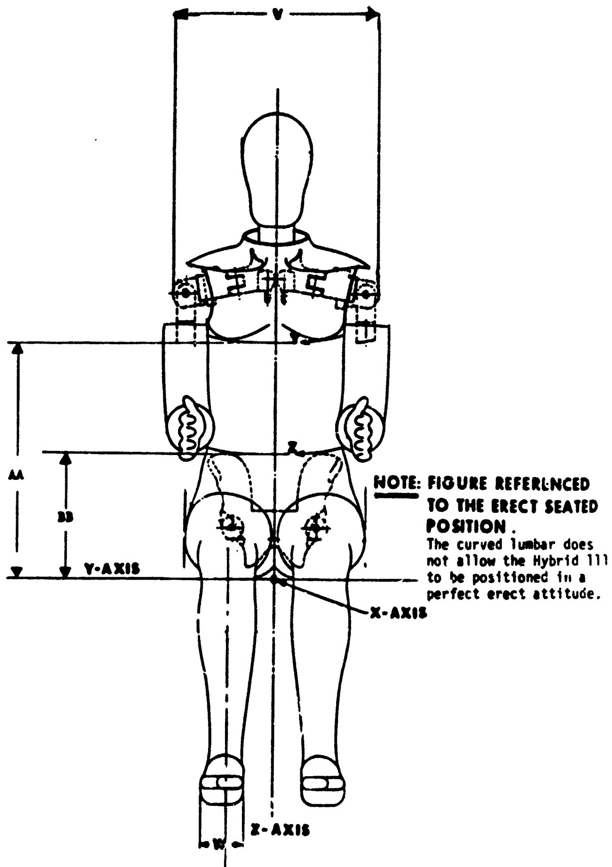
Figure 2. Hybrid III Exterior Body Dimensions - Front View
