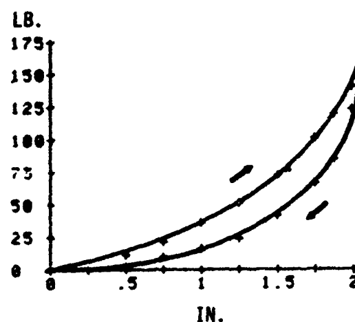
Figure 80. Skin Compliance Curves for Buttocks-Position 1
