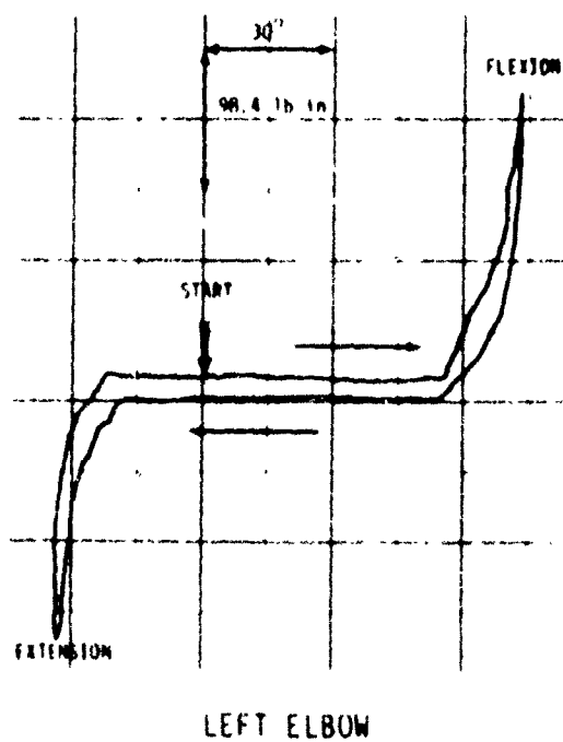
FIGURE 27. ELBOW FLEXION-EXTENSION AT 180° MEDIAL ROTATION FOR STANDING MANIKIN
