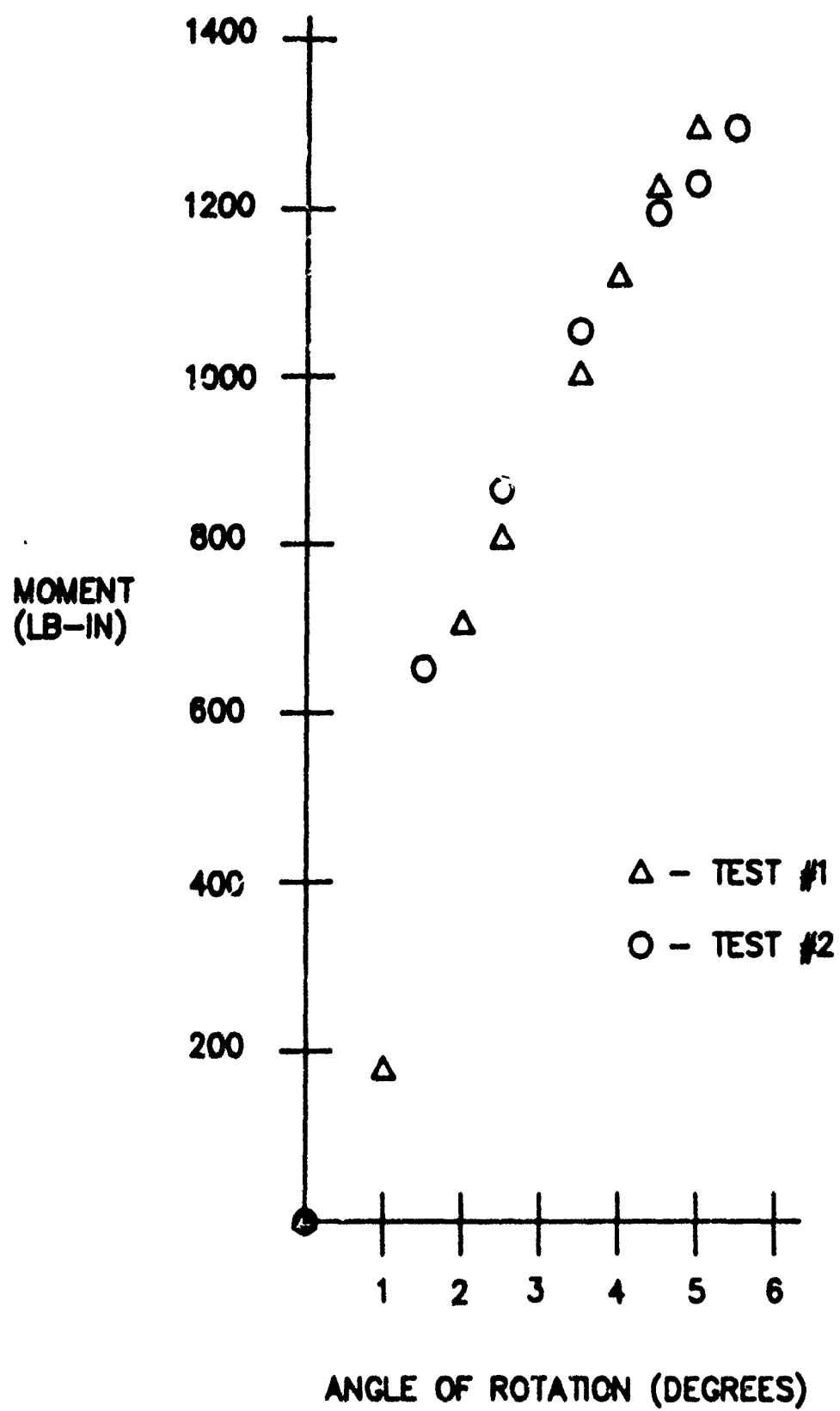
Figure 59. Curved Lumbar Spine Flexion Test
