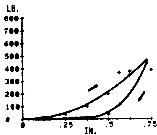
Figure 73. Skin Compliance Curves for Front of Head
