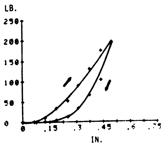
Figure 86. Skin Compliance Curves for Knee-Position 2
