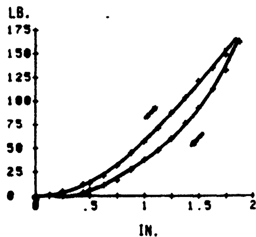
SEATED MANIKIN Figure 76. Skin Compliance Curves for Front of Thorax-Position 2
