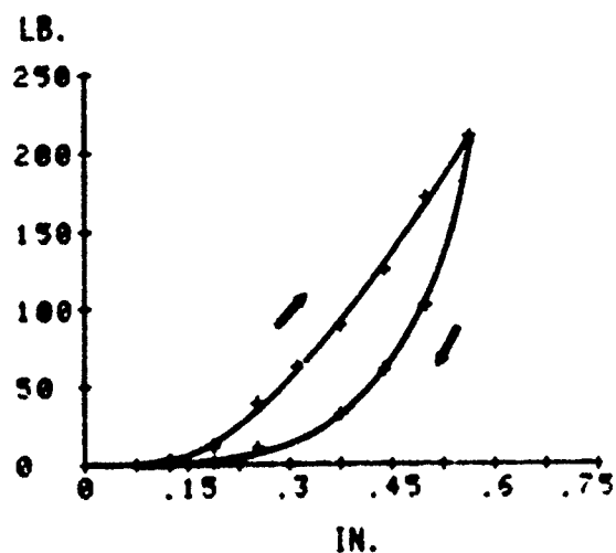
Figure 85. Skin Compliance Curves for Knee-Position 1
