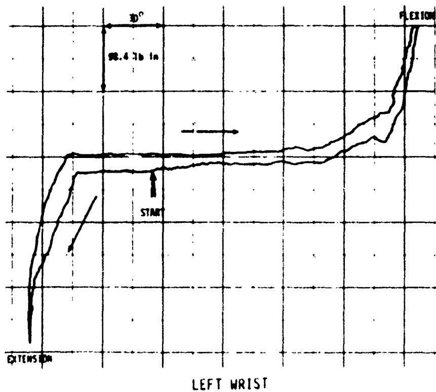
FIGURE 38. WRIST FLEXION-EXTENSION AT 0° ROTATION FOR SEATED MANIKIN
