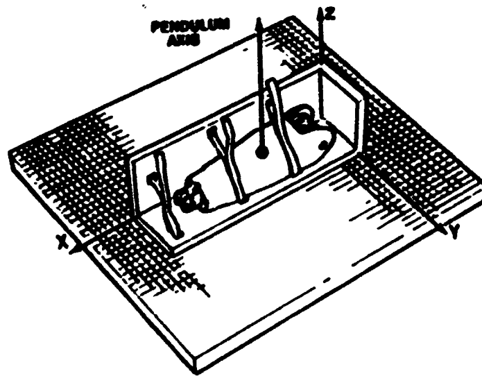
Figure 11. Forearm Mounted on MPI Platform to Determine Moment of Inertia
