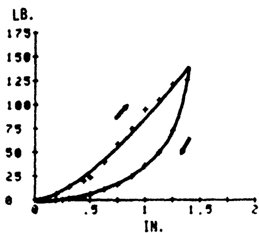
Figure 80. Skin Compliance Curves for Buttocks-Position 1
