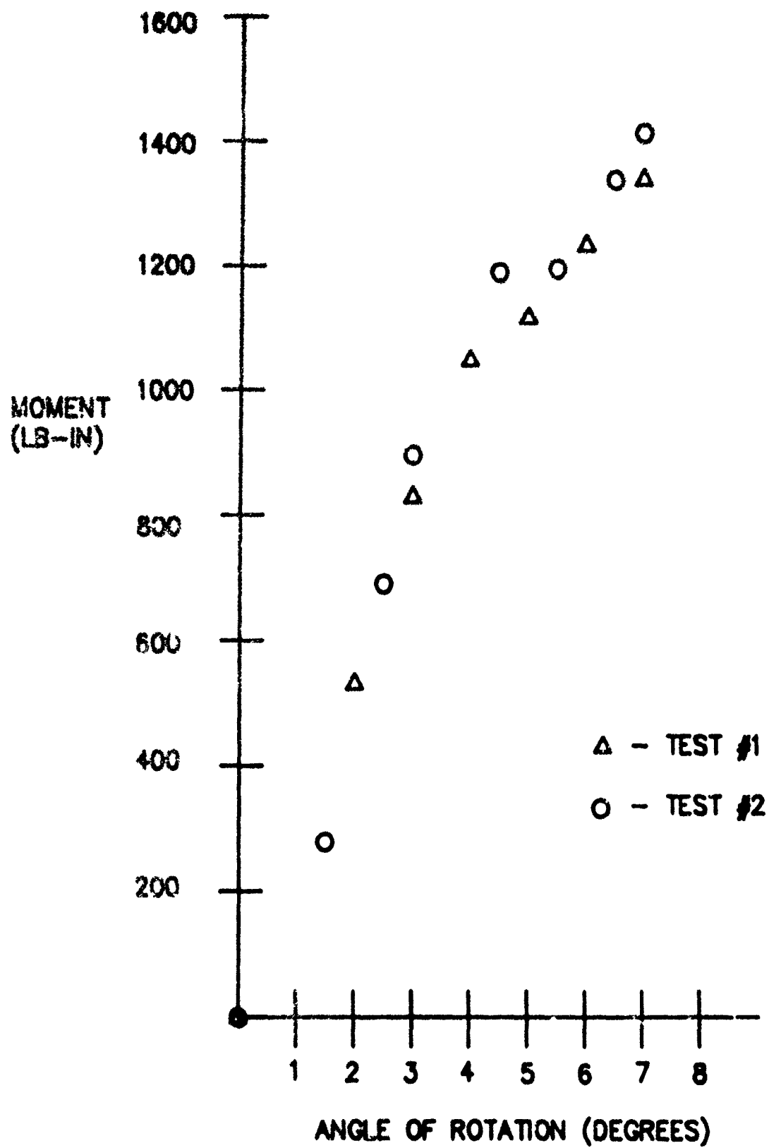
Figure 60. Curved Lumbar Spine Extension Test
