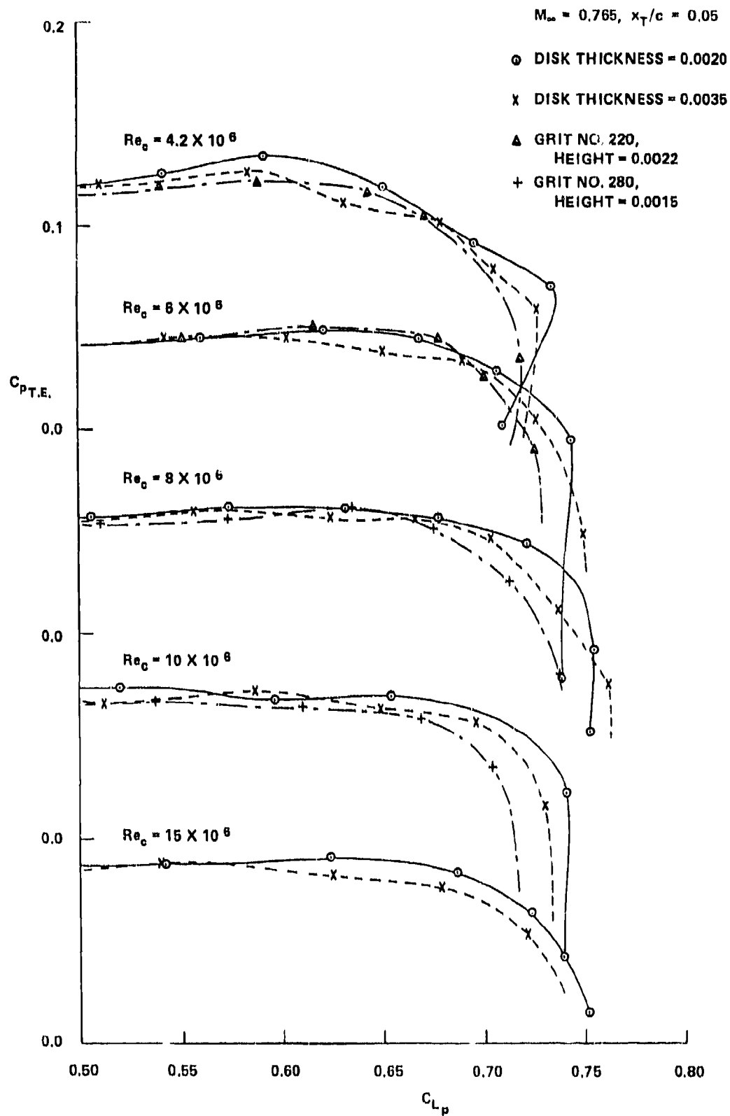
FIG. 5: TRAILING EDGE PRESSURE VERSUS LIFT AT VARIOUS REYNOLDS NUMBERS WITH DISK OR GRIT TRIPPINGS, x_T/c = 0.05
