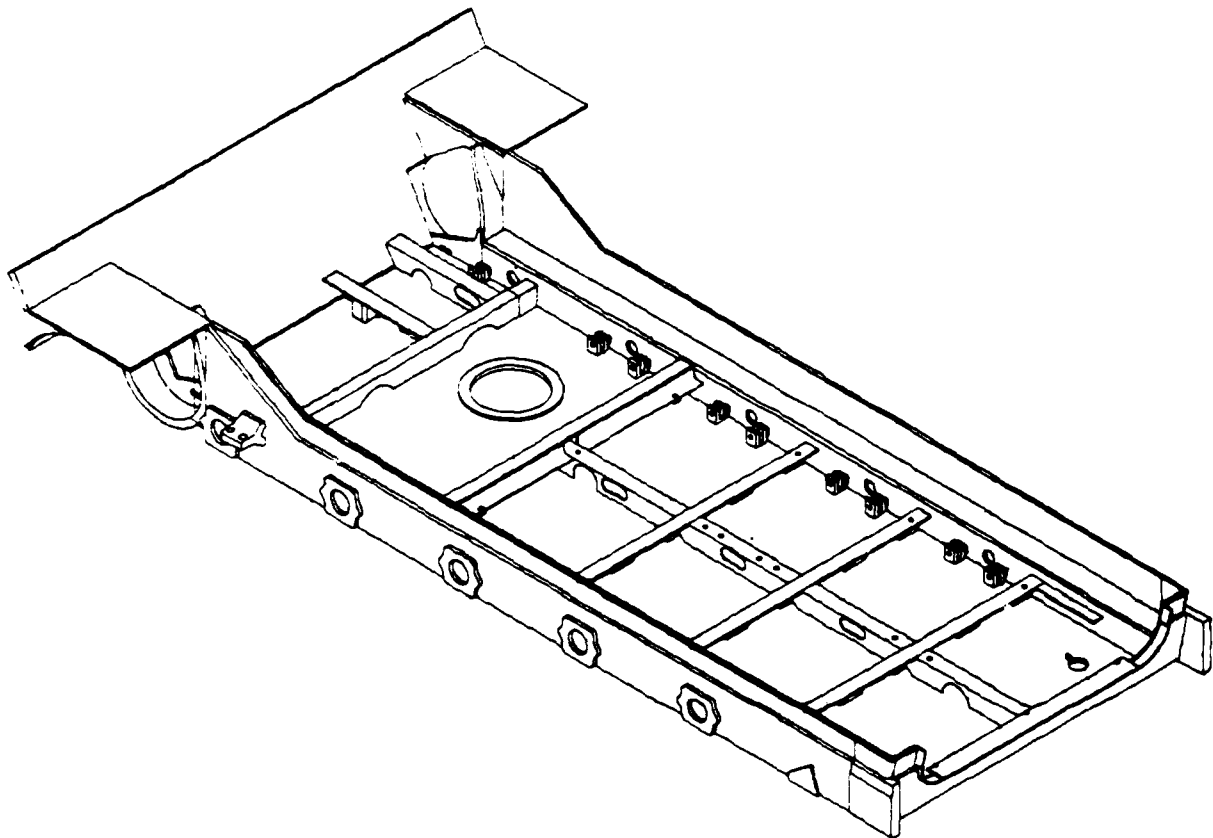
Figure 2-1. Hull Assembly
