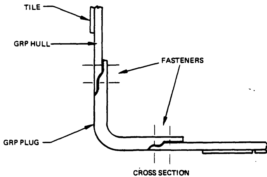
Figure 3-2. Field/Organizational and Depot Level Repair
