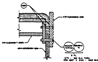
SECTION J-J SCALE 1/2
