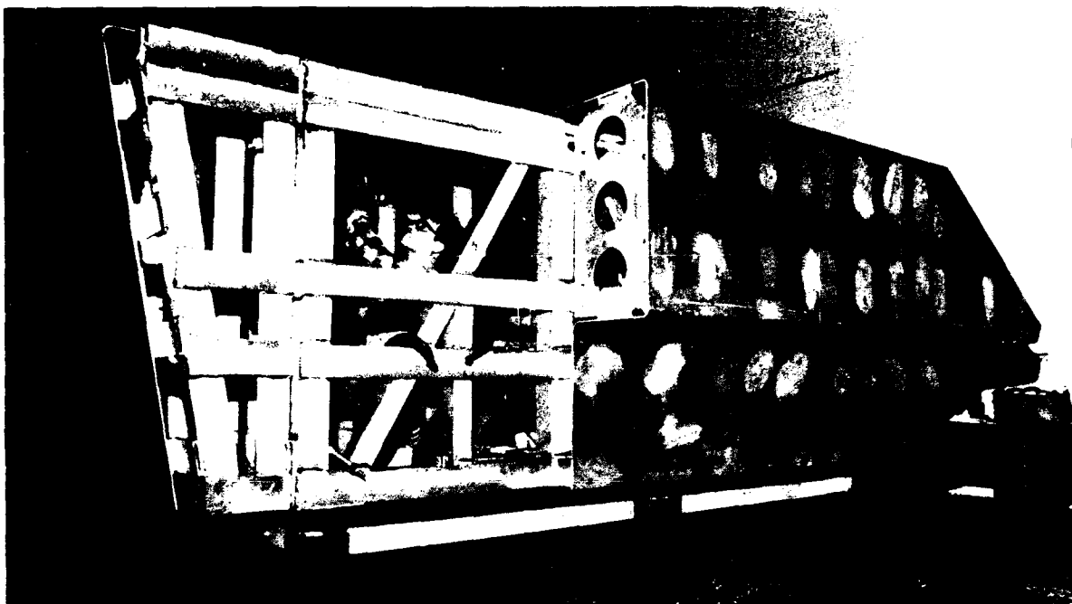
Figure 6-2. Upper Hull Layup Tool
