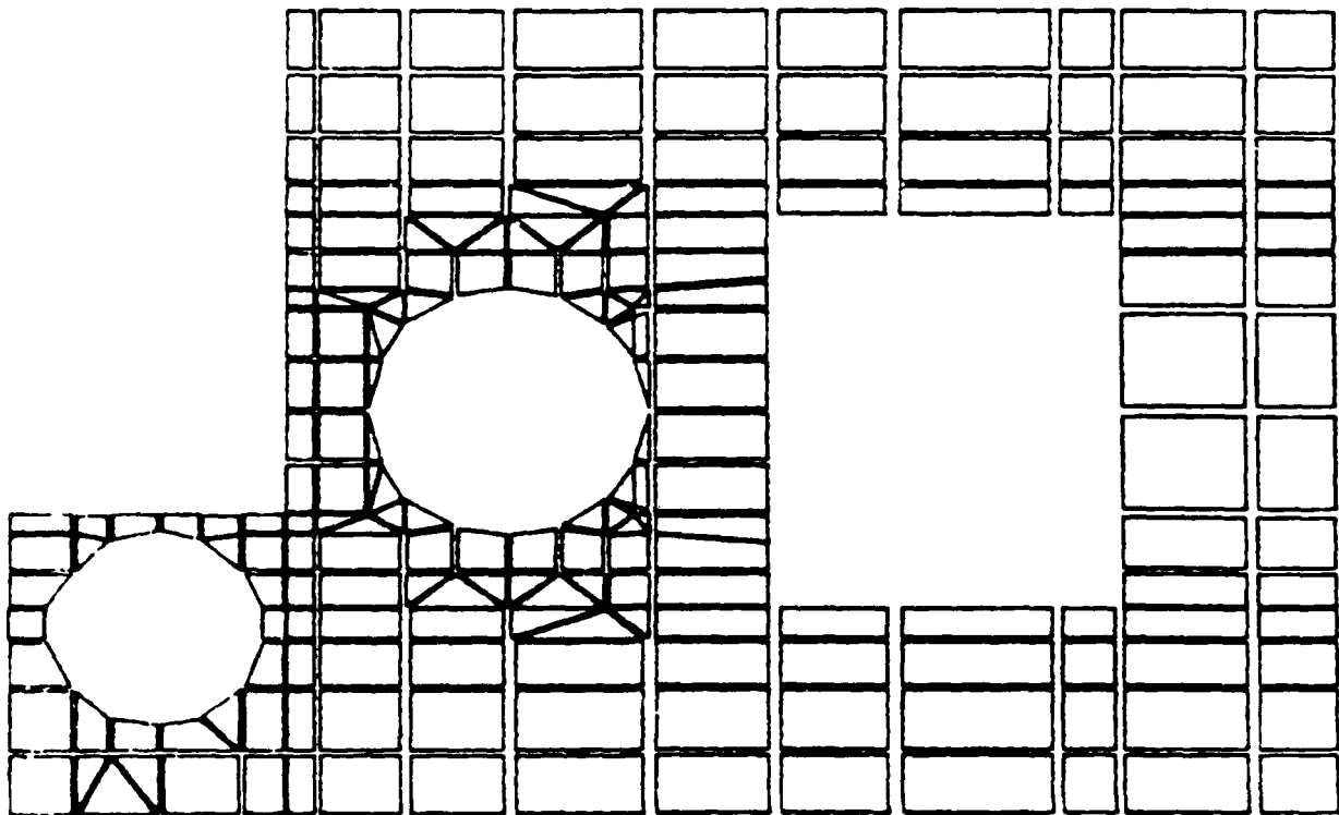
Figure 4-5. Top View of Finite Element Model
