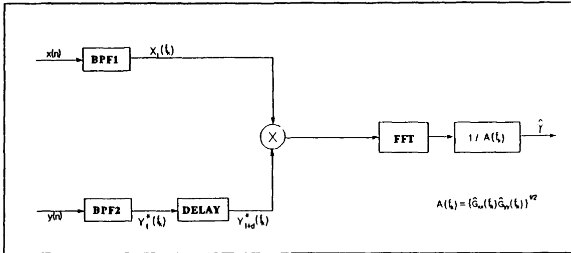
Figure 3. Coherence estimation block diagram using the FFT.
