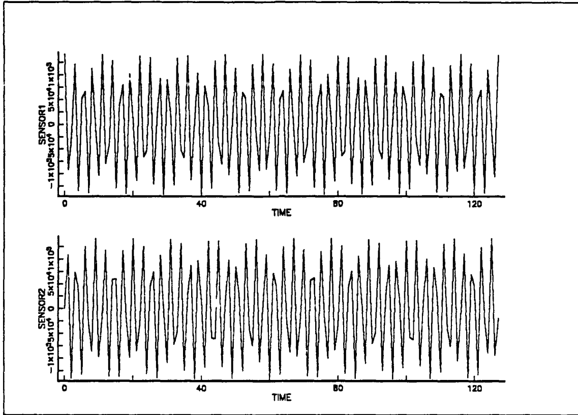
Figure 8. Two signals, 0 second delay at the sensors.
