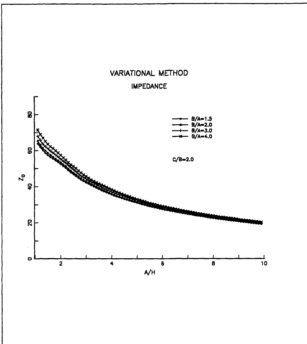
Figure 11. Calculated characteristic impedance of CBCPW by variational method: ( \epsilon_r = 3.52 , H = 1.5 mm)
