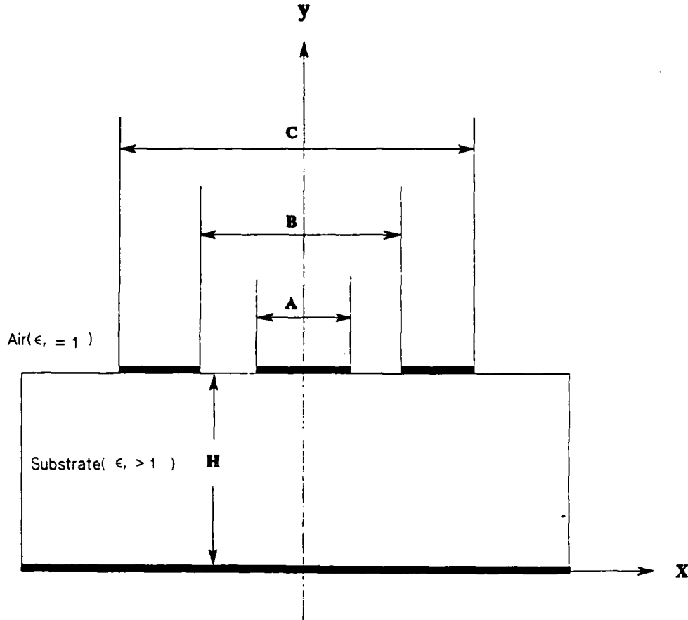
Figure 8. Geometry of CBCPW
