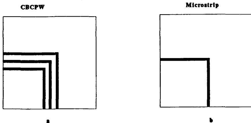
Figure 29. Line angle for conductor ambient field measurement
