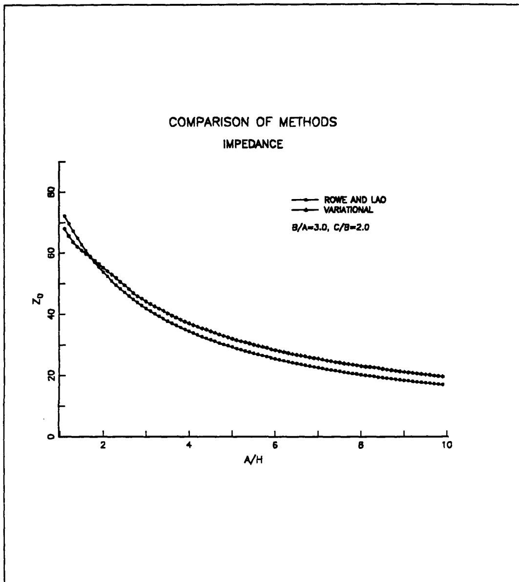
Figure 15. Computed results for characteristic impedance versus strip width with line dimensions as parameters: ( B/A = 3.0 , C/B = 2.0 , \epsilon_r = 3.52 , H = 1.5 mm )
