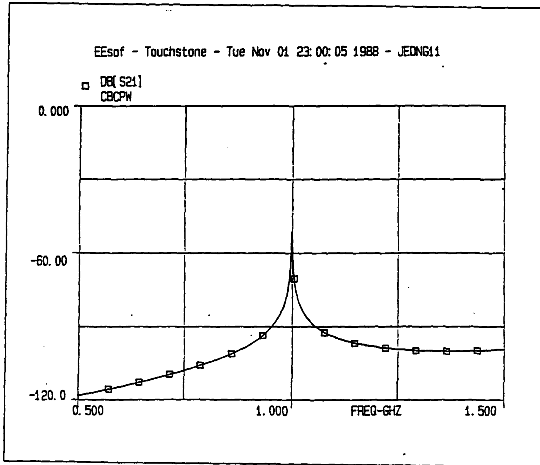
Figure 25. Plot for dB magnitude S_{21} versus frequency
