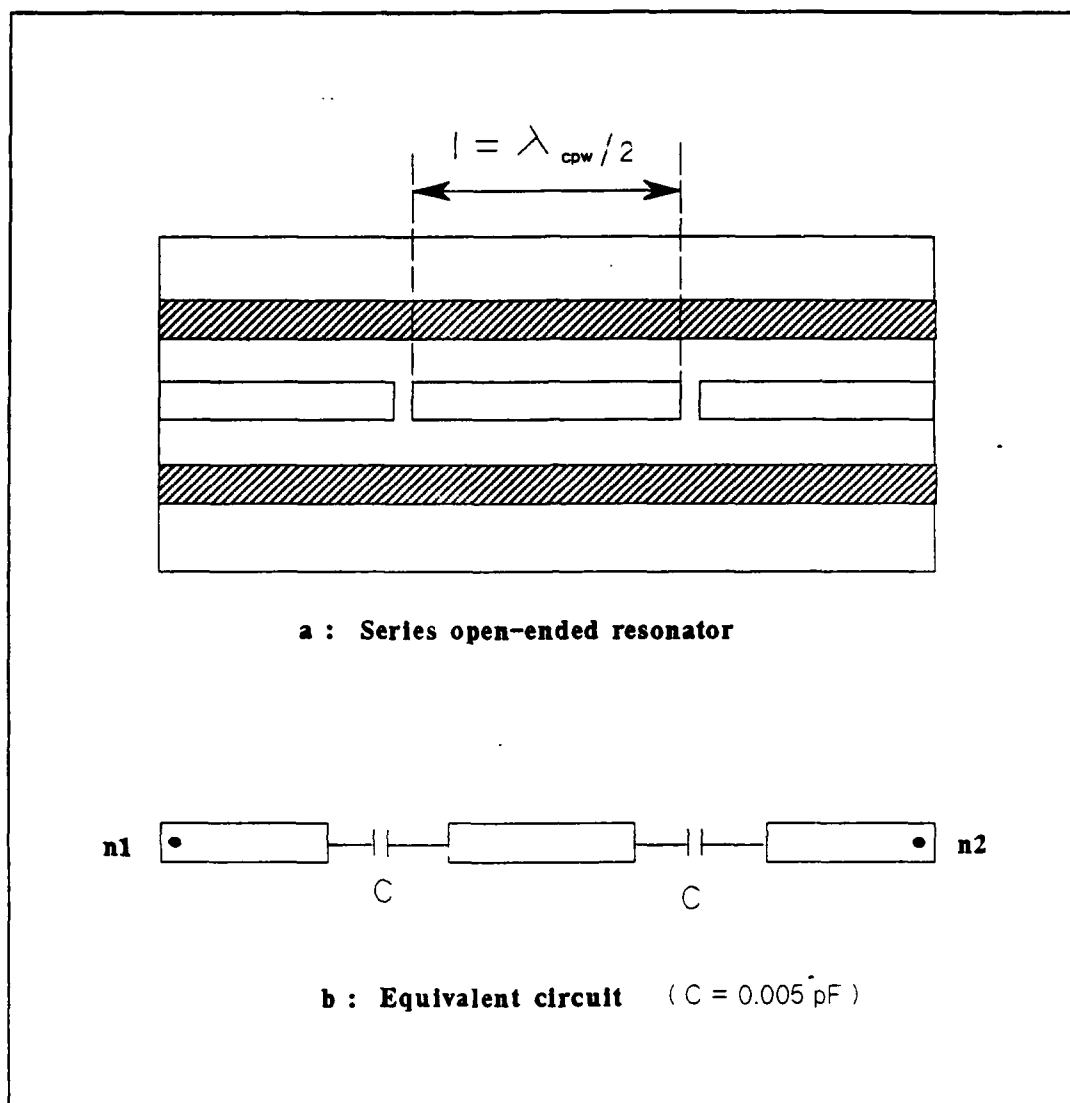
Figure 24. Series open-ended resonator and equivalent circuit
