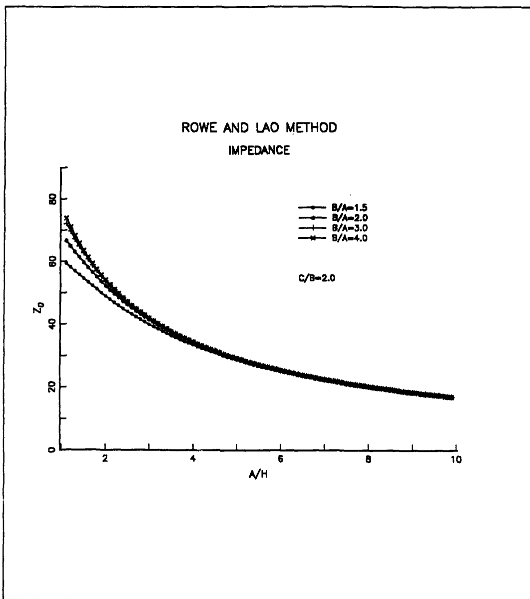
Figure 6. Calculated characteristic impedance of CBCPW by boundary point matching method: ( \epsilon_r = 3.52 , H = 1.5 mm)
