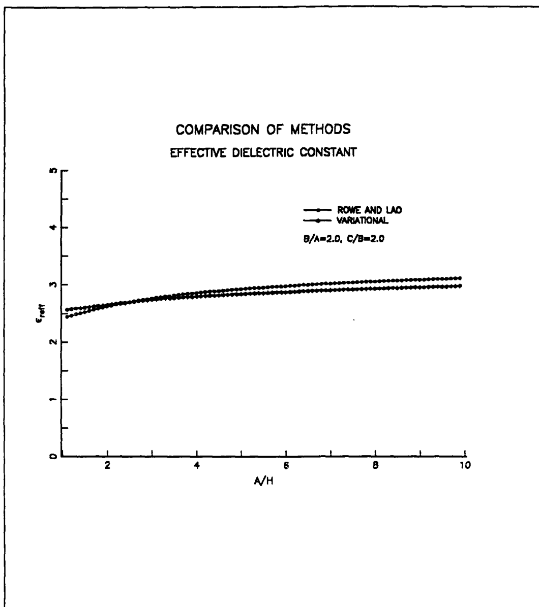
Figure 18. Computed results for dielectric constant versus strip width for various line parameters: ( B/A = 2.0 , C/B = 2.0 , \epsilon_r = 3.52 , H = 1.5 mm )
