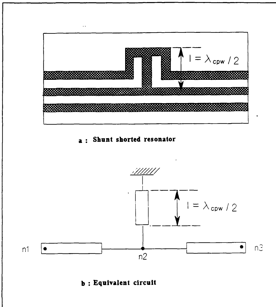
Figure 27. Shunt shorted resonator and equivalent circuit
