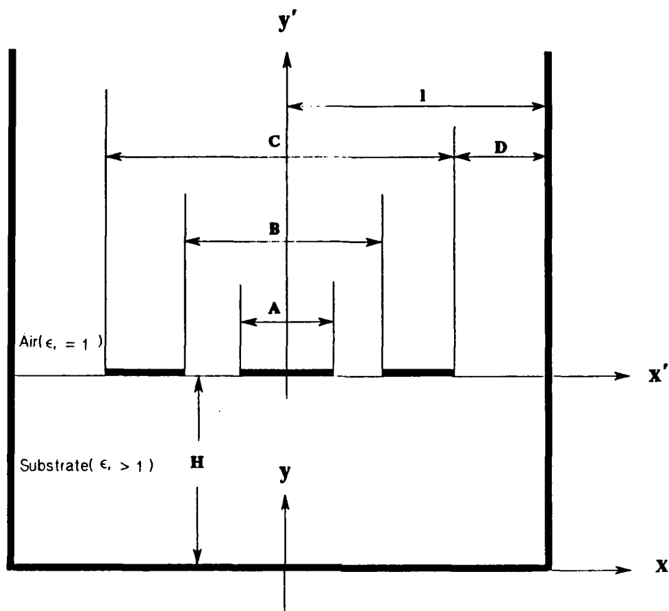
Figure 4. Geometry of a conductor backed CPW
