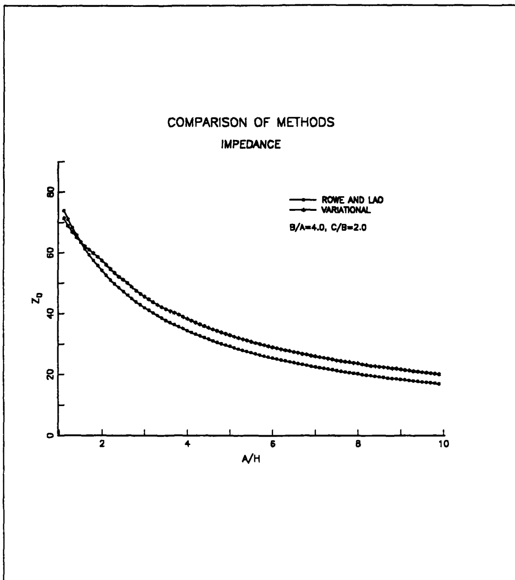
Figure 16. Computed results for characteristic impedance versus strip width with line dimensions as parameters: ( B/A=4.0 , C/B=2.0 , \epsilon_r = 3.52 , H = 1.5 mm )
