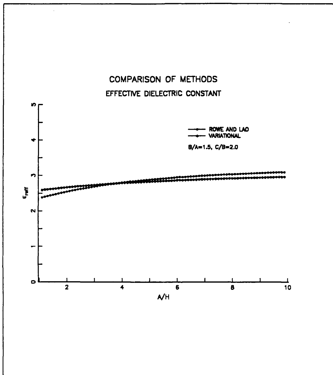
Figure 17. Computed results for dielectric constant versus strip width for various line parameters: ( B/A = 1.5 , C/B = 2.0 , \epsilon_r = 3.52 , H = 1.5 mm )
