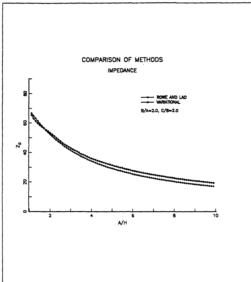
Figure 14. Computed results for characteristic impedance versus strip width with line dimensions as parameters: ( B/A=2.0 , C/B=2.0 , \epsilon_r = 3.52 , H = 1.5 mm )
