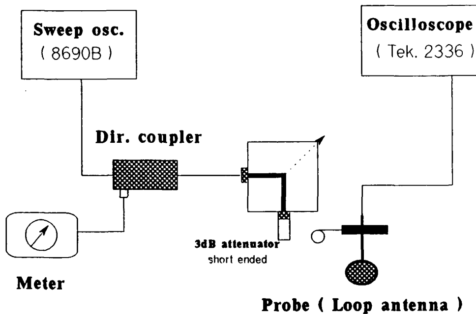
Figure 30. Block diagram for conductor ambient field measurement
