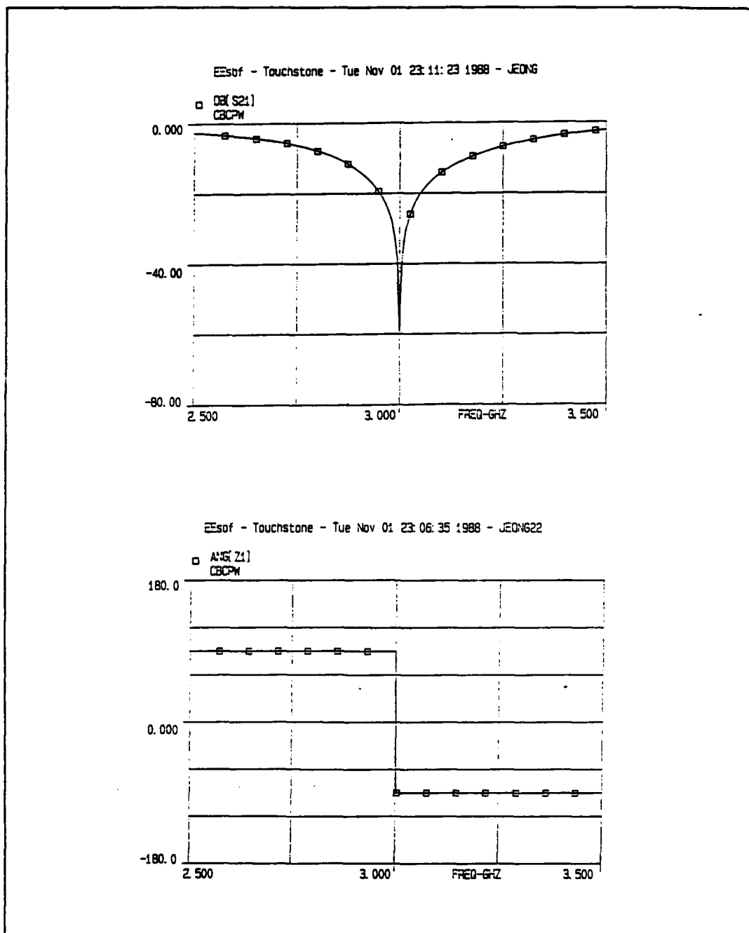
Figure 28. Plot for dB magnitude S_{21} with shunt shorted stub, and computed angle of impedance of \frac{\lambda}{4} open stub at resonance
