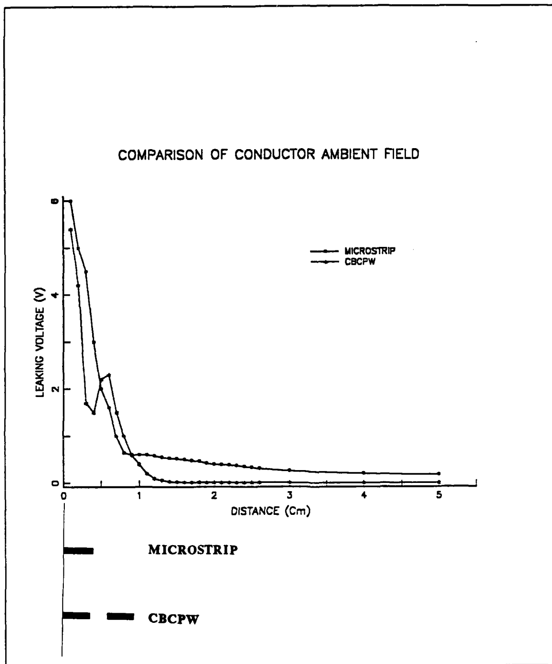
Figure 31. Conductor ambient field distribution
