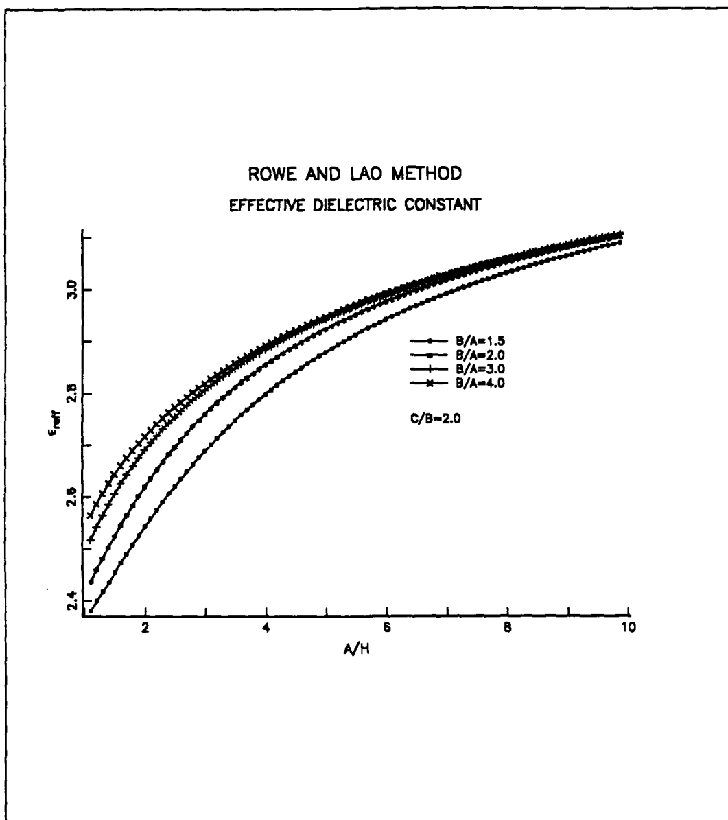
Figure 7. Calculated effective dielectric constant of CBCPW by boundary point matching method: ( \epsilon_r = 3.52 , H = 1.5 mm)
