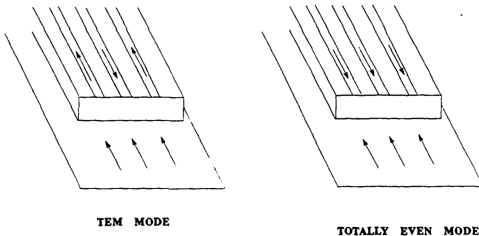
Figure 3. Current flow characteristics of propagation modes
