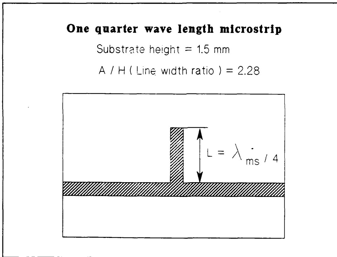
Figure 21. Quarter wave length stub for substrate dielectric constant measurement
