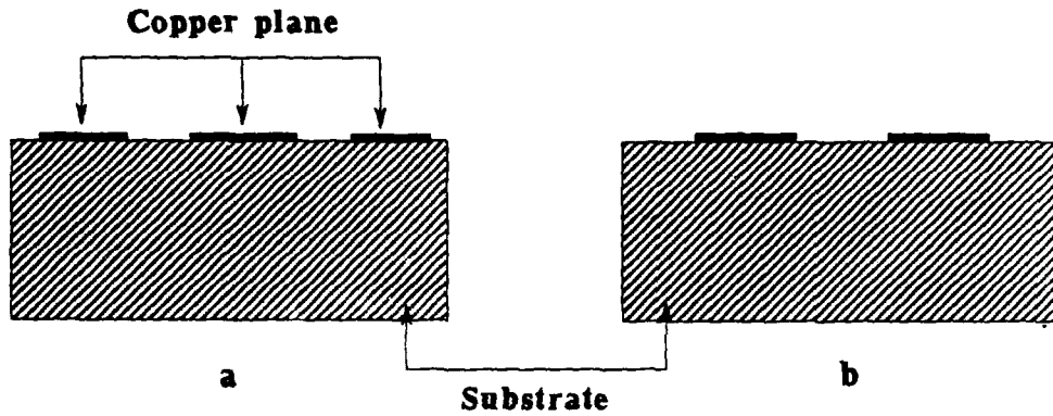
Figure 1. Coplanar systems
