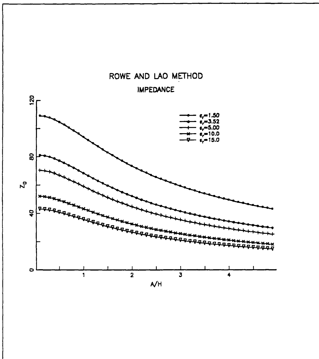
Figure 32. Characteristic impedance versus strip width with dielectric constant as a parameter: ( B/A = 2.0 , C/B = 2.0 , H = 1.5 mm )
