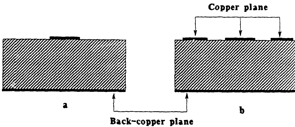
Figure 2. Conductor backed planar waveguides
