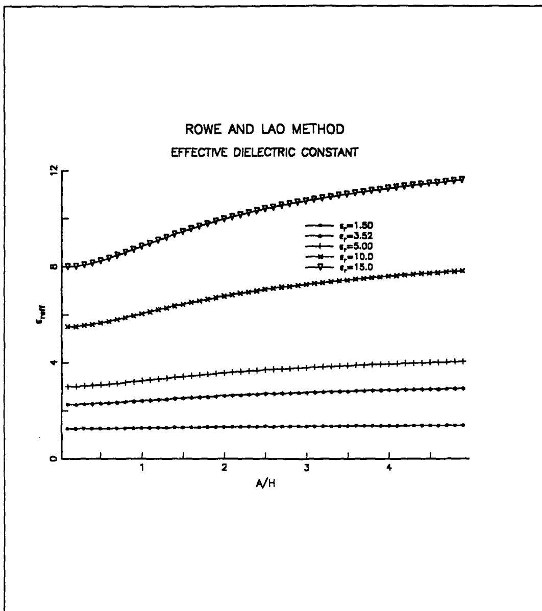
Figure 33. Effective dielectric constant versus strip width with substrate dielectric constant as a parameter: ( B/A = 2.0 , C/B = 2.0 , H = 1.5 mm )
