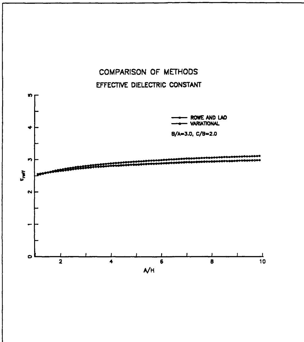
Figure 19. Computed results for dielectric constant versus strip width for various line parameters: ( B/A = 3.0 , C/B = 2.0 , \epsilon_r = 3.52 , H = 1.5 mm )
