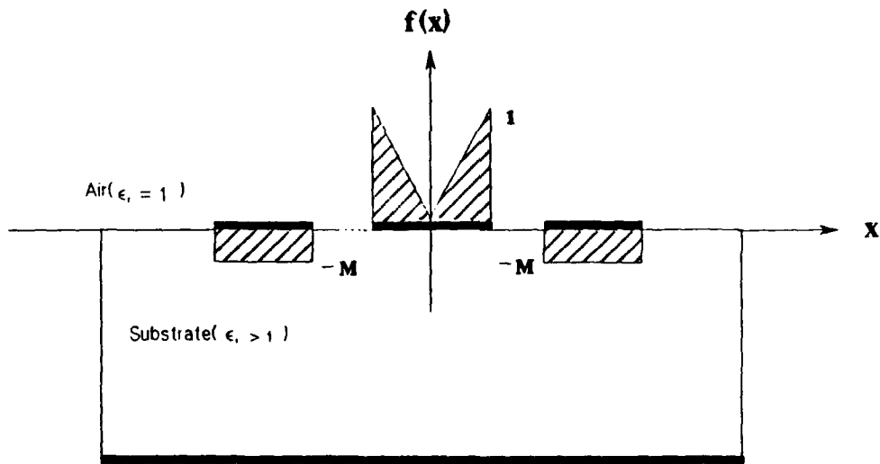
Figure 10. Assumed linear-charge density function of CBCPW: ( f(x) = |x| )
