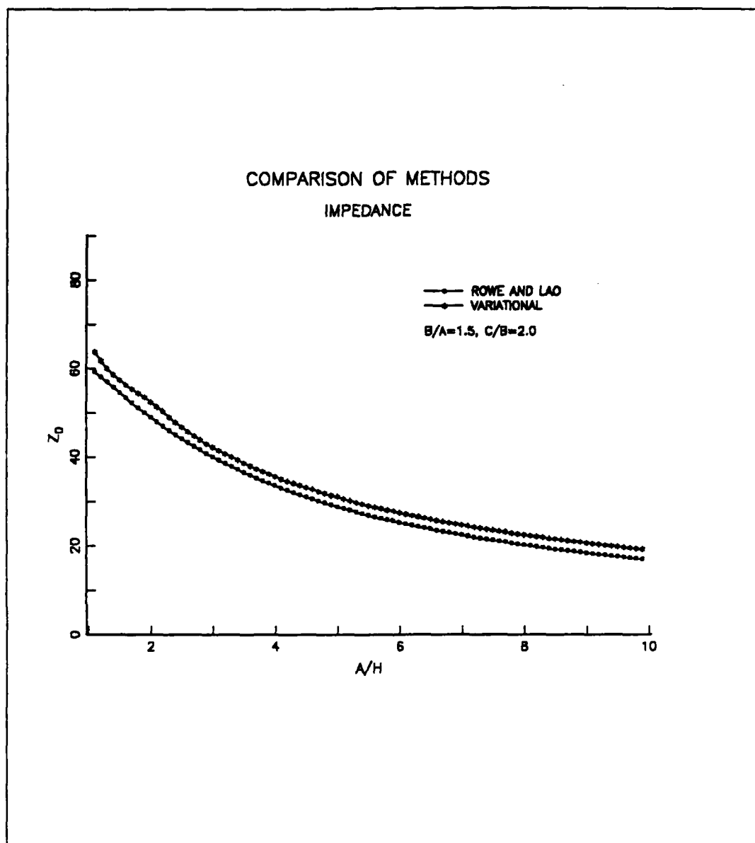
Figure 13. Computed results for characteristic impedance versus strip width with line dimensions as parameters: ( B/A = 1.5 , C/B = 2.0 , \epsilon_r = 3.52 , H = 1.5 mm )
