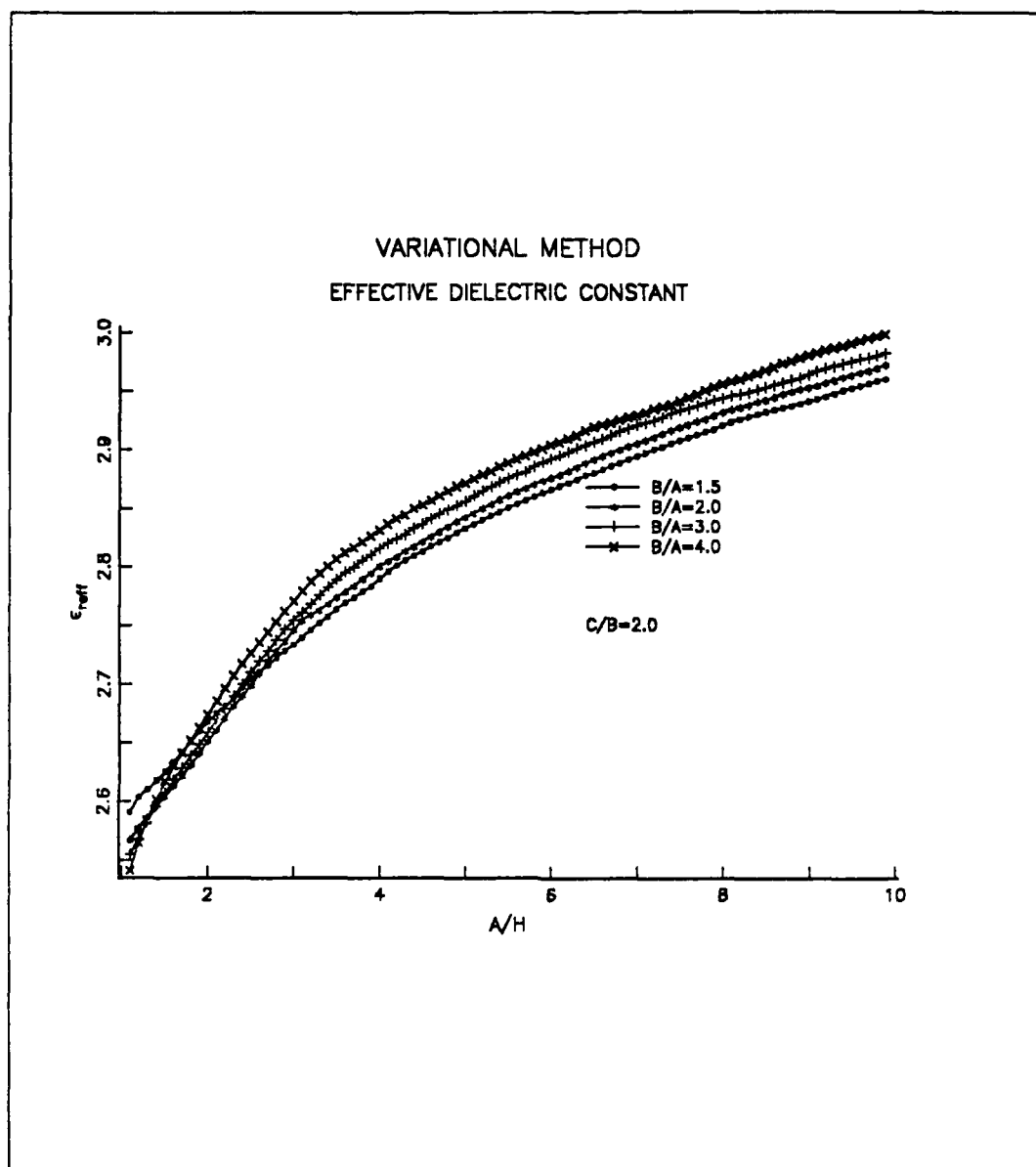
Figure 12. Calculated effective dielectric constant of CBCPW by variational method: ( \epsilon_r = 3.52 , H = 1.5 mm)
