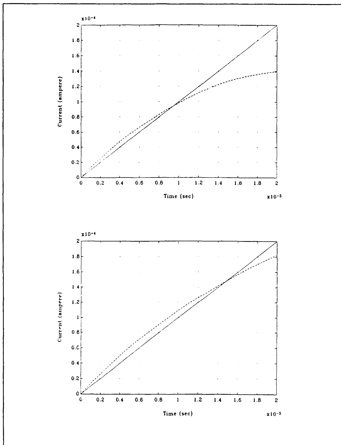
Fig. 4.1 DC transfer characteristic of input replicator.
