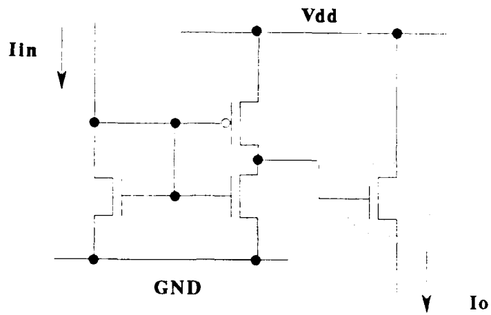
a) Step-down function generator
