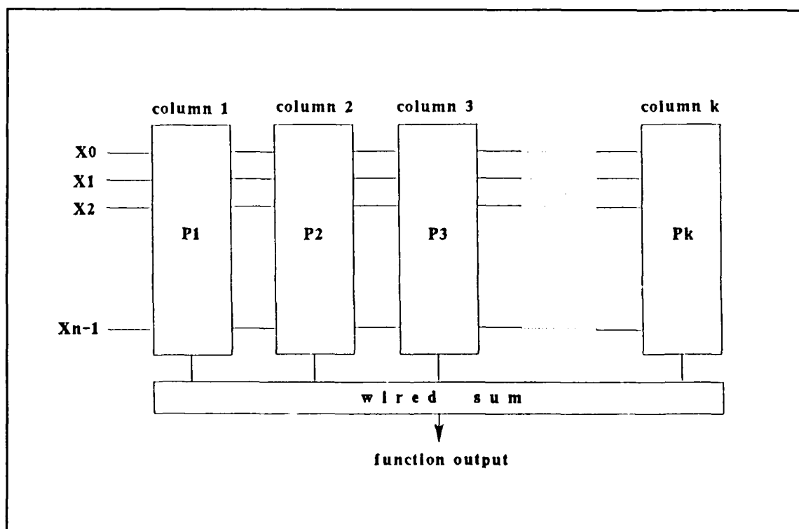
Fig. 5.1 Top level design of PLA
