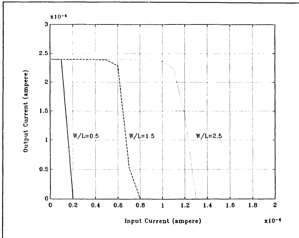
Fig. 4.3 DC transfer characteristic of step-down function generator
