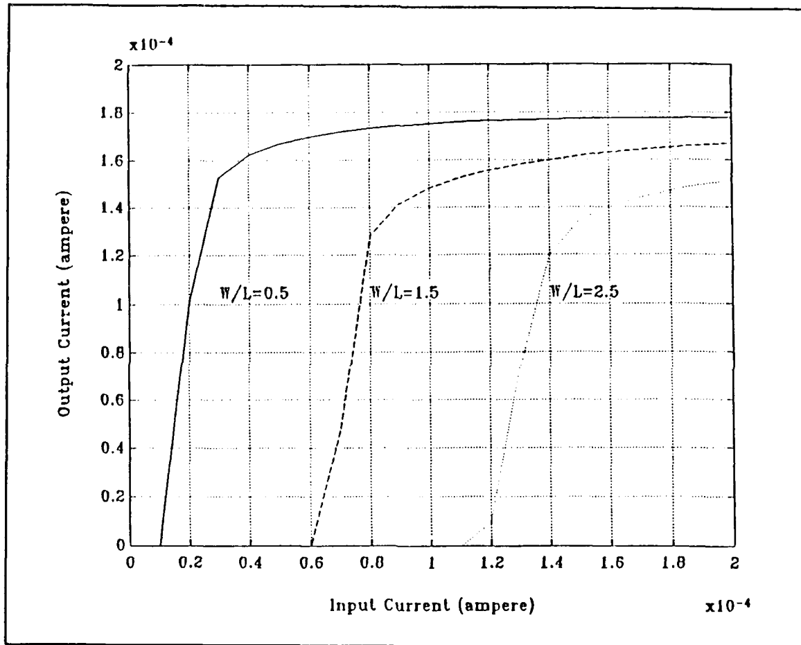
Fig. 4.2 DC transfer characteristic of step-up function generator
