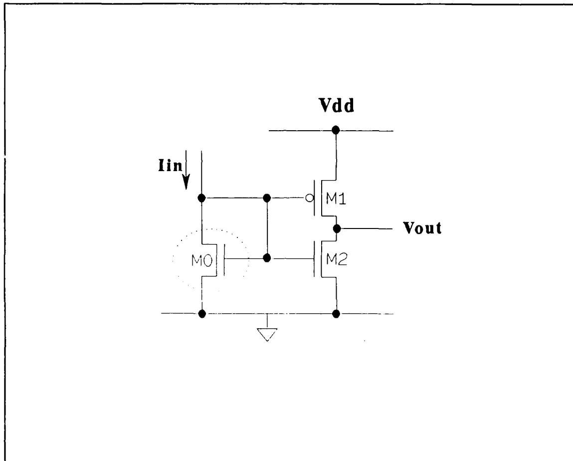
Fig. 2.1 CMOS inverter with the current input
