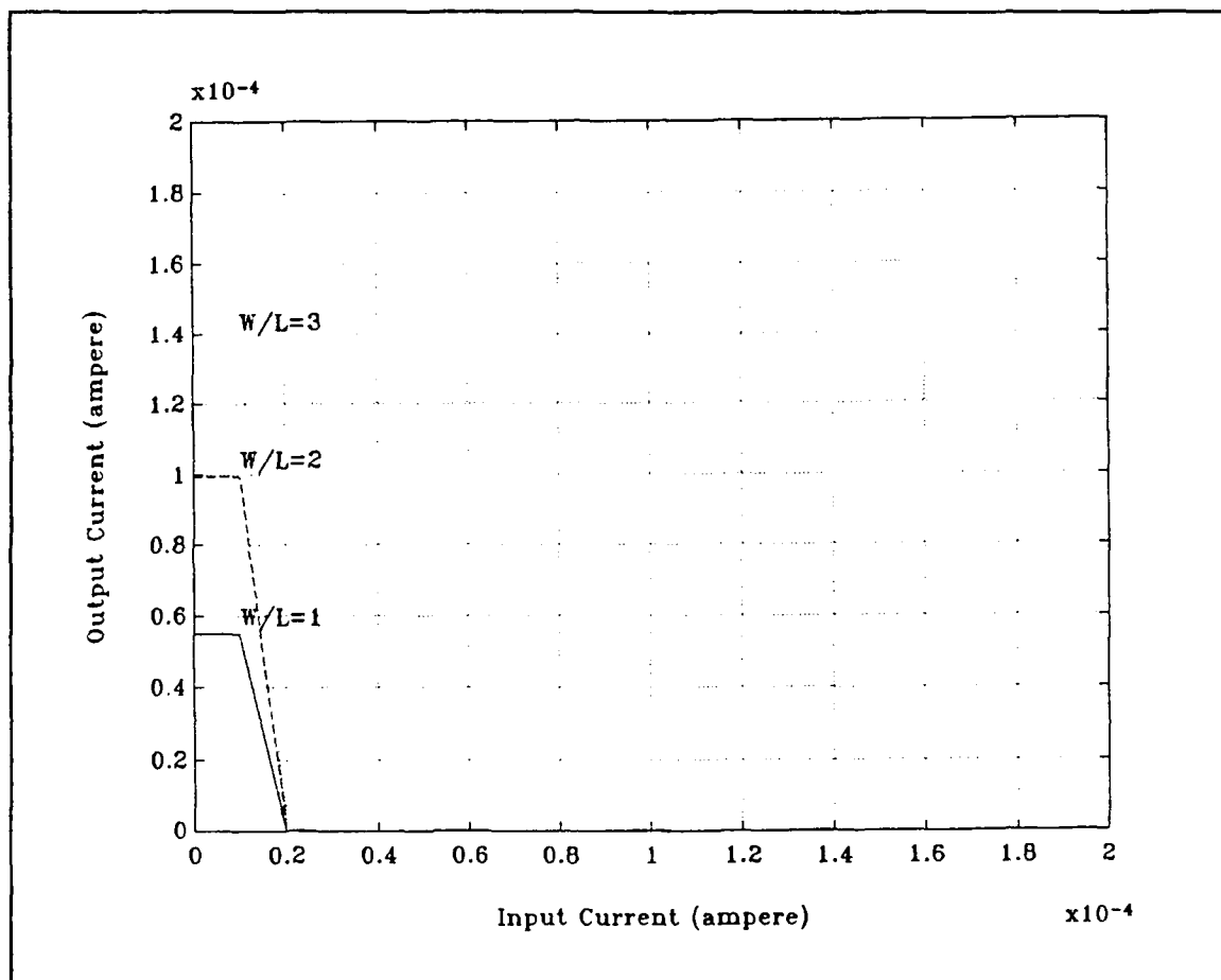
Fig. 4.4 DC transfer characteristic of column output generator
