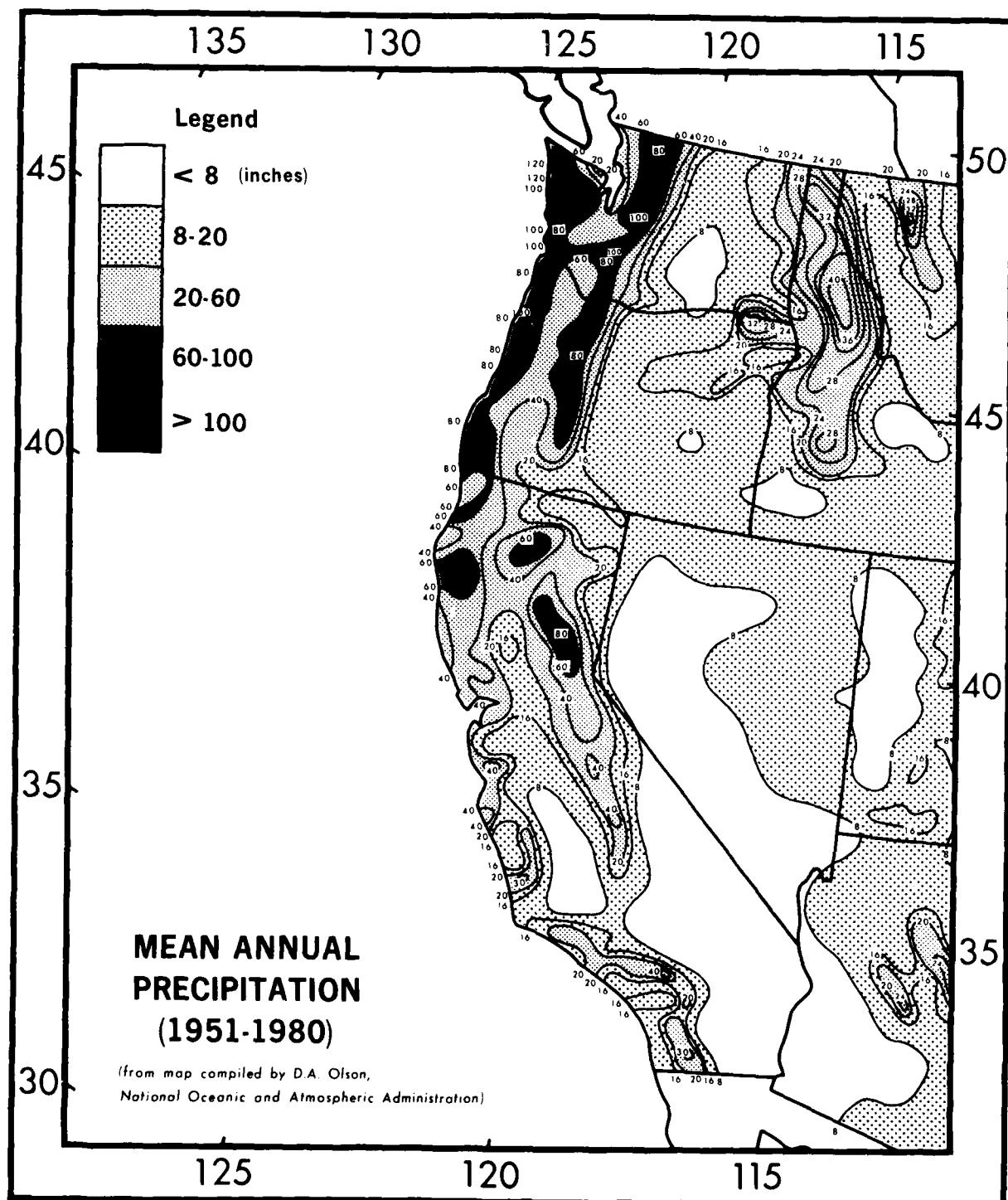
FIGURE 5. MEAN ANNUAL PRECIPITATION
