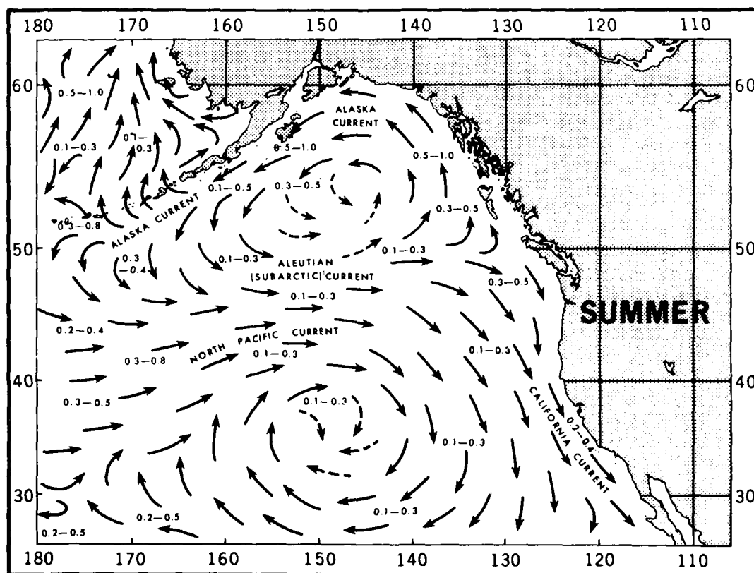
FIGURE 3. SURFACE CURRENTS (SUMMER AND WINTER)
