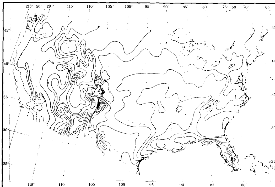
FIGURE 6. MEAN NUMBER OF ANNUAL THUNDERSTORMS
