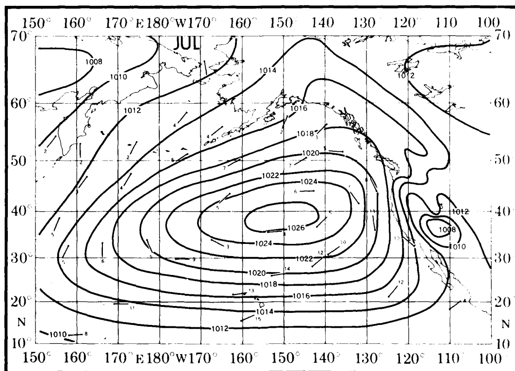
FIGURE 4. JANUARY AND JULY MEAN SEA-LEVEL PRESSURE AND VECTOR MEAN WINDS
