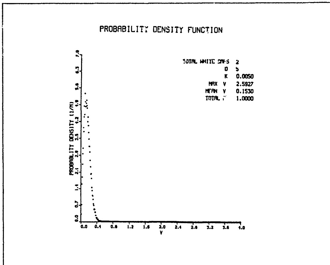
Figure 52. Simulated PDF of chatter voltage from whitecaps only, Randomness factor = 0.005, internal decorrelation time = 5.
