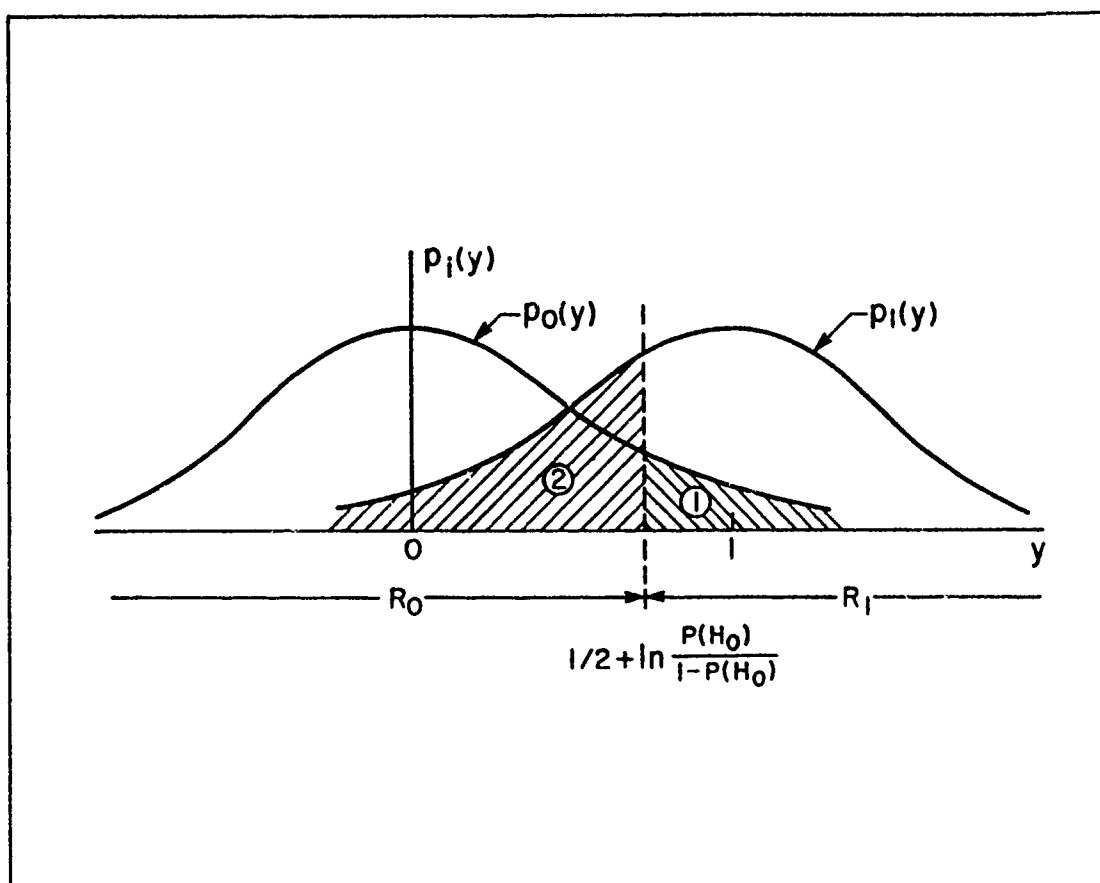
Figure 1. Decision Diagram in Gaussian Noise.
