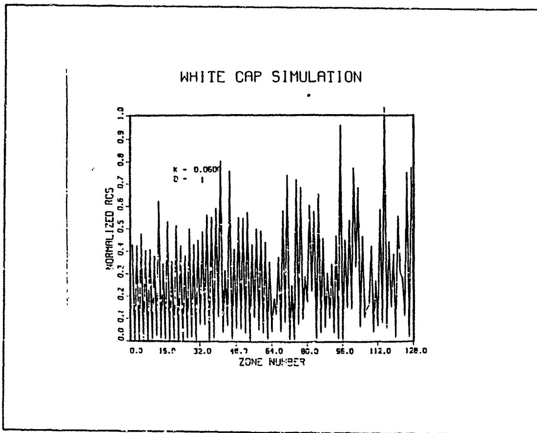
Figure 8. Simulated scattered signal from whitecap, D = 1 , k = 0.06 .
